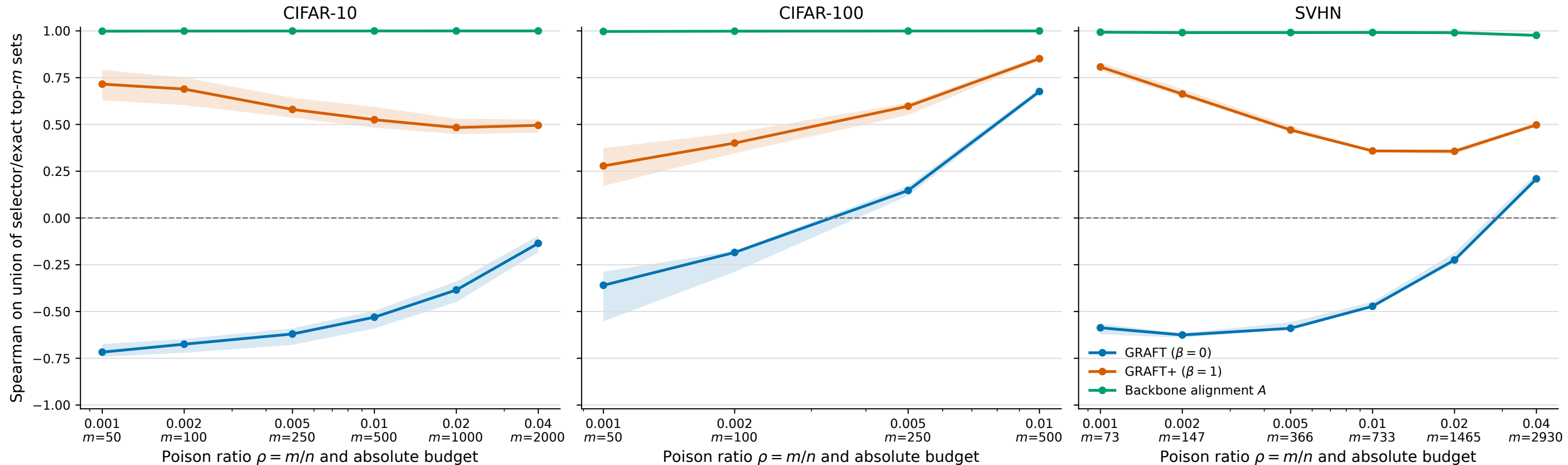
Budget-local rank agreement with exact gradient alignment Lines are target medians; bands are target IQRs
