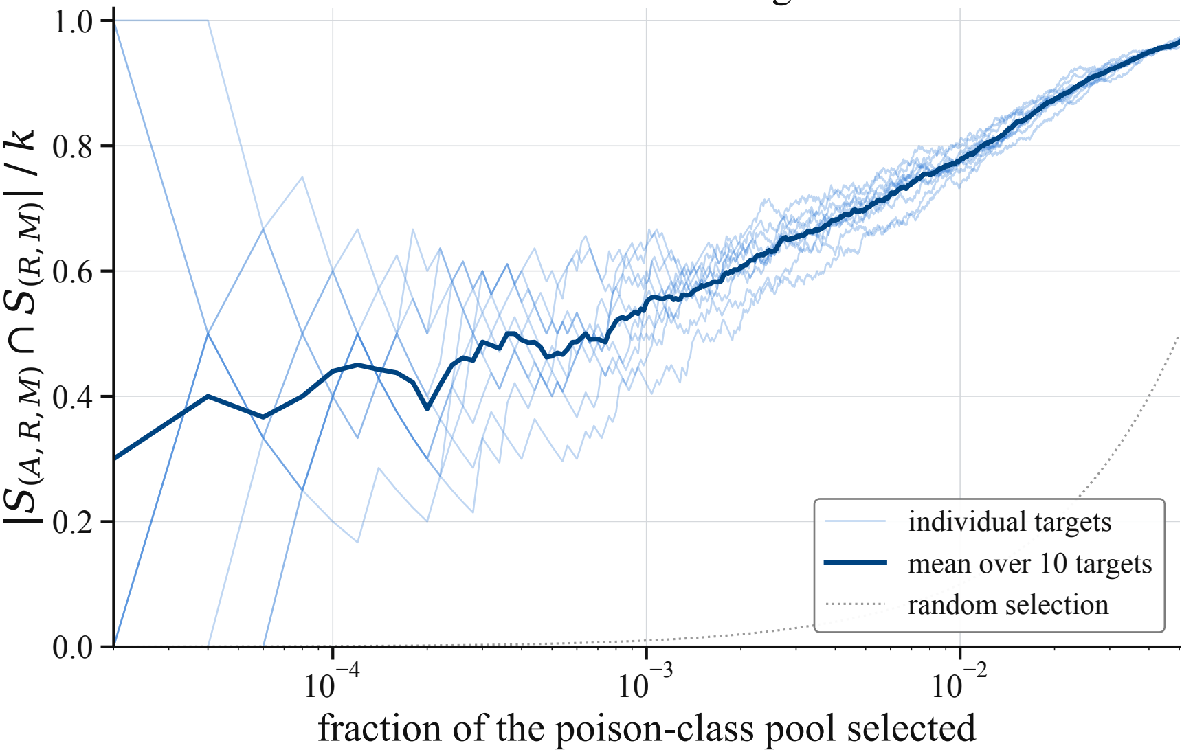
ResNet20BN / fc / dog-bird
