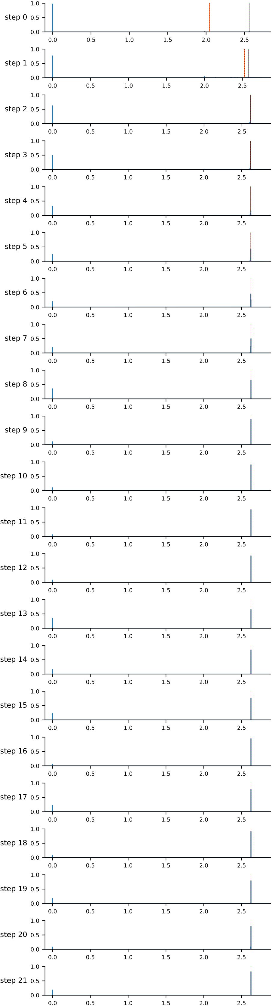
reward
