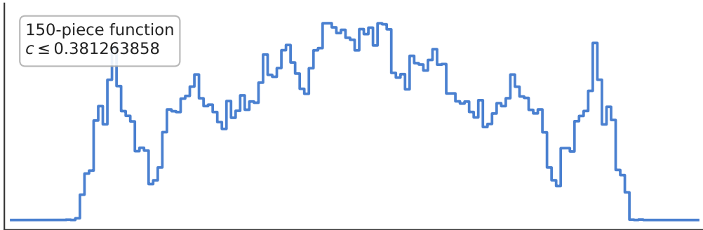
Erdos h (step 11 group 1 rollout 4)
