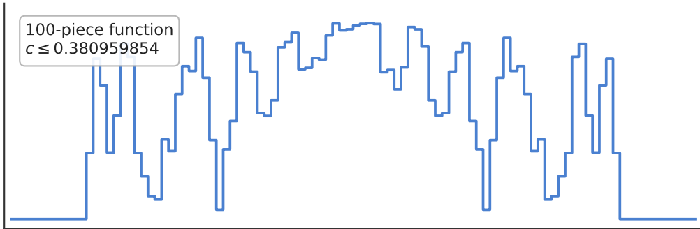
Erdos h (step 19 group 7 rollout 38)
