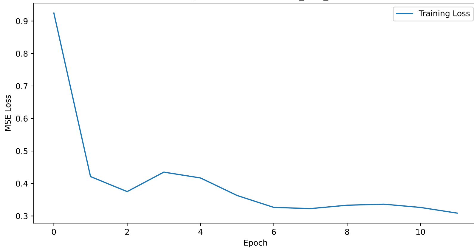
Training Loss Curve for dallas_12H_nhits
