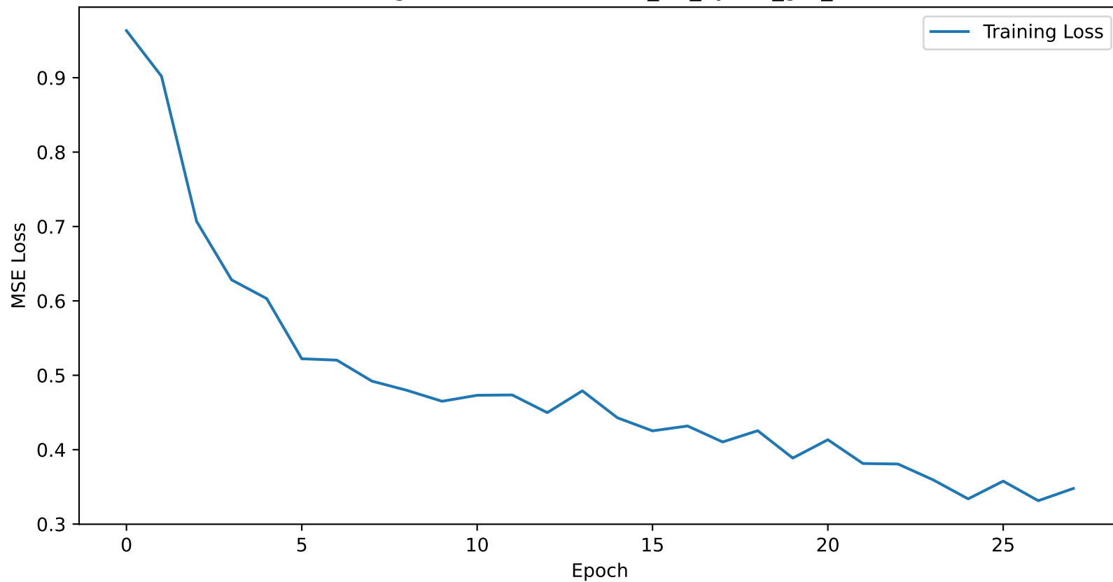
Training Loss Curve for dallas_2H_hybrid_gru_lstm
