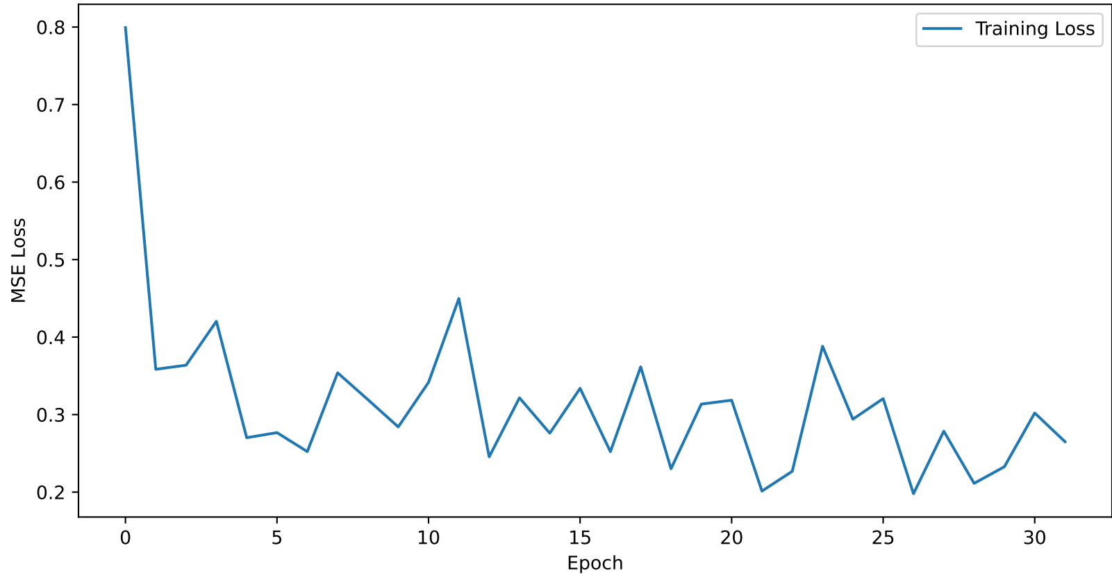
Training Loss Curve for dallas_6H_nhits
