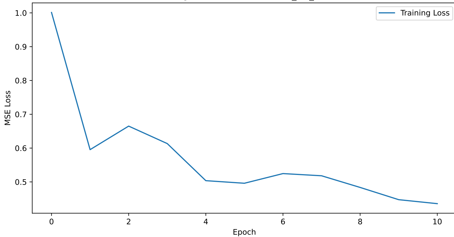
Training Loss Curve for atlanta_1D_nhits
