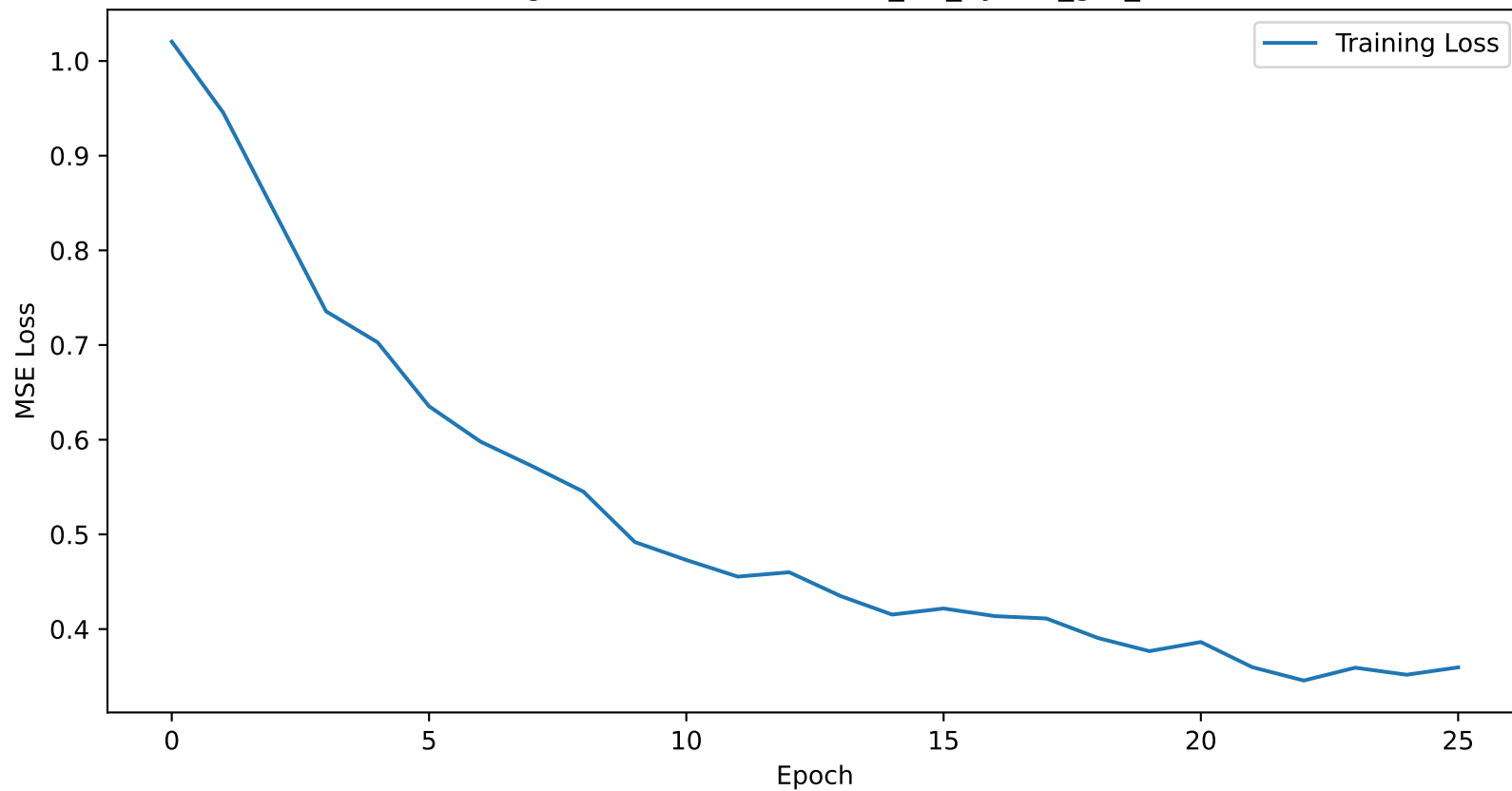
Training Loss Curve for atlanta_1H_hybrid_gru_lstm
