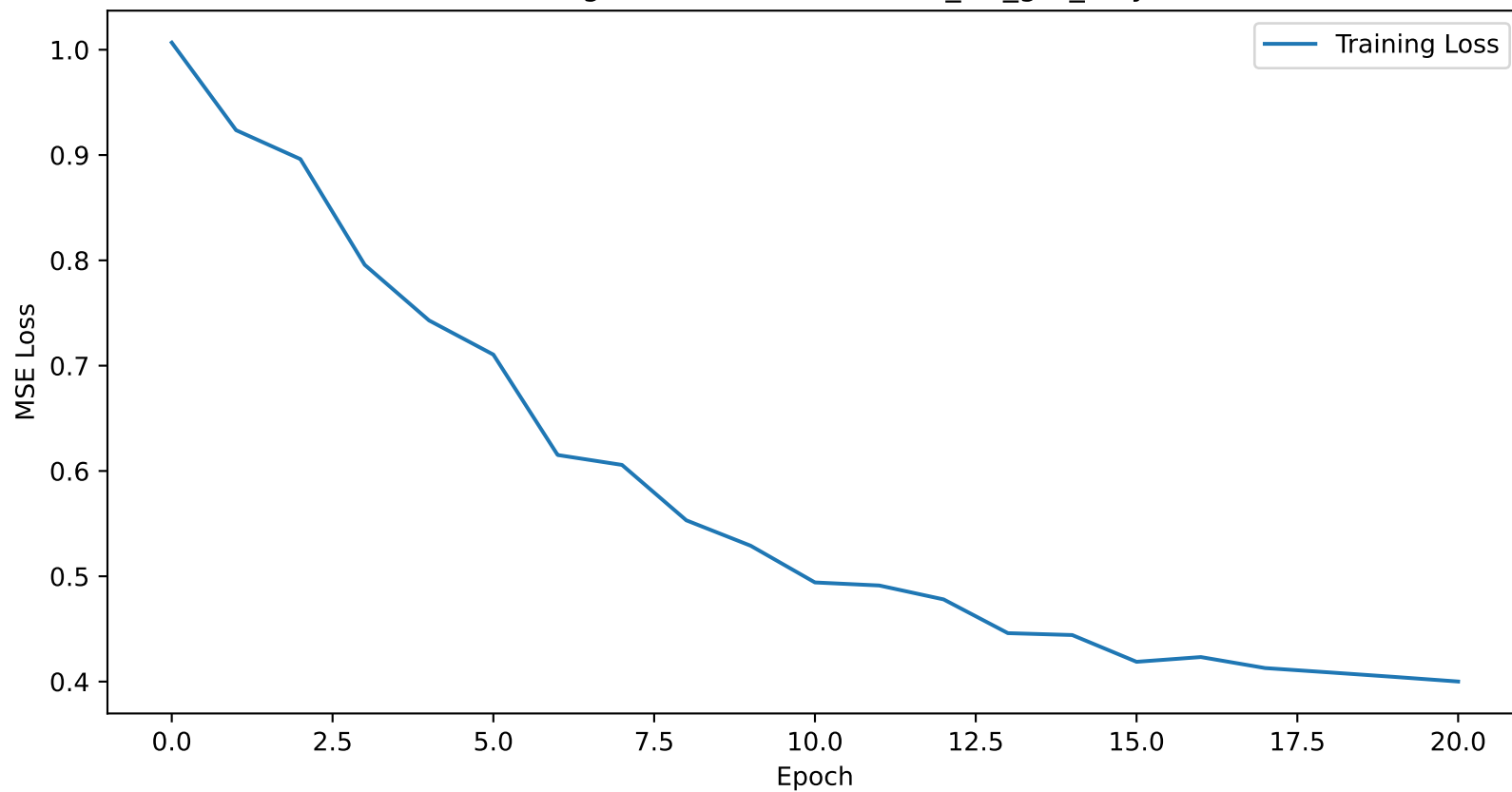
Training Loss Curve for atlanta_1H_gru_only
