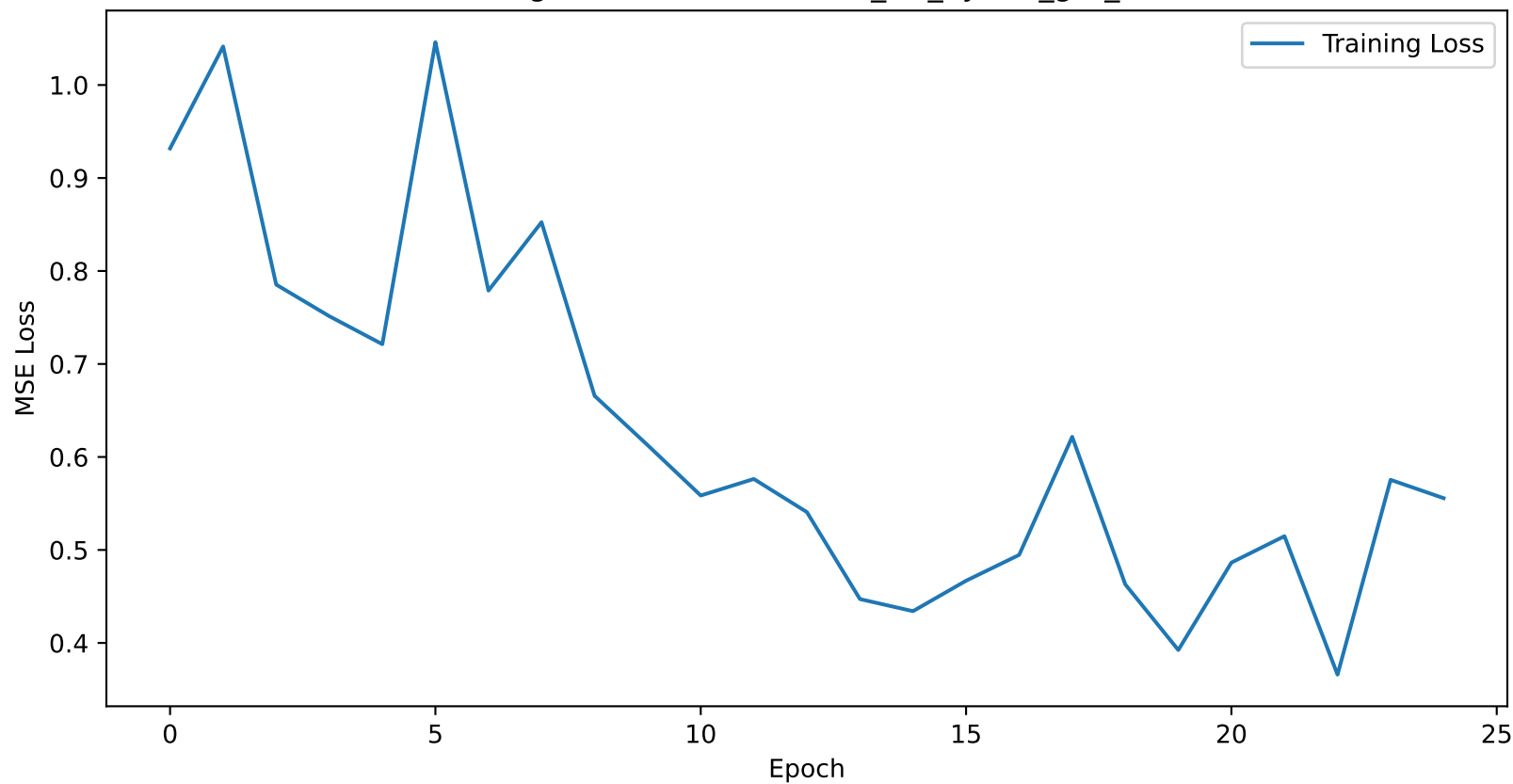
Training Loss Curve for dallas_6H_hybrid_gru_lstm
