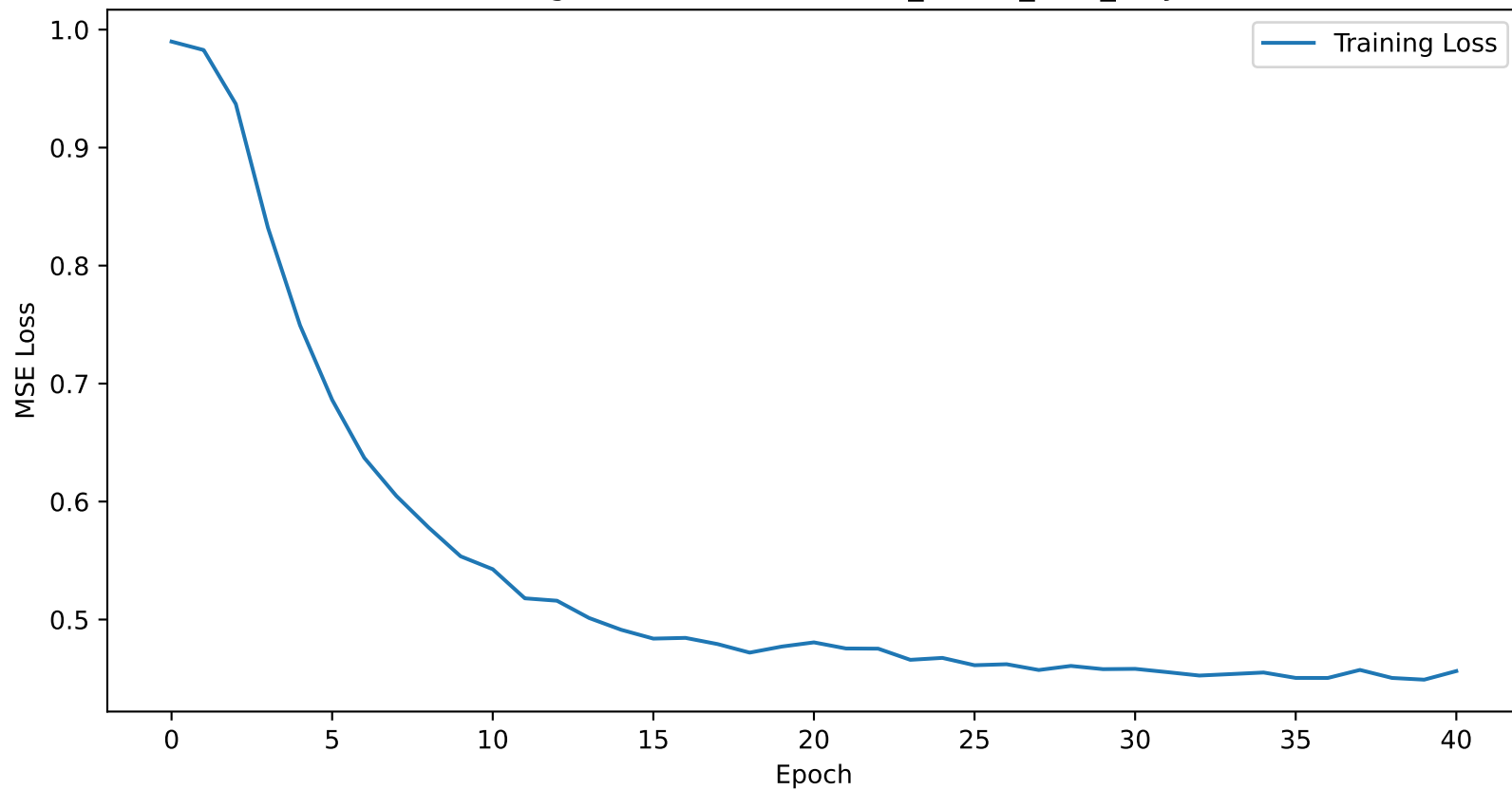
Training Loss Curve for boston_30min_lstm_only
