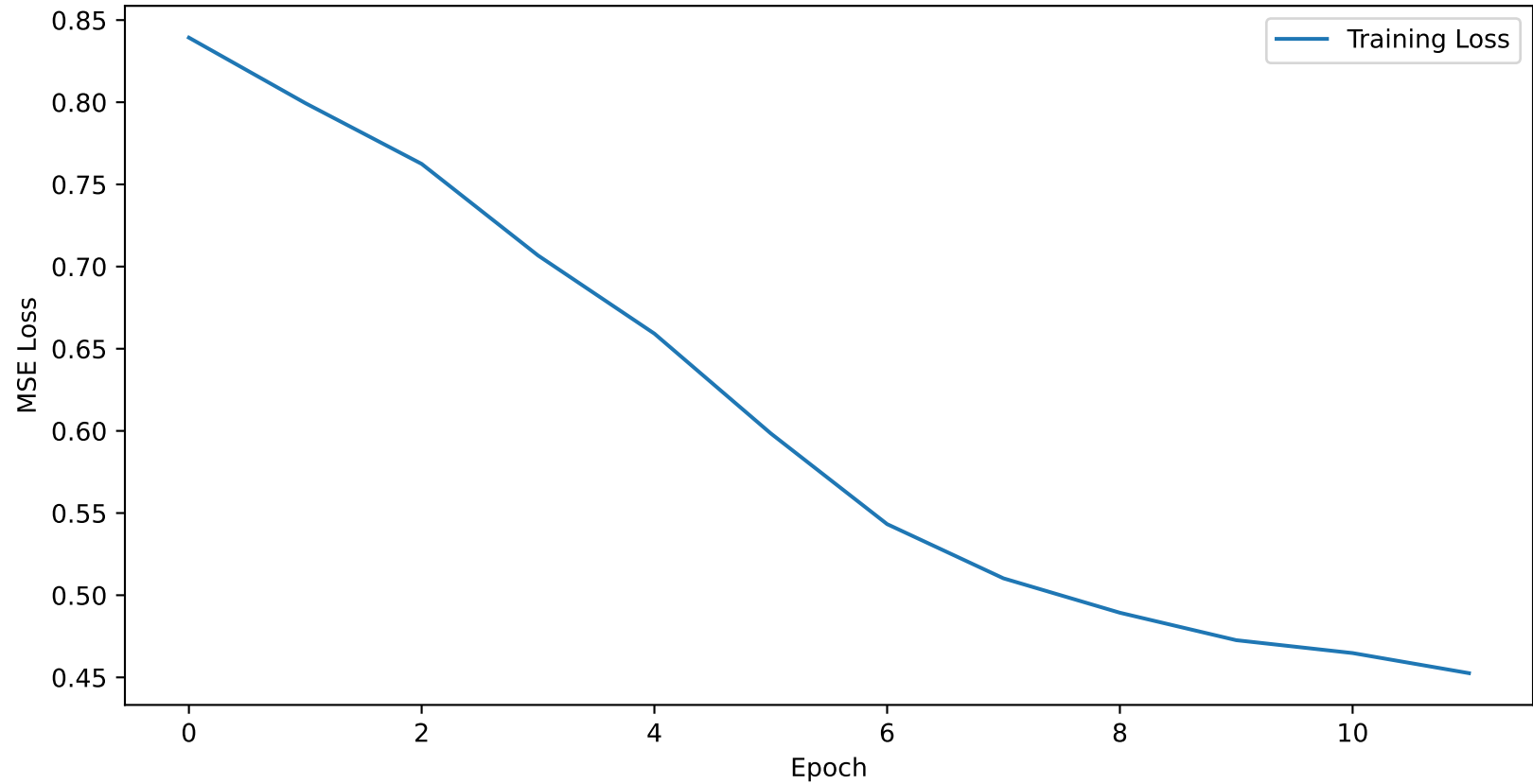
Training Loss Curve for elpaso_5min_gru_only
