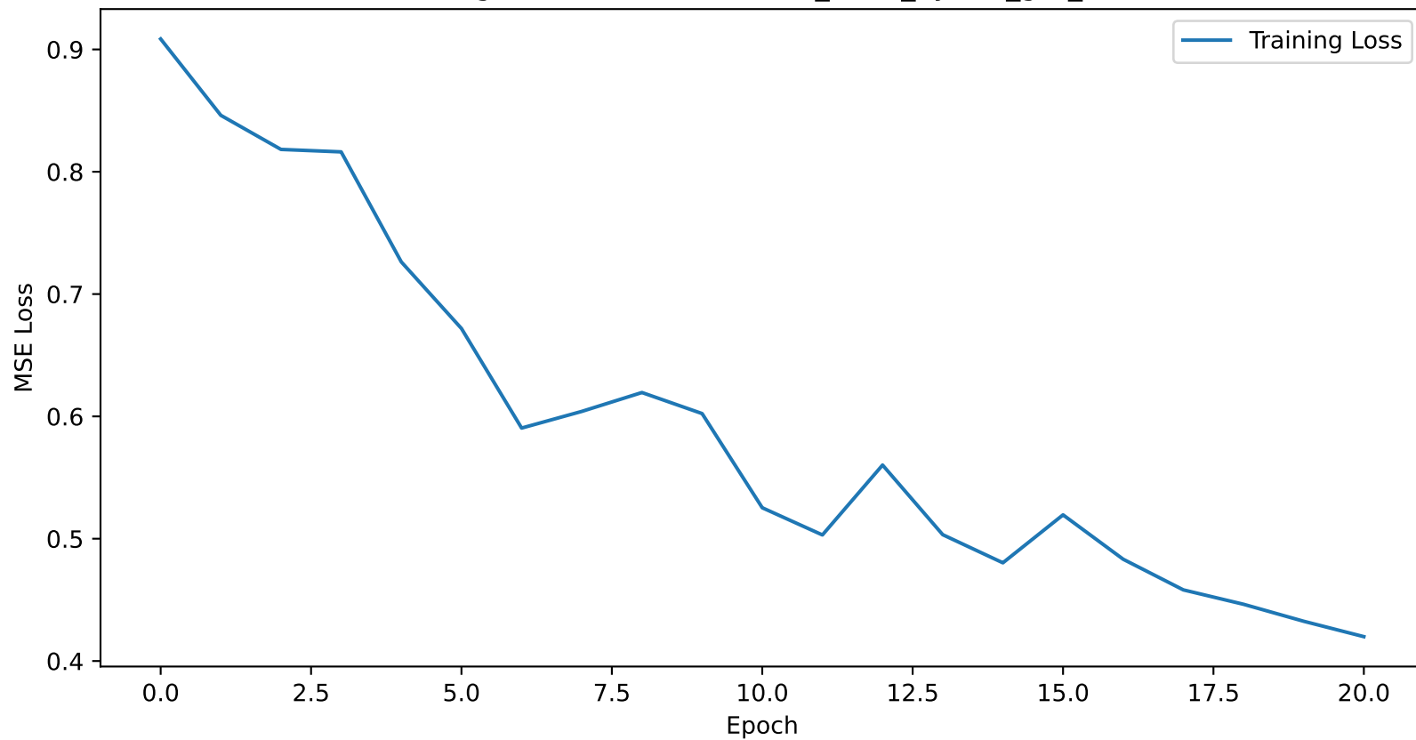
Training Loss Curve for atlanta_5min_hybrid_gru_lstm
