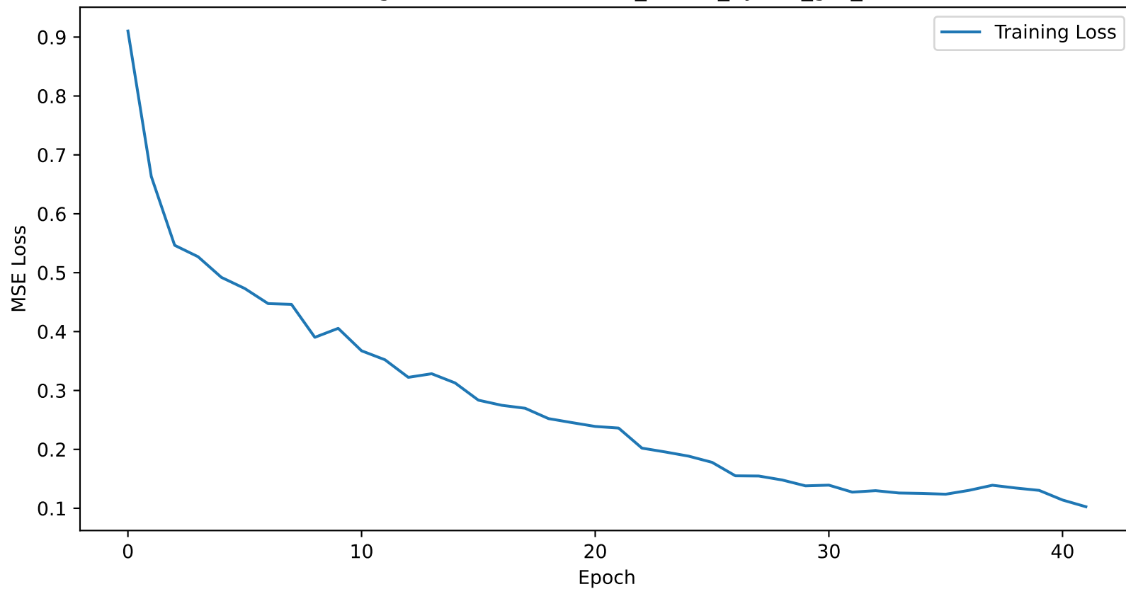
Training Loss Curve for dallas_45min_hybrid_gru_lstm
