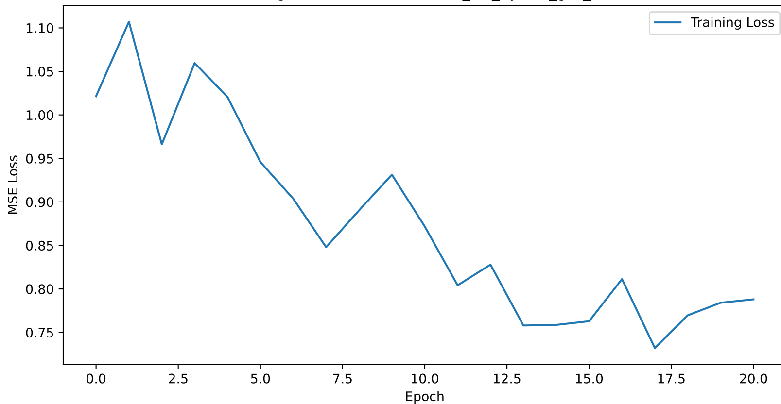
Training Loss Curve for atlanta_6H_hybrid_gru_lstm
