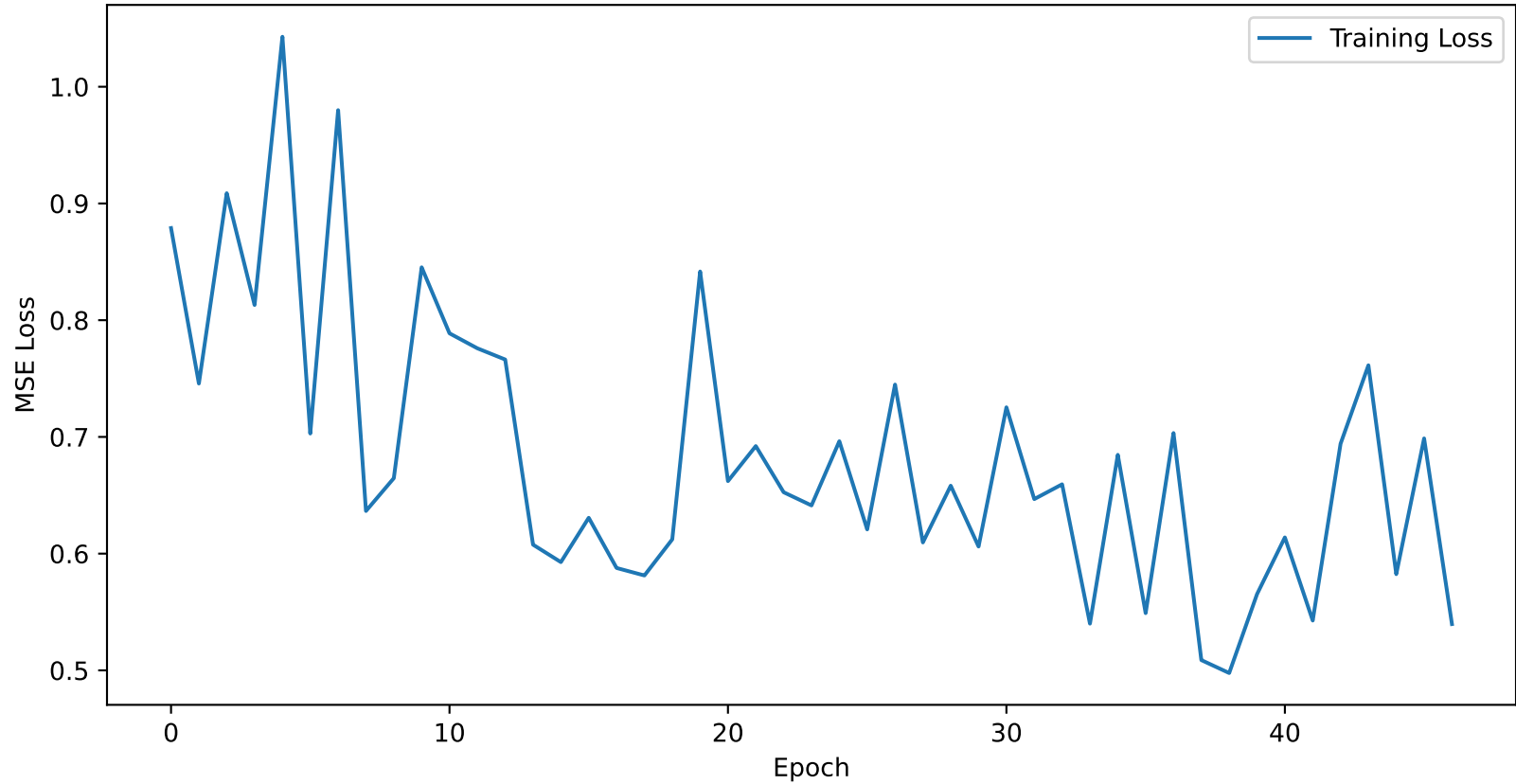
Training Loss Curve for elpaso_6H_lstm_only
