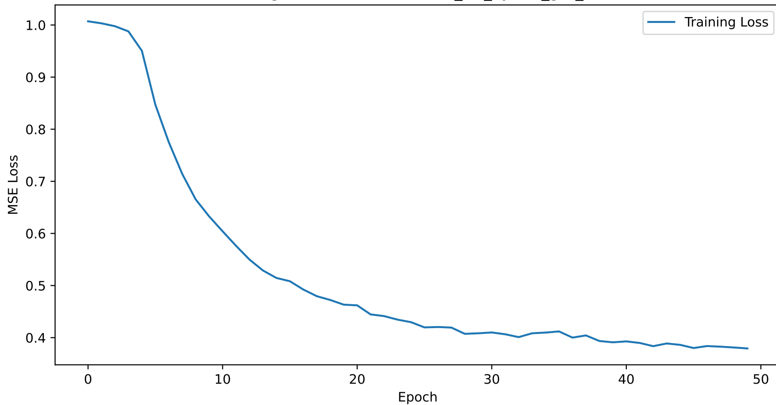
Training Loss Curve for boston_1H_hybrid_gru_lstm
