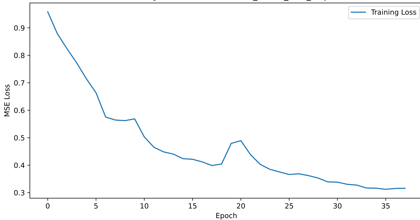
Training Loss Curve for atlanta_15min_lstm_only
