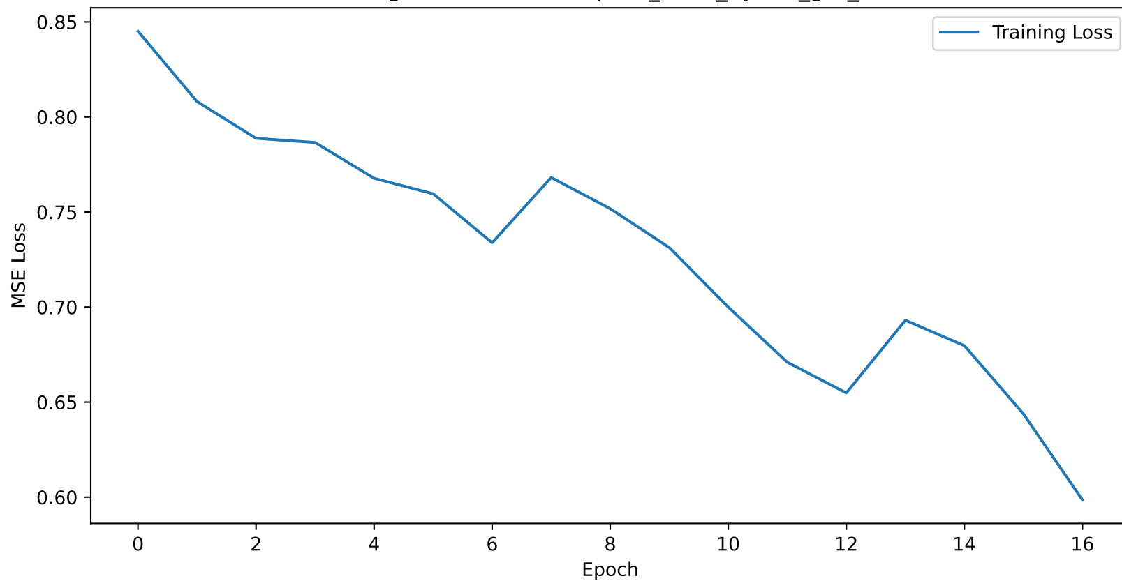
Training Loss Curve for elpaso_5min_hybrid_gru_lstm
