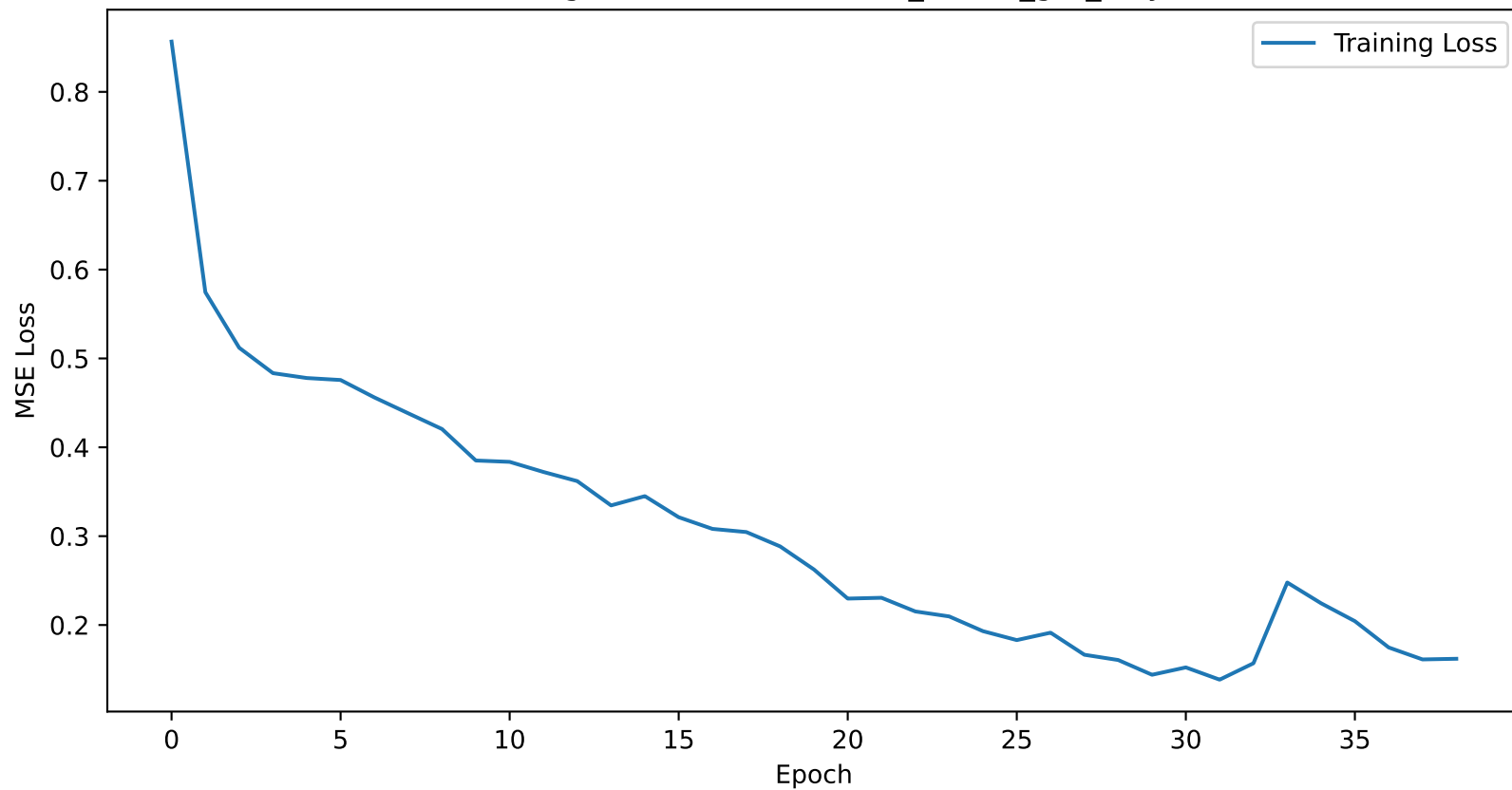
Training Loss Curve for dallas_45min_gru_only
