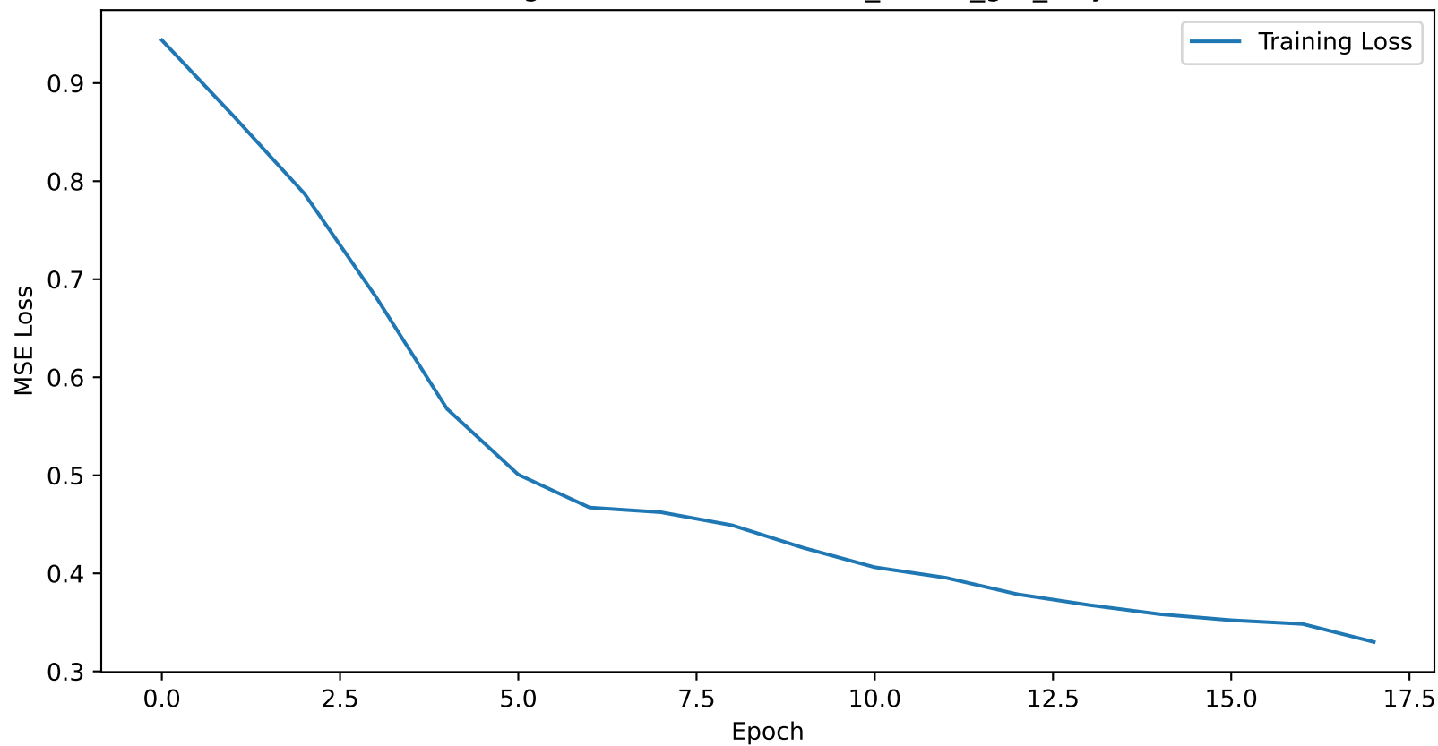
Training Loss Curve for atlanta_15min_gru_only
