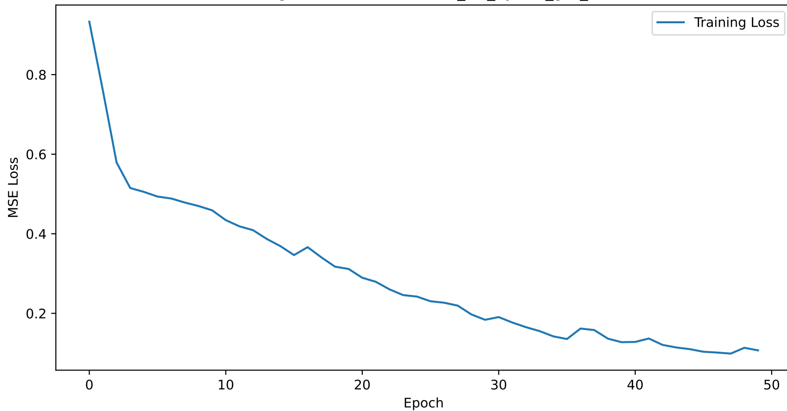
Training Loss Curve for dallas_1H_hybrid_gru_lstm
