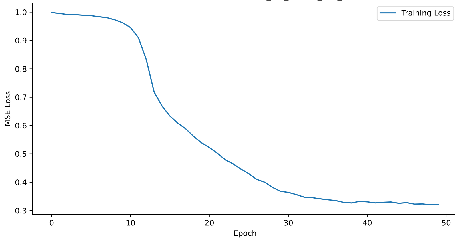
Training Loss Curve for boston_2H_hybrid_gru_lstm
