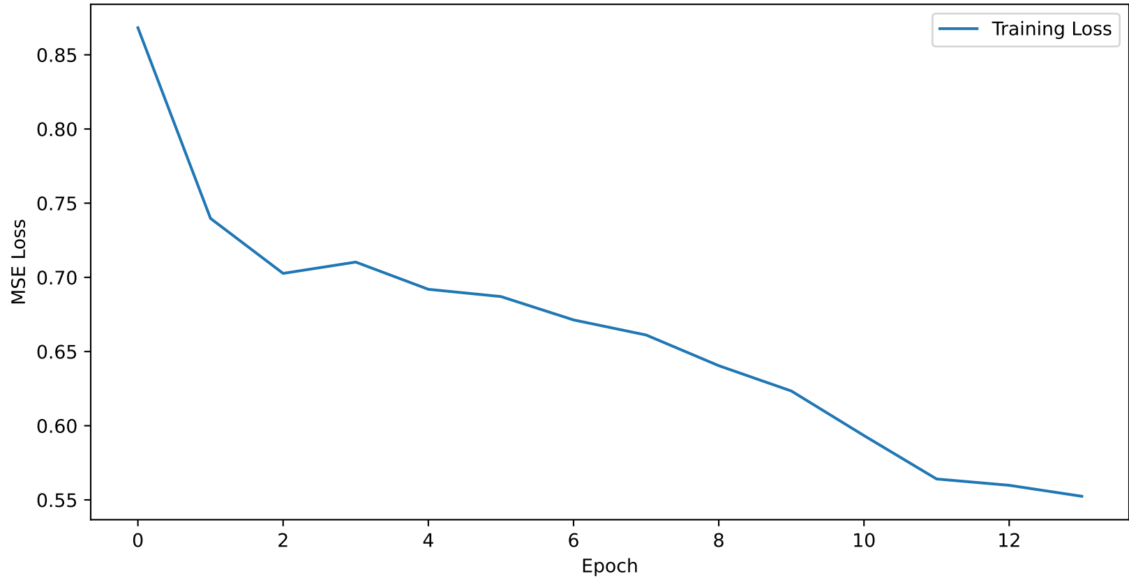
Training Loss Curve for elpaso_30min_gru_only
