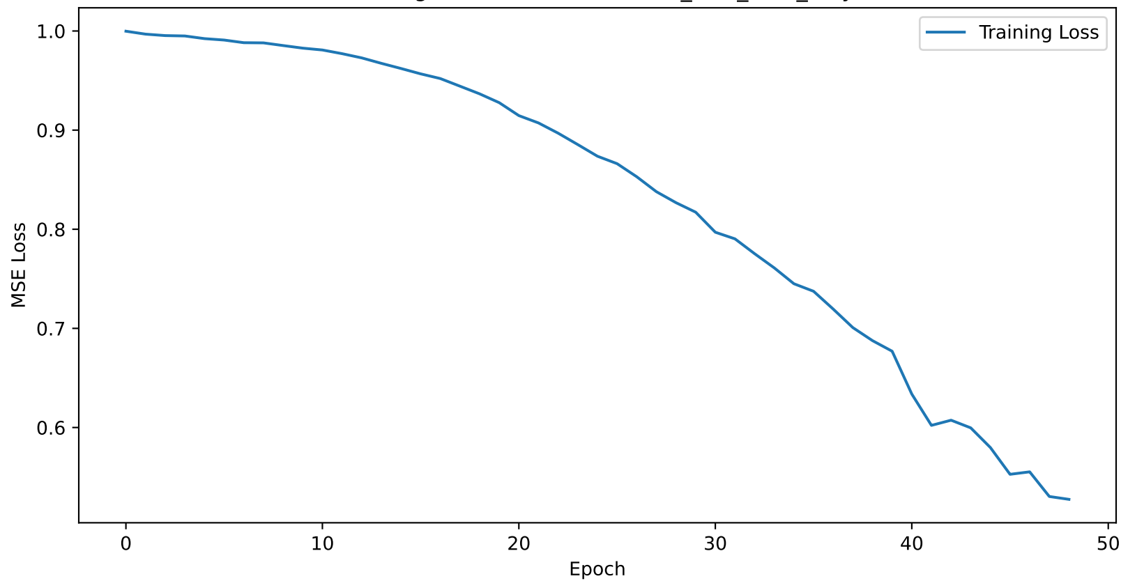
Training Loss Curve for atlanta_12H_lstm_only
