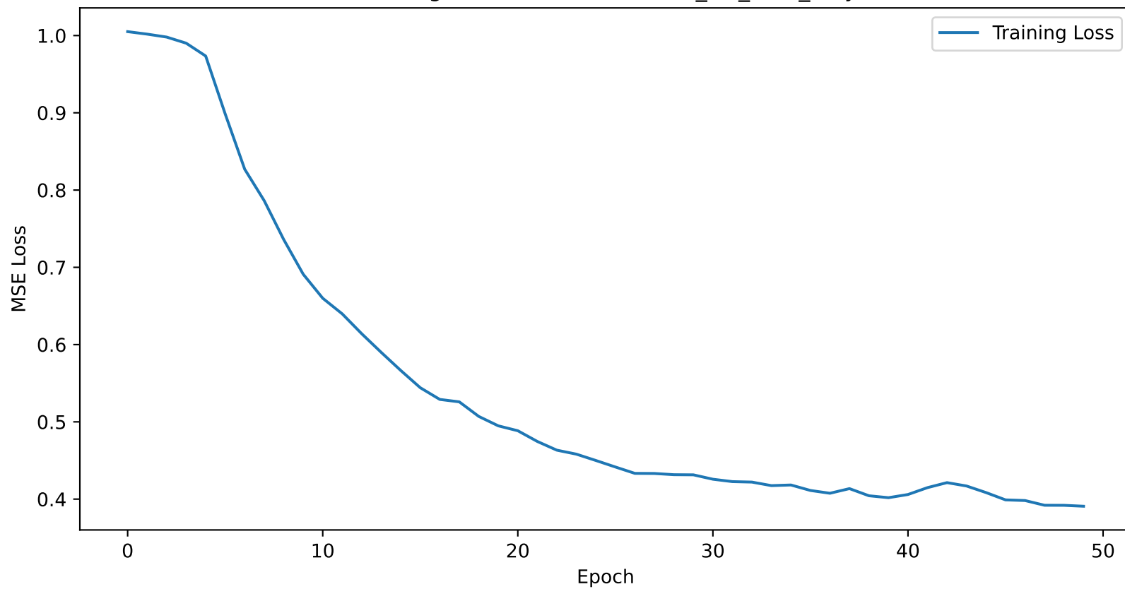
Training Loss Curve for boston_1H_lstm_only
