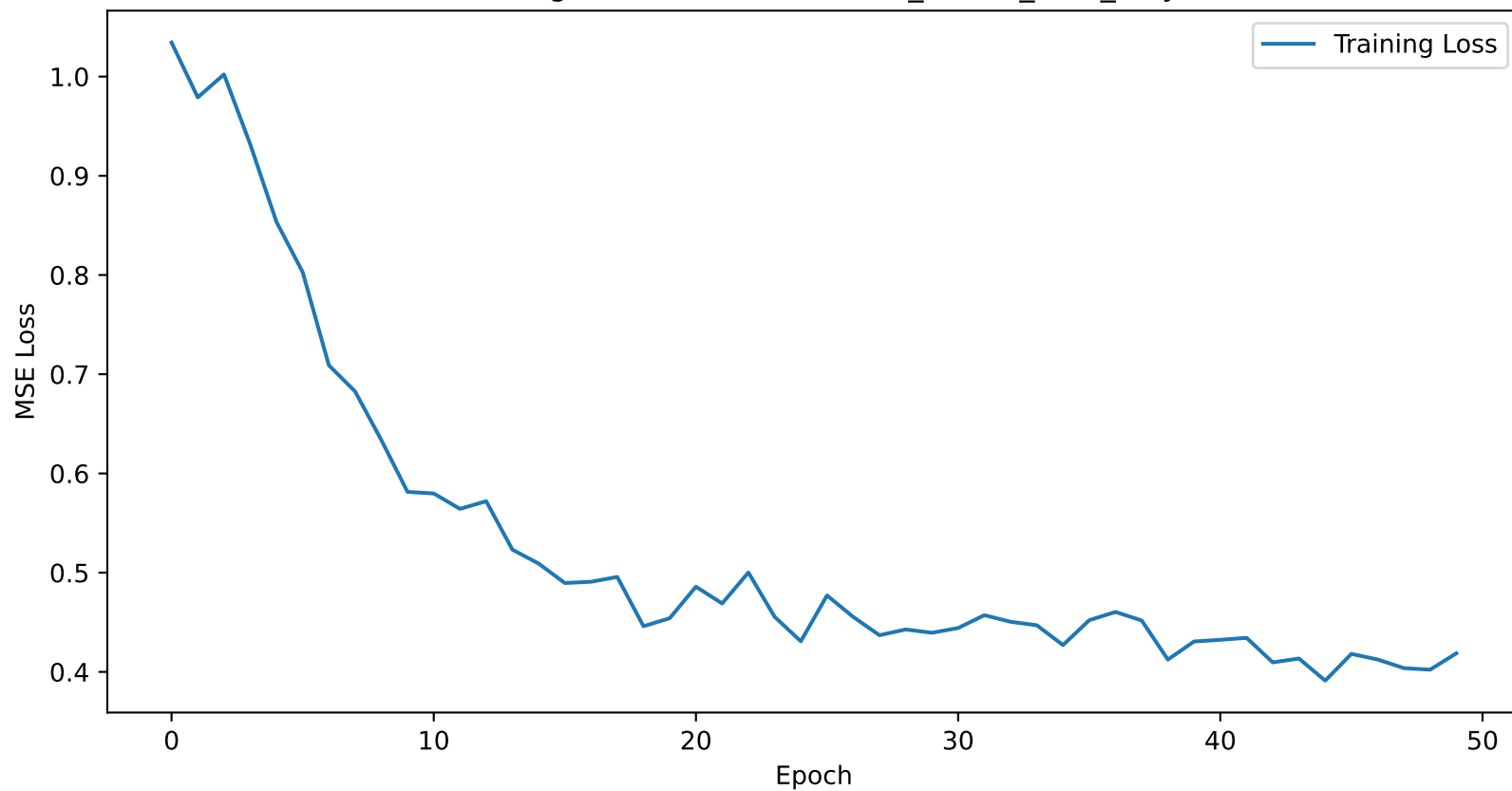
Training Loss Curve for boston_45min_lstm_only
