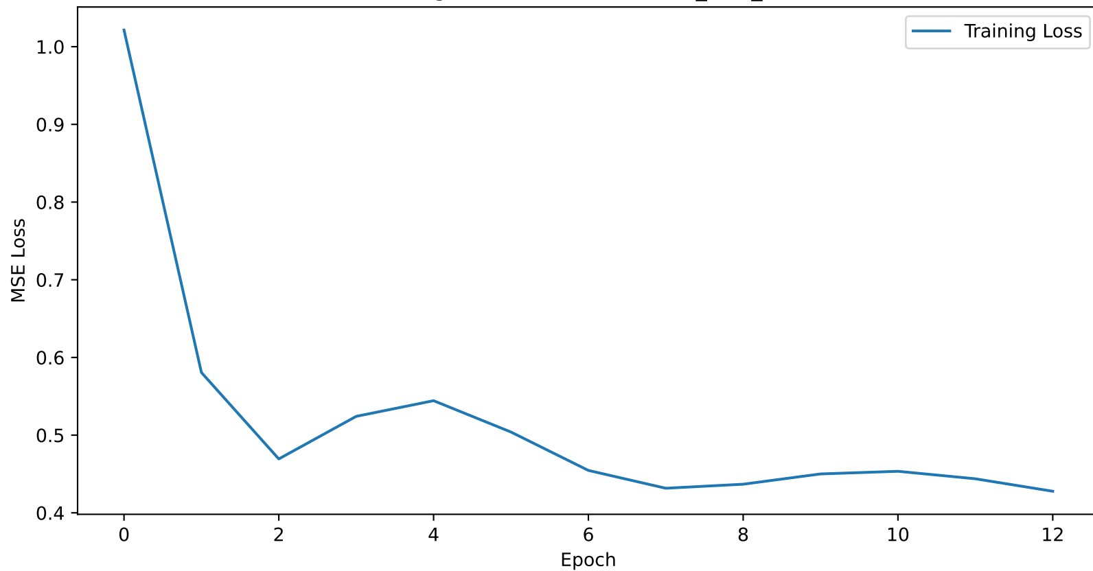
Training Loss Curve for atlanta_12H_nhits
