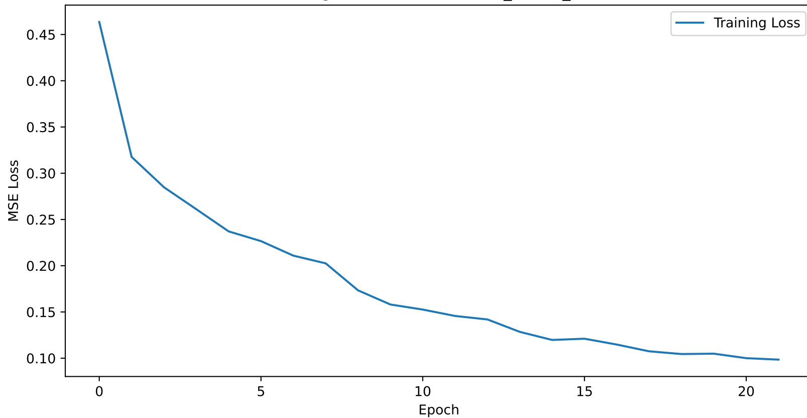
Training Loss Curve for dallas_15min_nhits
