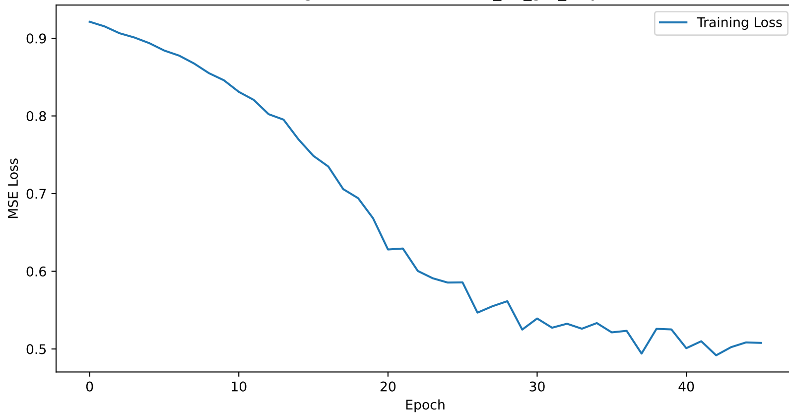
Training Loss Curve for atlanta_1D_gru_only
