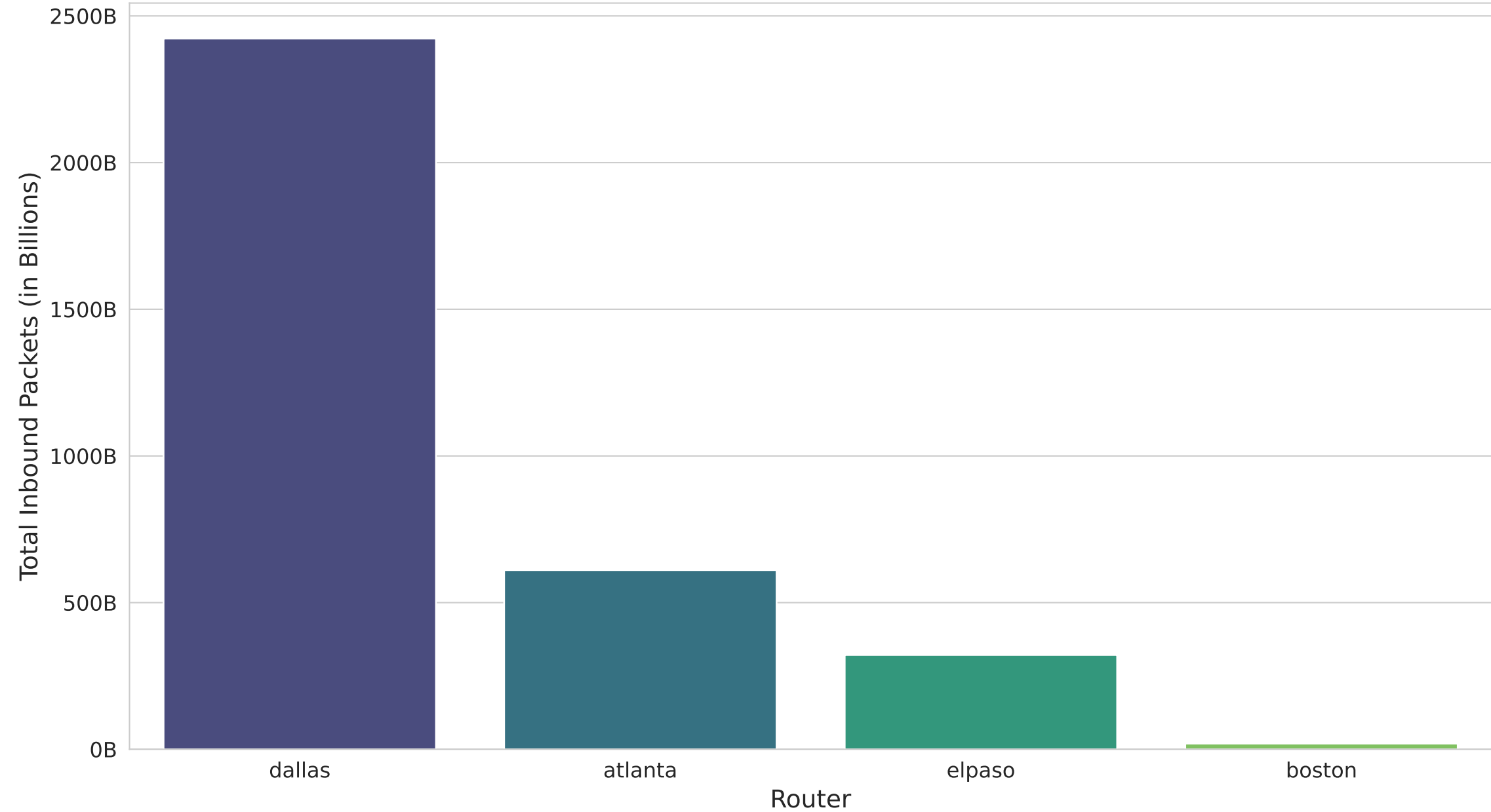
Total Traffic Volume Over 57 Days by Router
