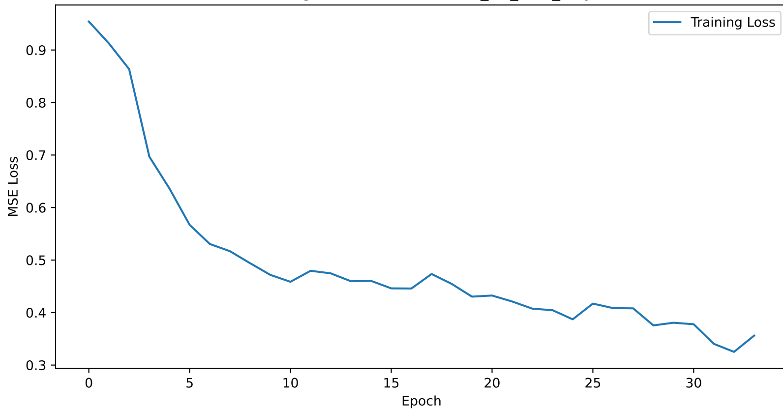
Training Loss Curve for dallas_2H_1stm_only
