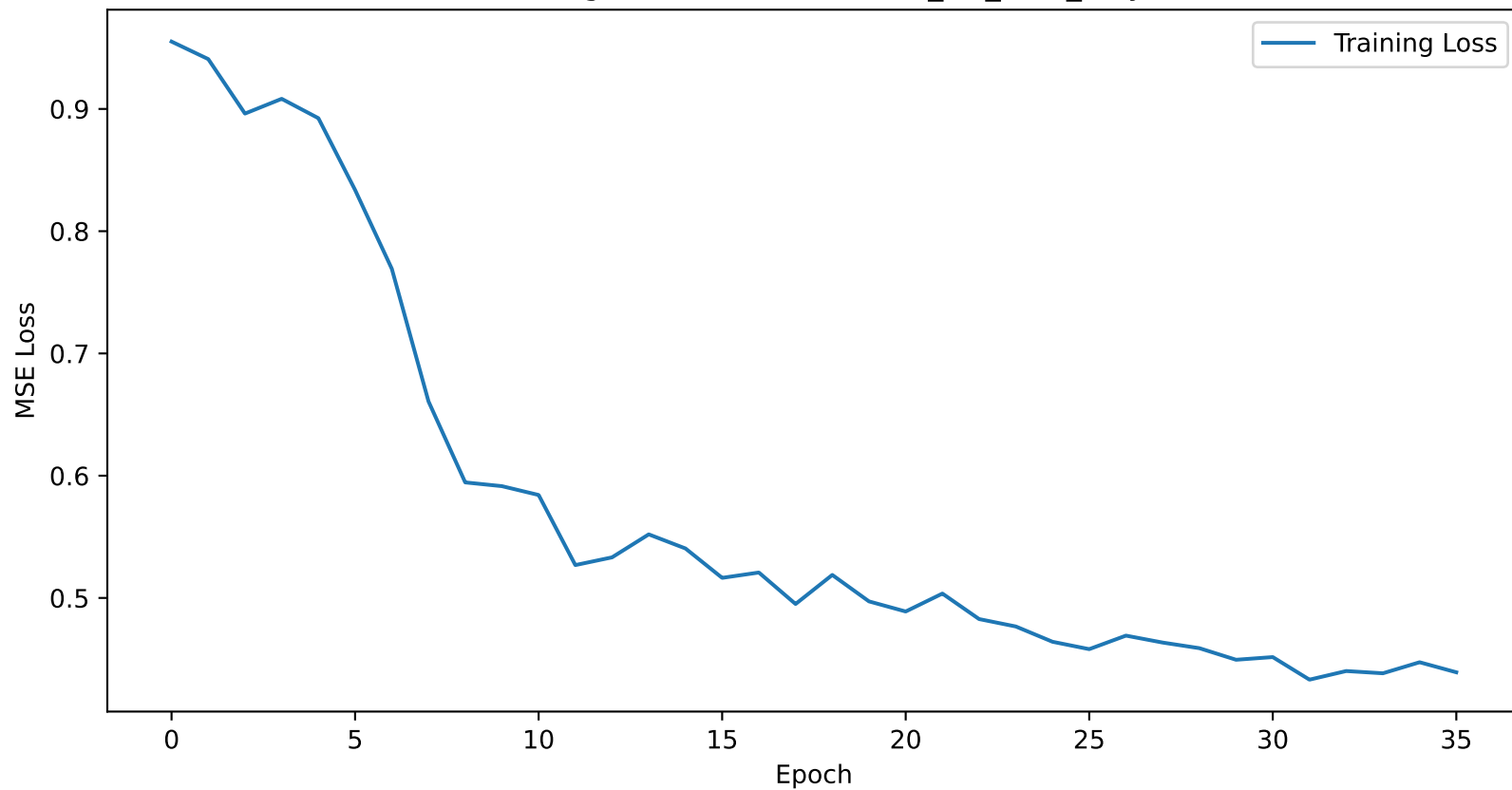
Training Loss Curve for dallas_4H_lstm_only
