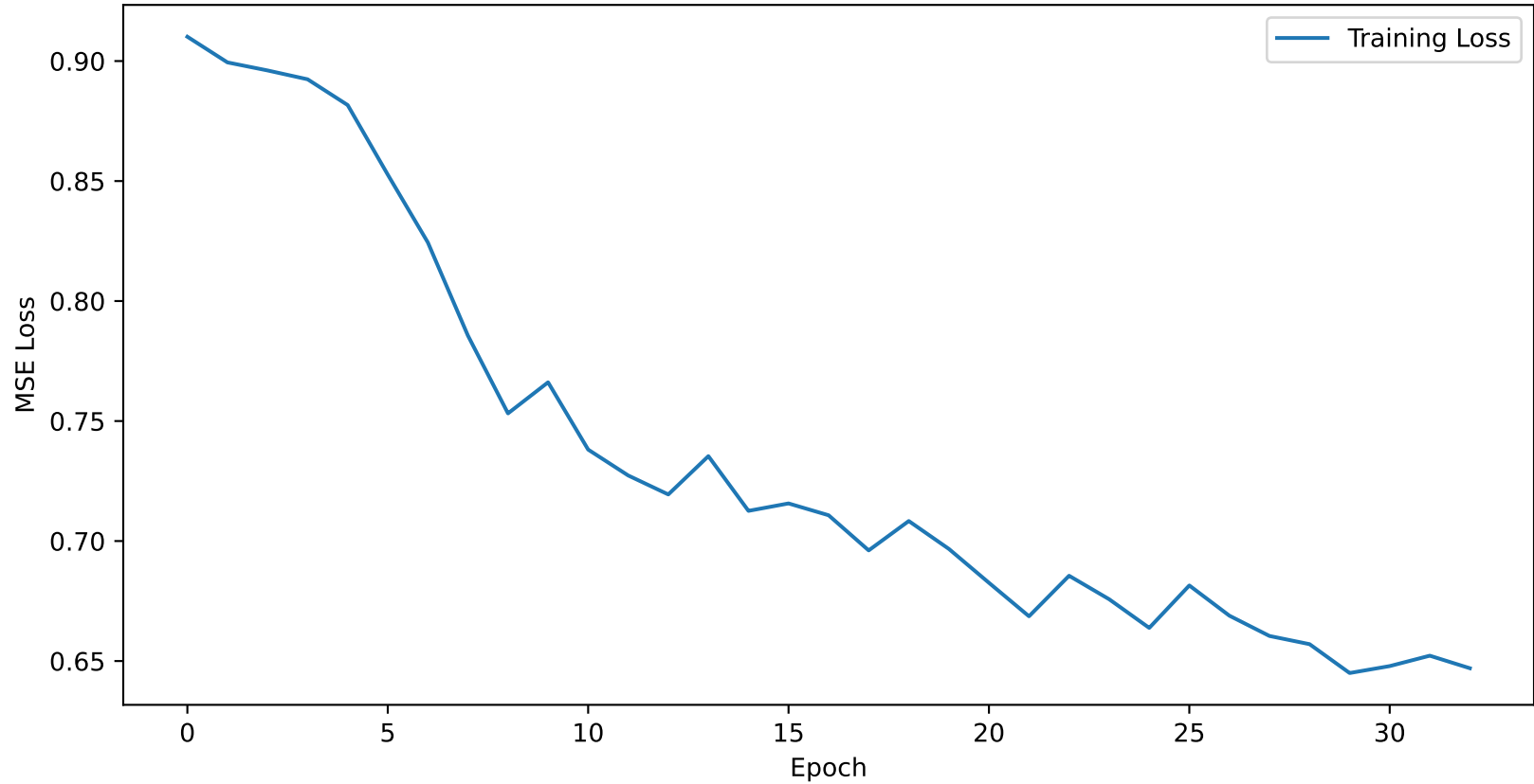
Training Loss Curve for elpaso_4H_lstm_only
