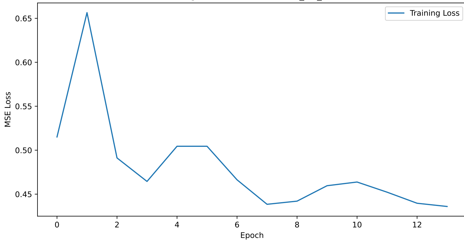
Training Loss Curve for boston_1D_nhits
