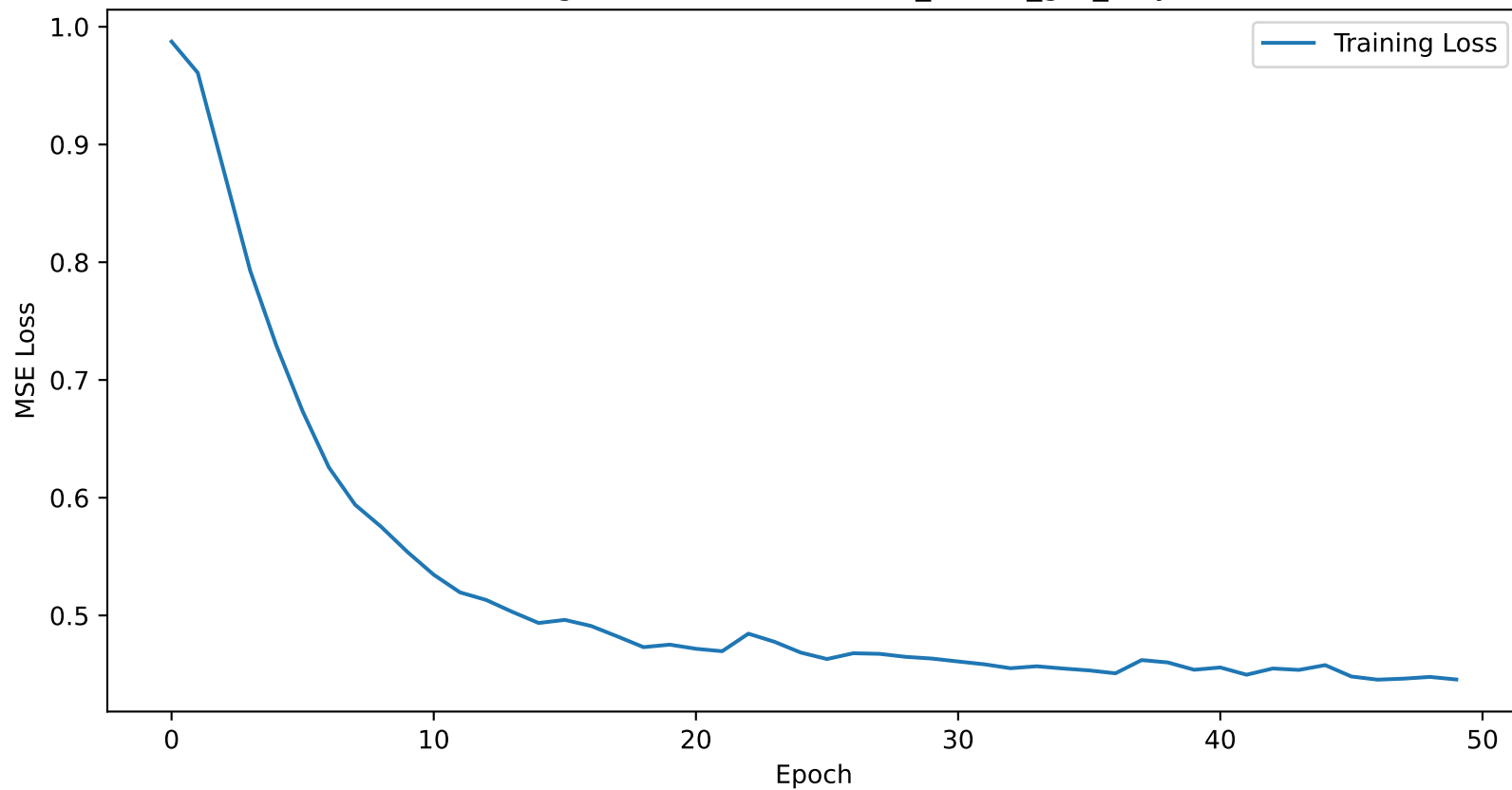
Training Loss Curve for boston_30min_gru_only
