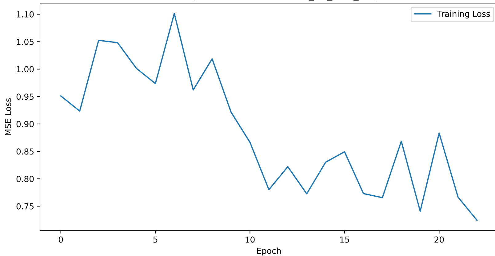
Training Loss Curve for atlanta_6H_lstm_only
