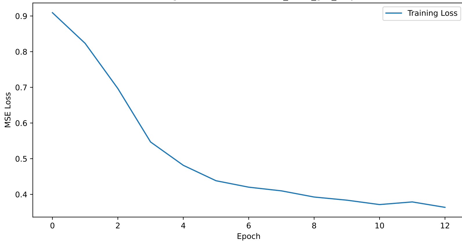
Training Loss Curve for atlanta_5min_gru_only
