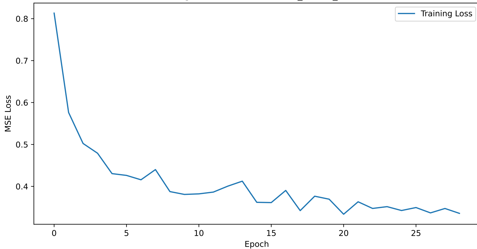
Training Loss Curve for boston_45min_nhits
