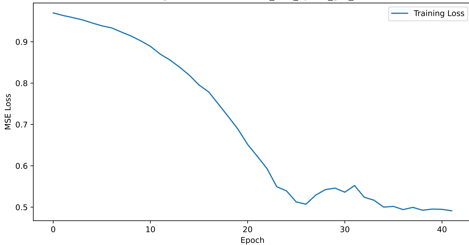
Training Loss Curve for dallas_12H_hybrid_gru_lstm
