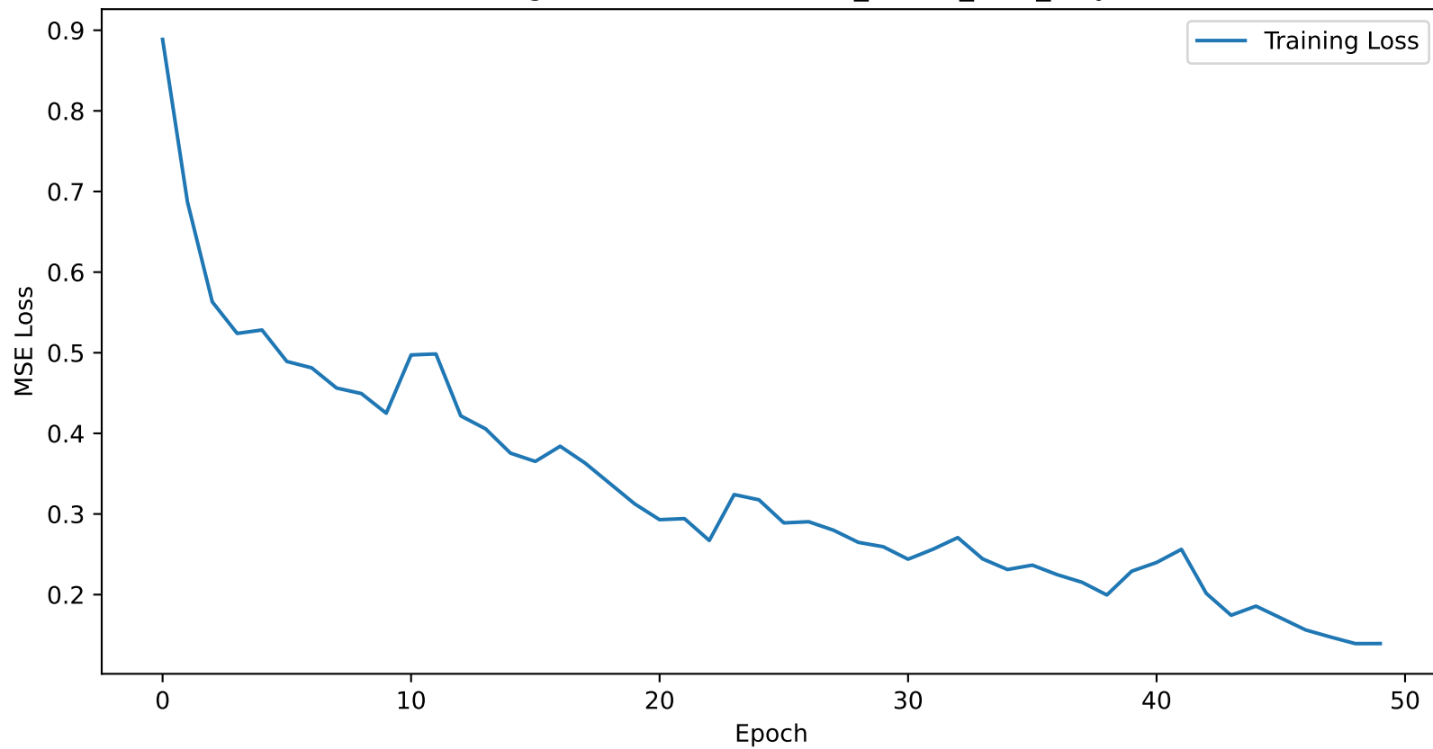
Training Loss Curve for dallas_30min_lstm_only
