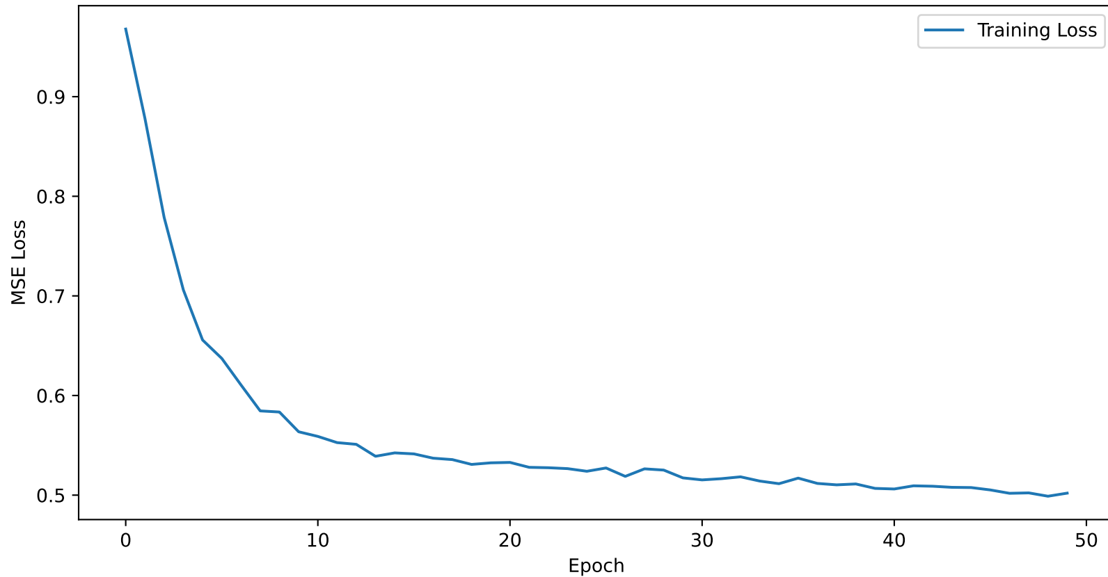
Training Loss Curve for boston_15min_gru_only
