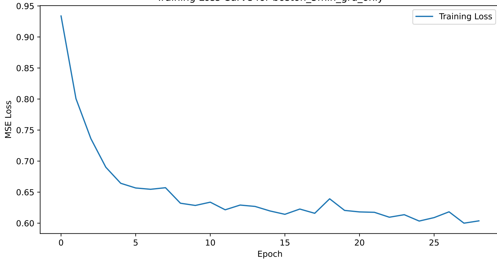
Training Loss Curve for boston_5min_gru_only
