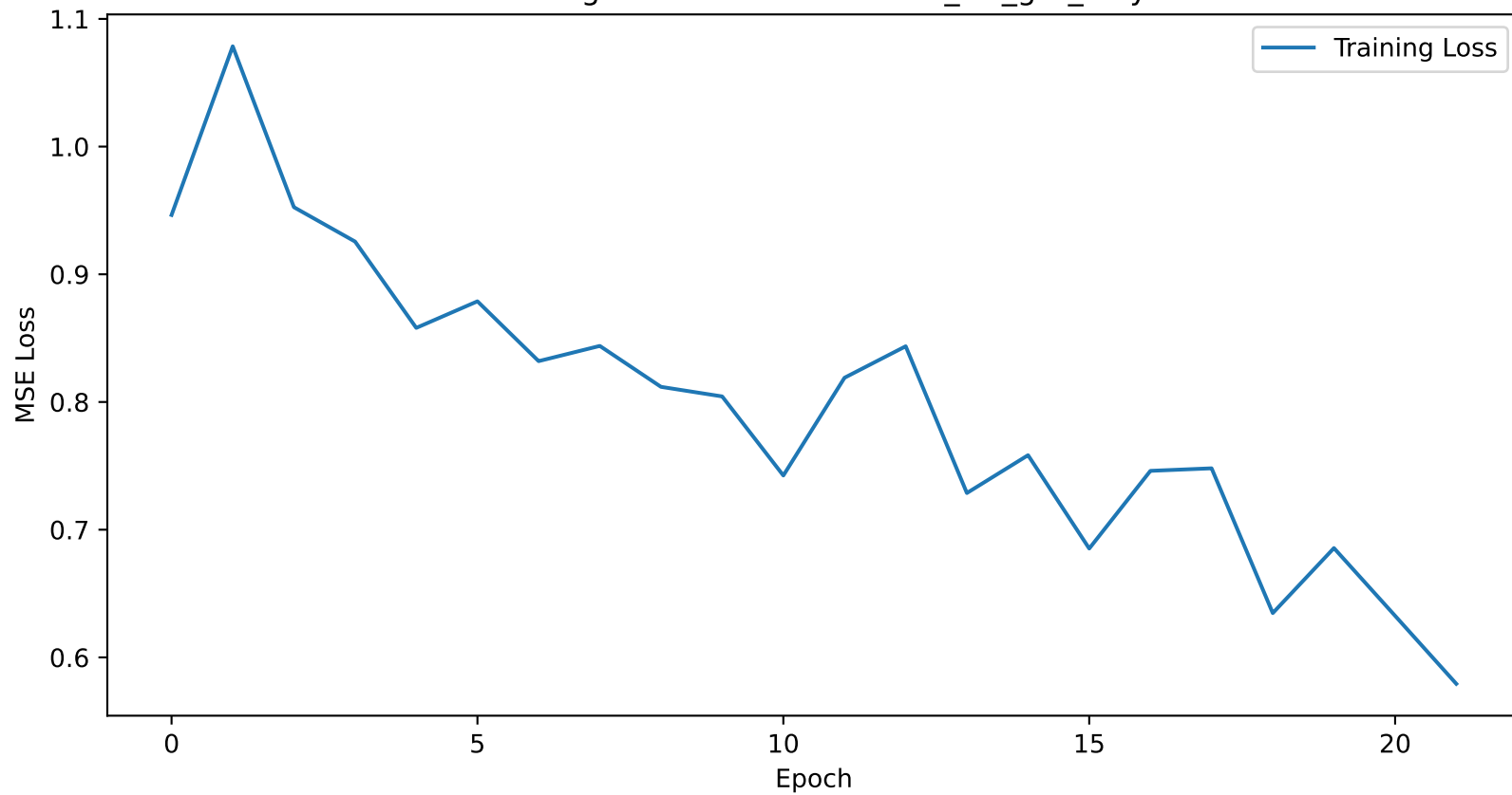
Training Loss Curve for atlanta_6H_gru_only
