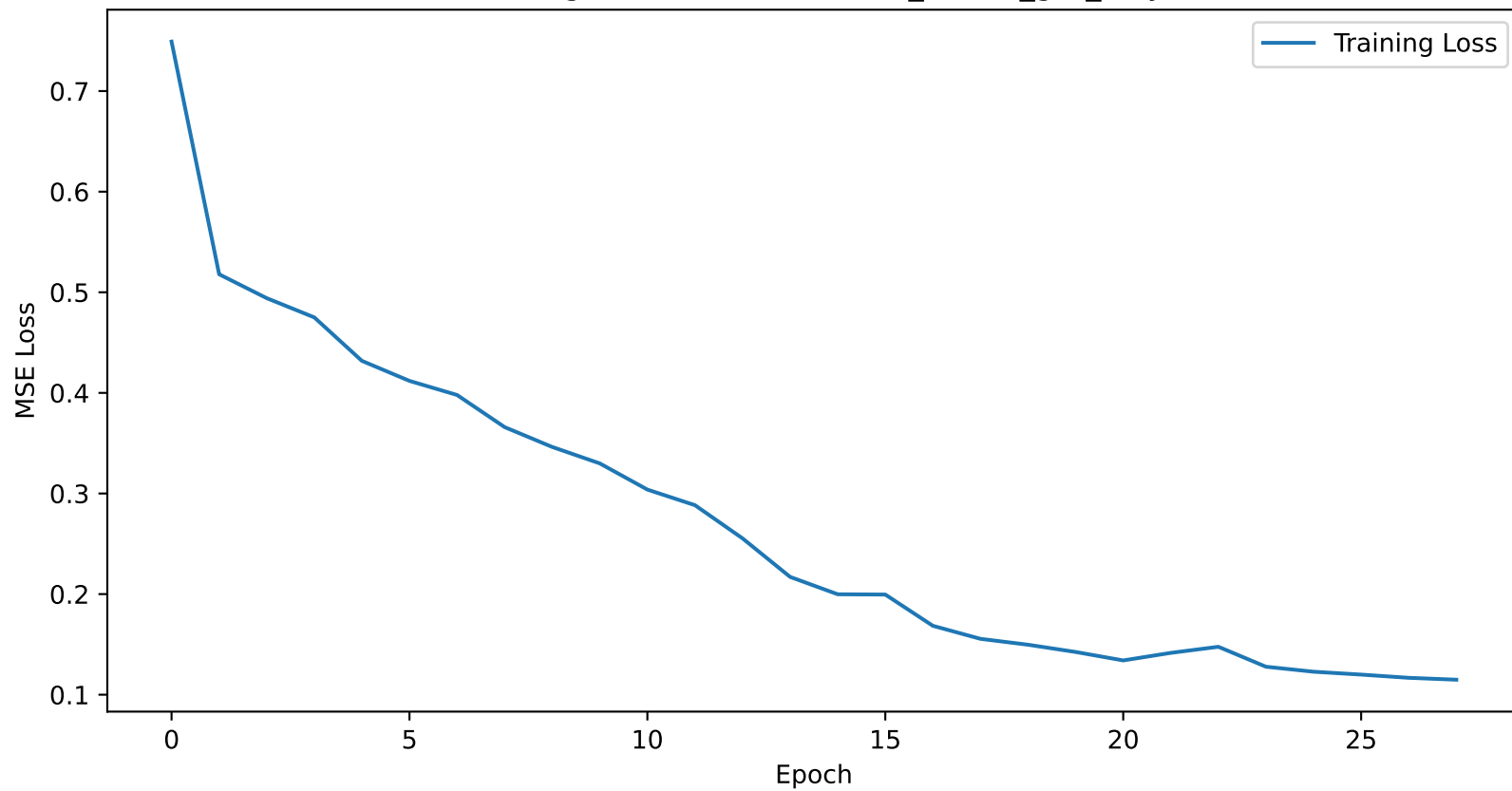
Training Loss Curve for dallas_15min_gru_only
