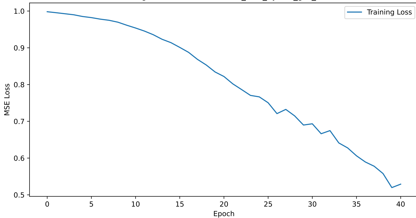
Training Loss Curve for atlanta_12H_hybrid_gru_lstm
