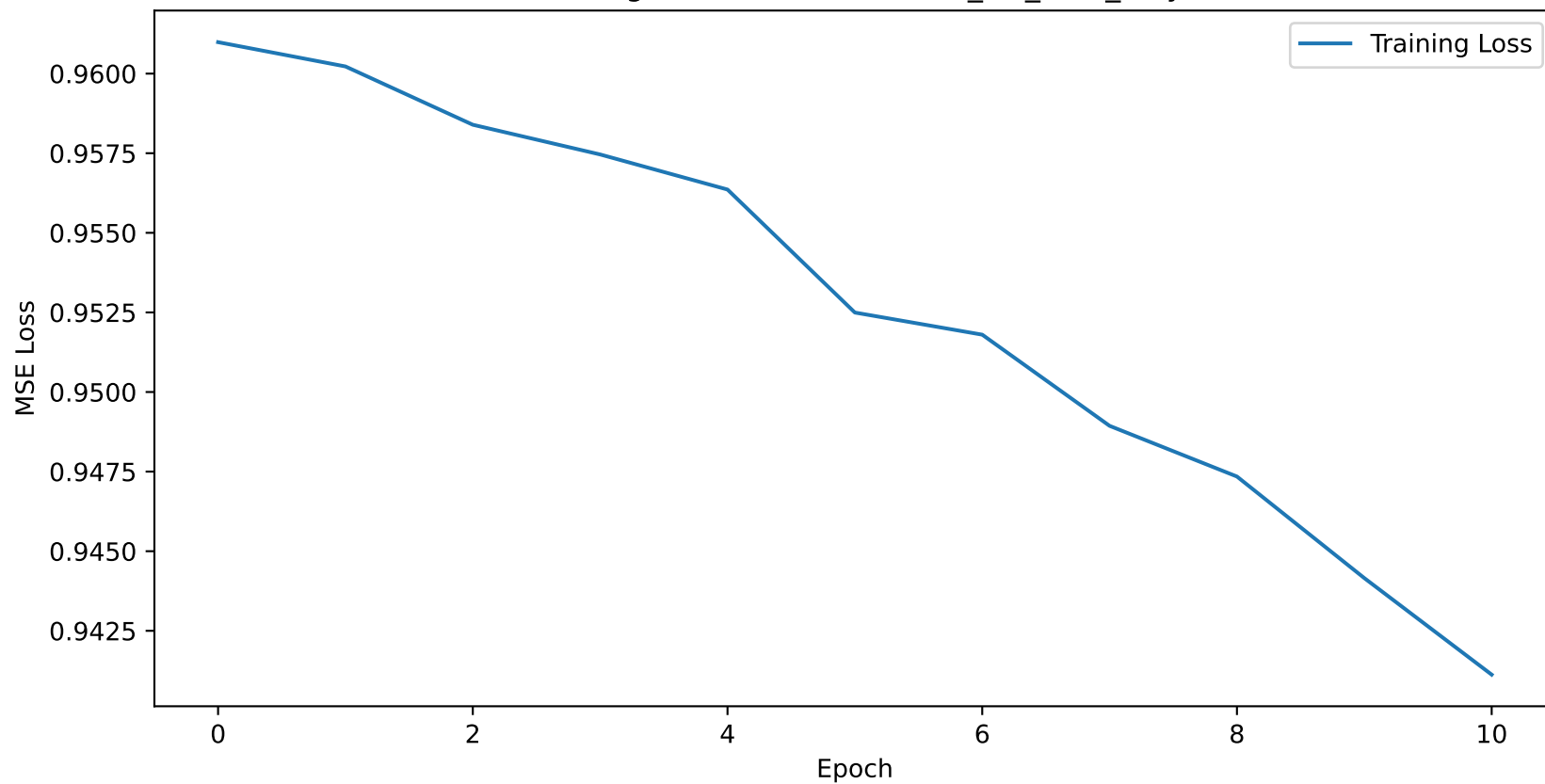
Training Loss Curve for dallas_1D_lstm_only
