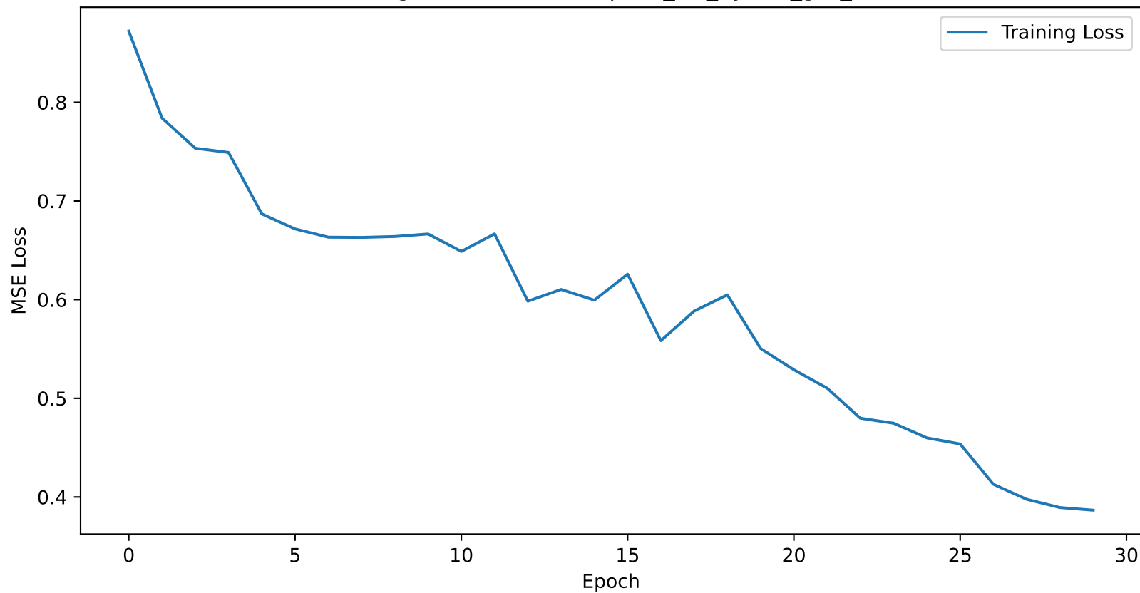
Training Loss Curve for elpaso_1H_hybrid_gru_lstm
