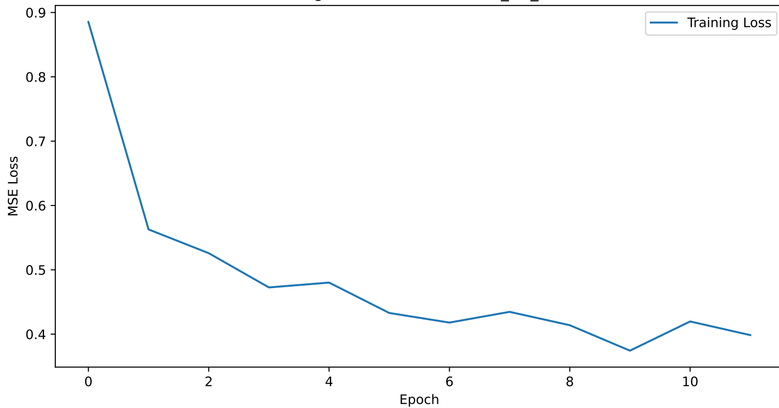
Training Loss Curve for atlanta_6H_nhits
