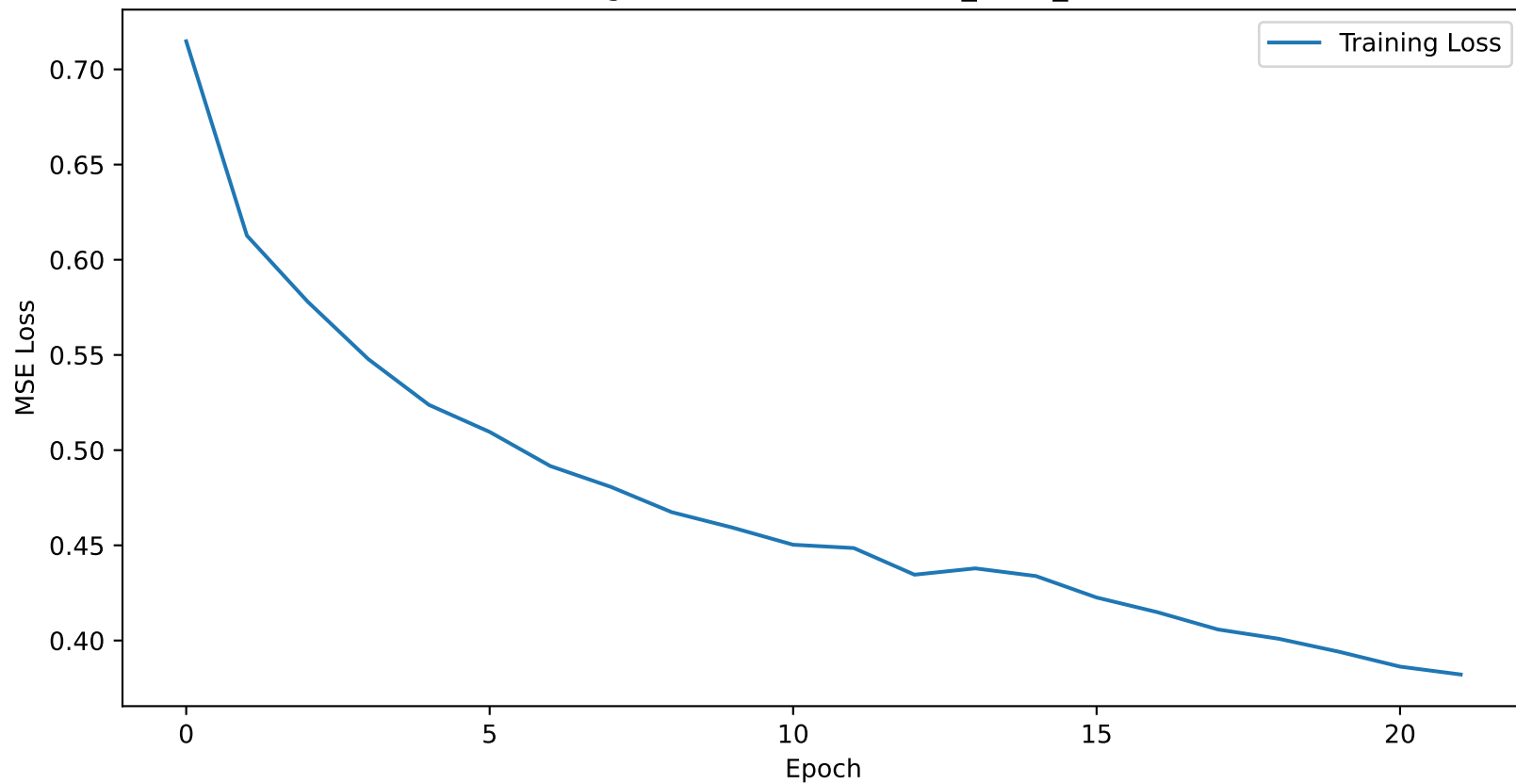
Training Loss Curve for boston_5min_nhits
