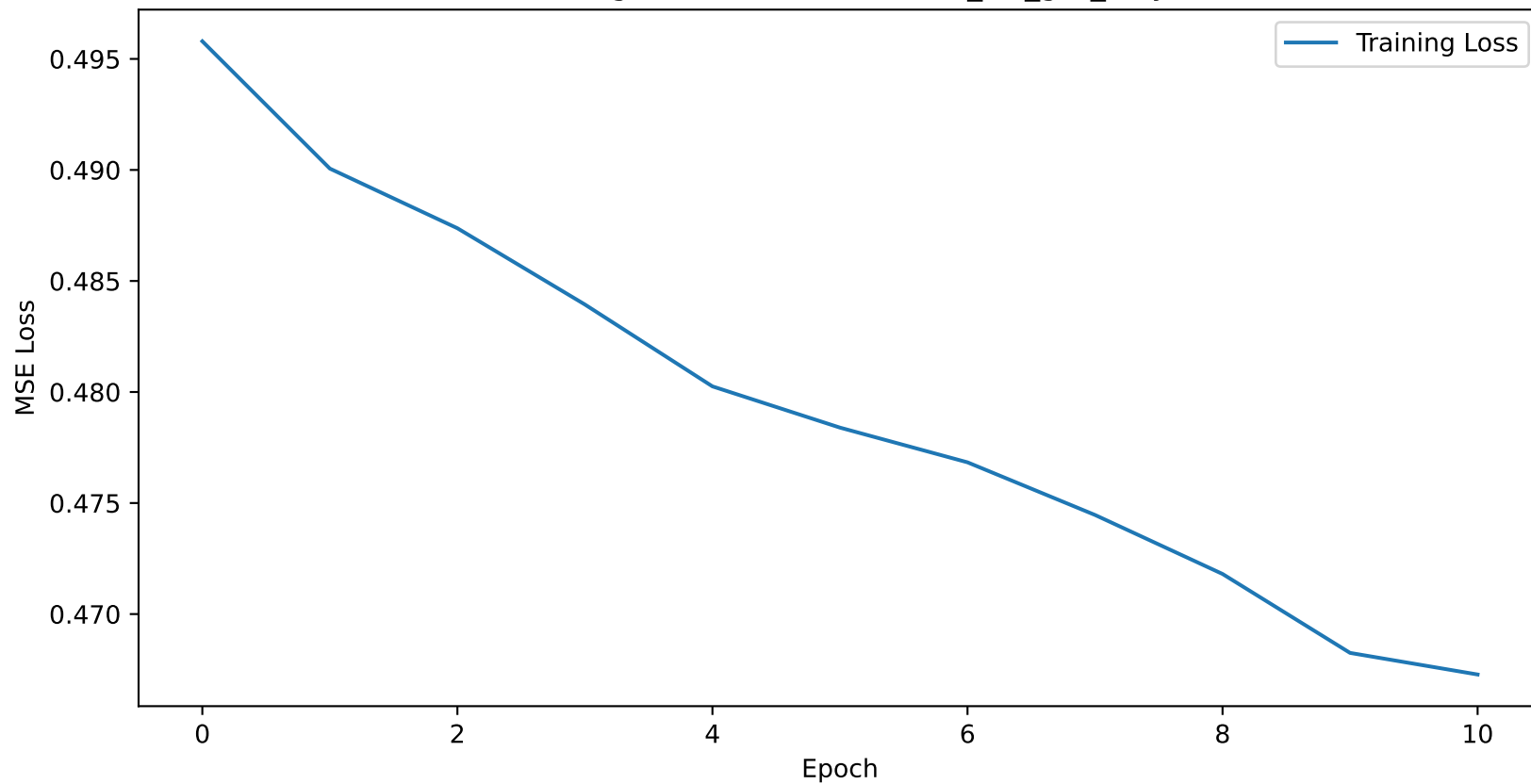
Training Loss Curve for boston_1D_gru_only
