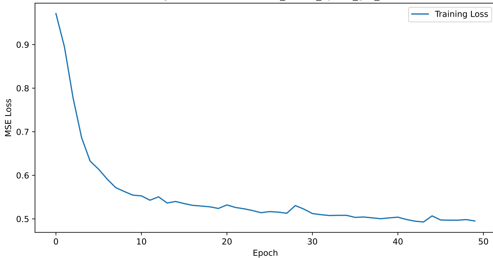
Training Loss Curve for boston_15min_hybrid_gru_lstm
