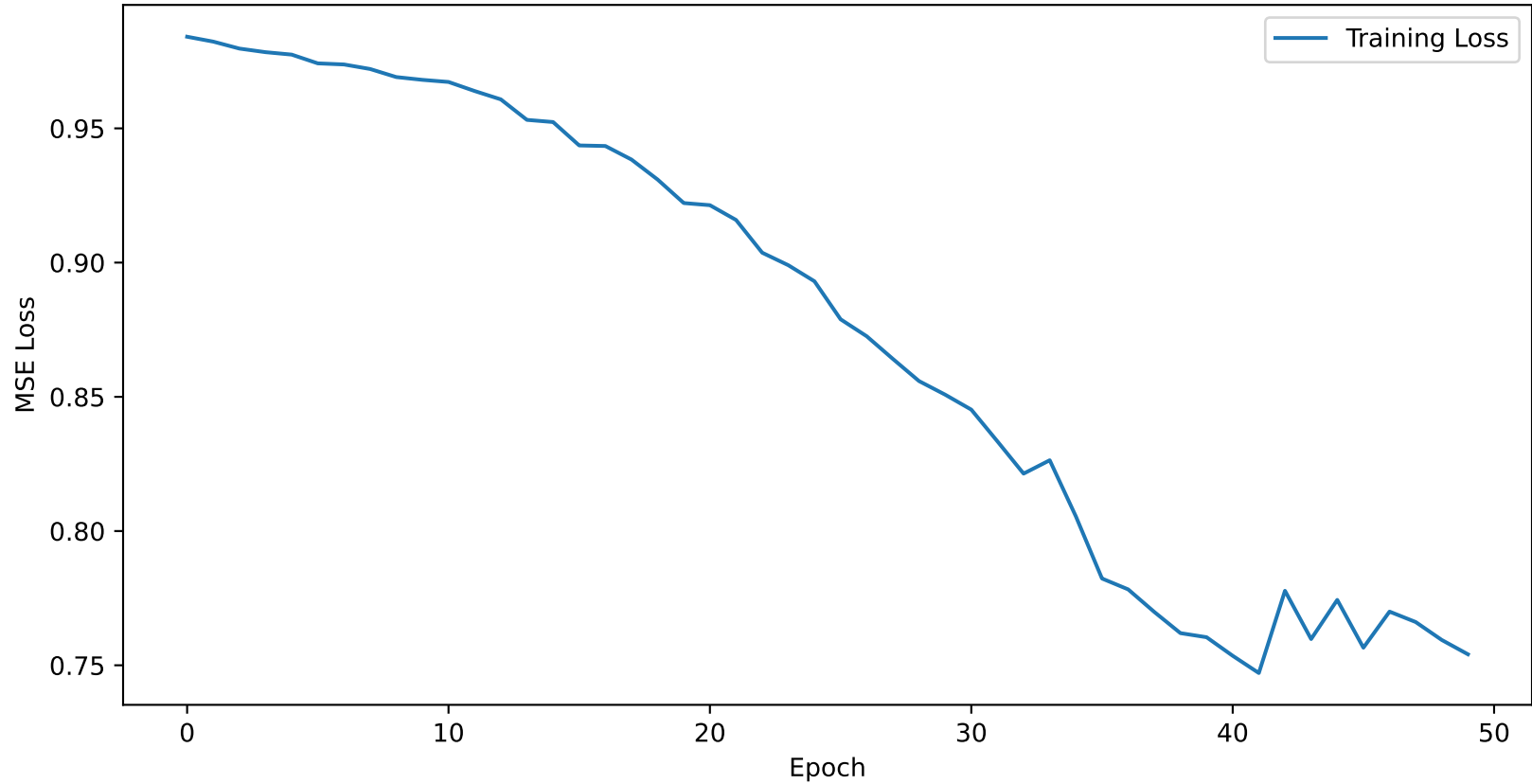
Training Loss Curve for elpaso_1D_lstm_only
