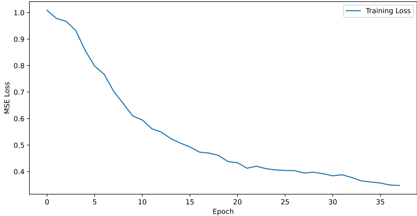
Training Loss Curve for atlanta_2H_hybrid_gru_lstm
