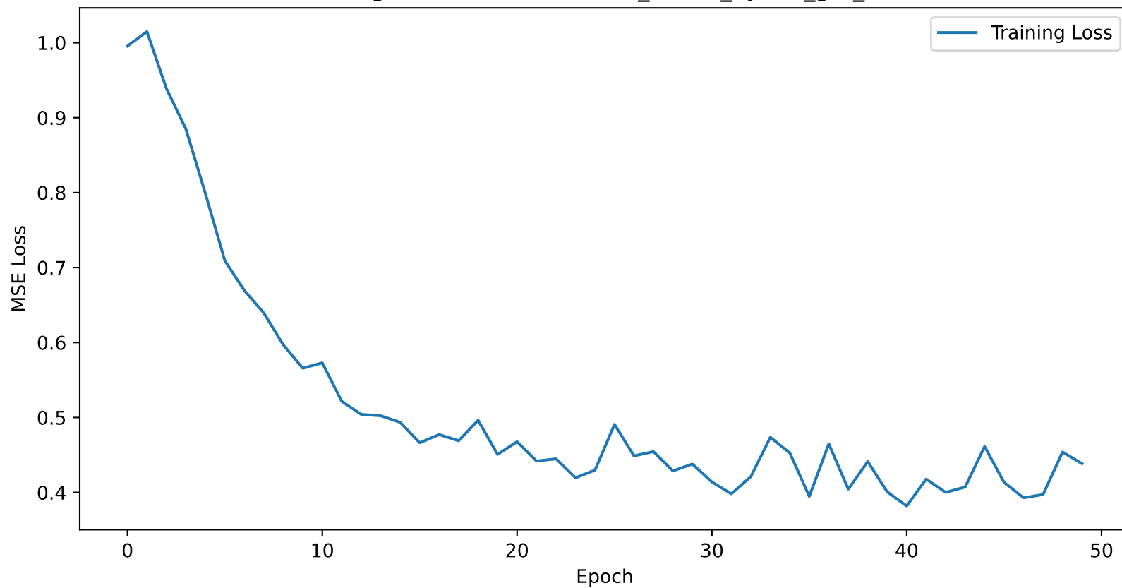
Training Loss Curve for boston_45min_hybrid_gru_lstm
