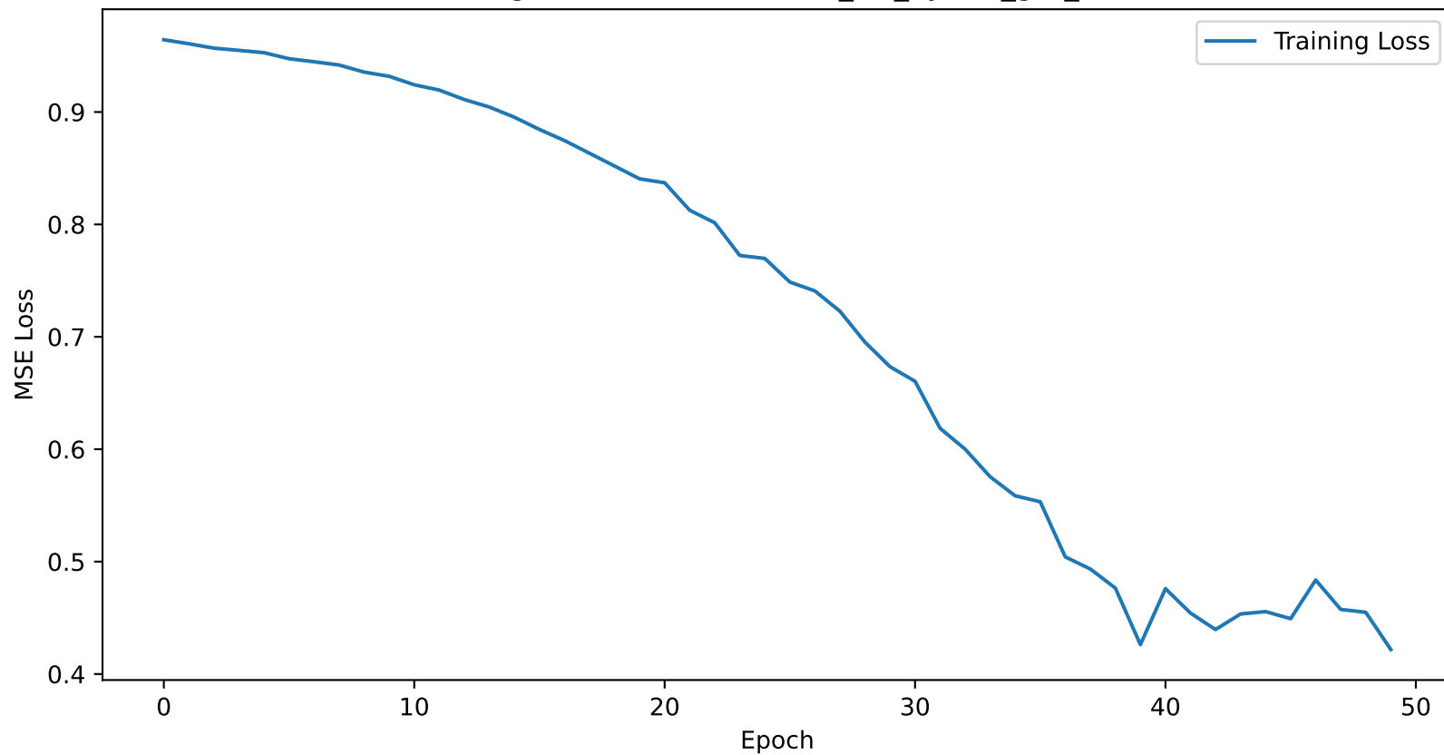
Training Loss Curve for dallas_1D_hybrid_gru_lstm
