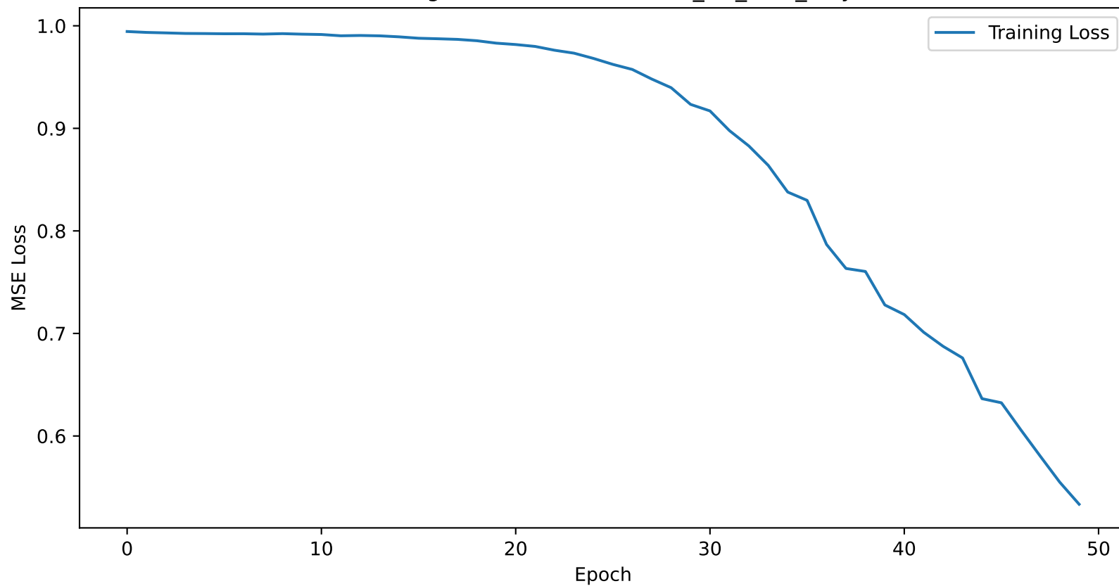
Training Loss Curve for boston_4H_lstm_only
