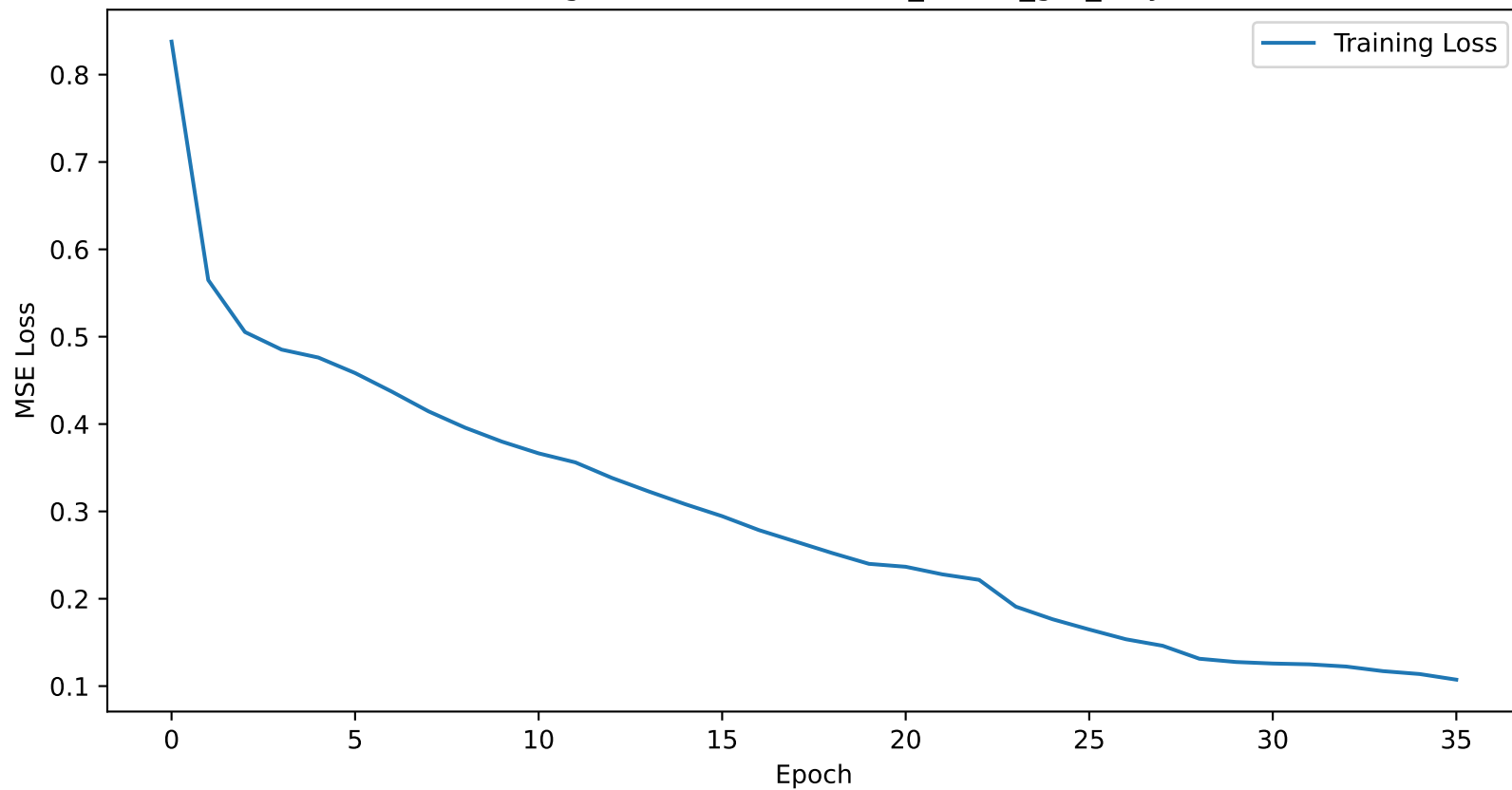
Training Loss Curve for dallas_30min_gru_only
