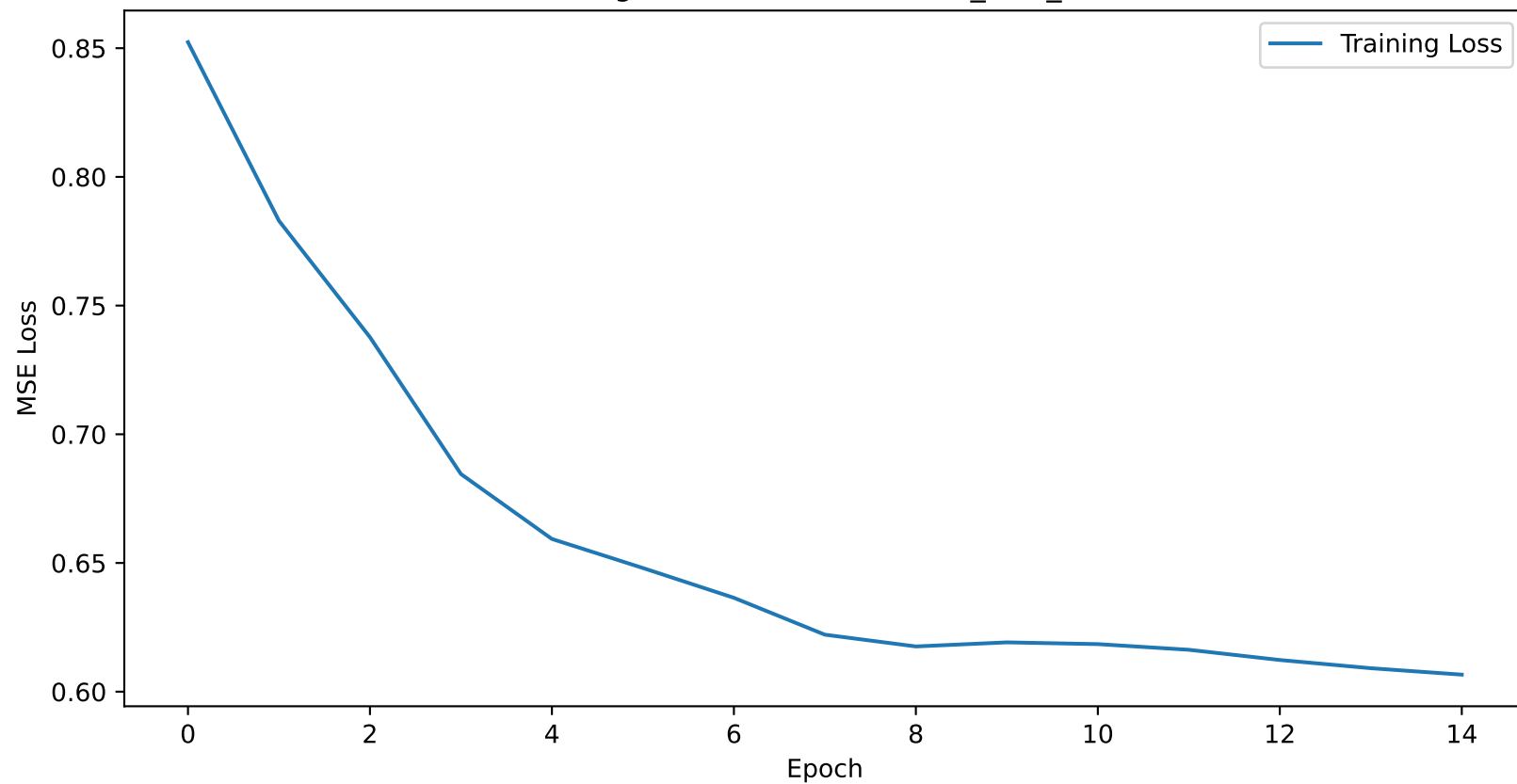
Training Loss Curve for boston_12H_nhits
