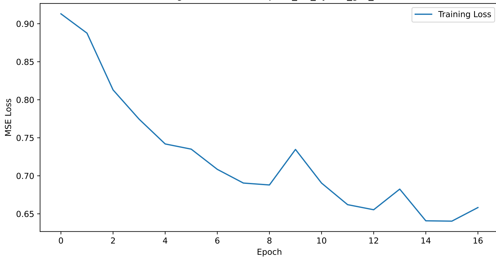
Training Loss Curve for elpaso_2H_hybrid_gru_lstm
