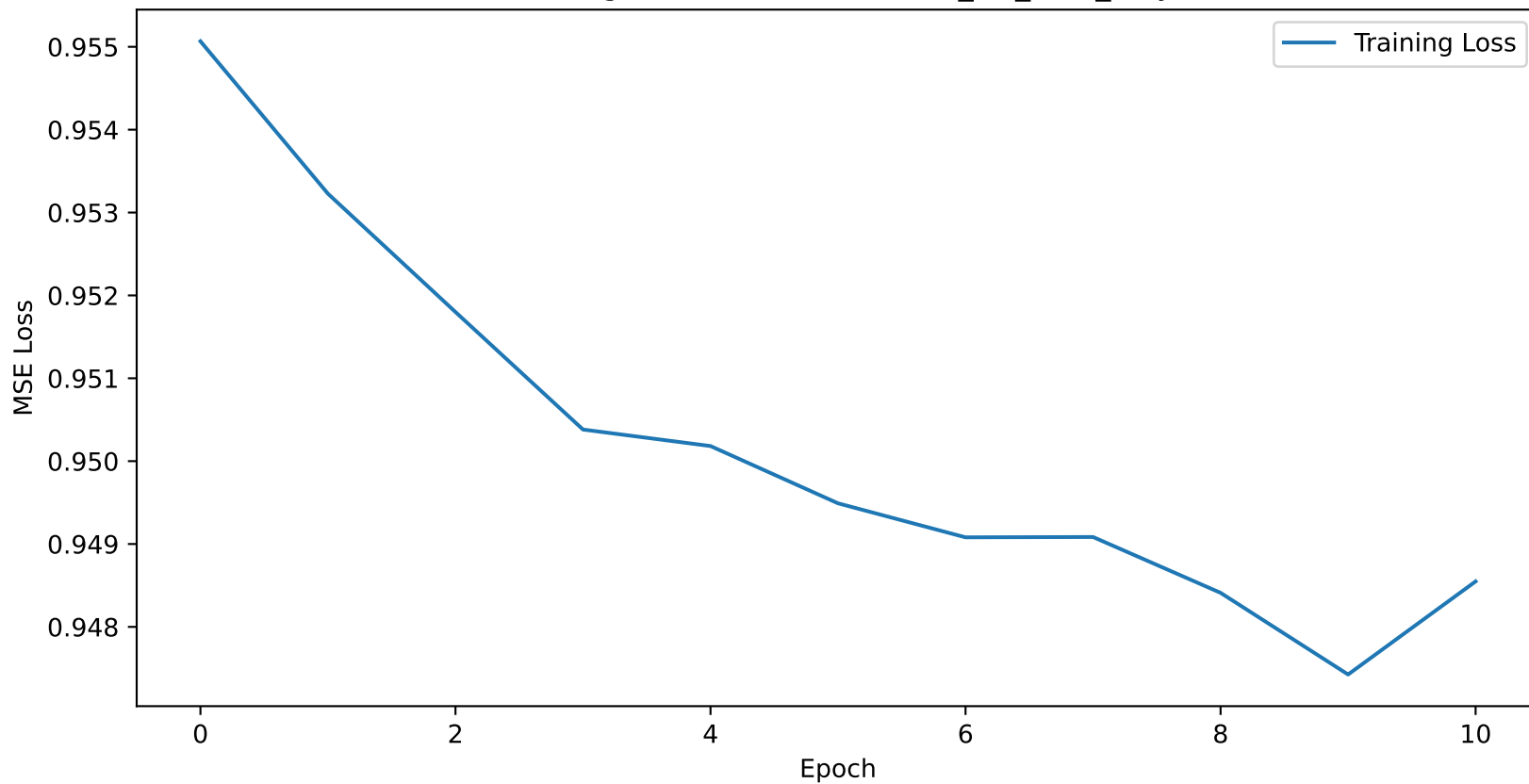
Training Loss Curve for boston_6H_lstm_only
