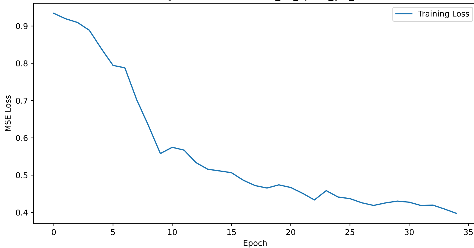
Training Loss Curve for dallas_4H_hybrid_gru_lstm
