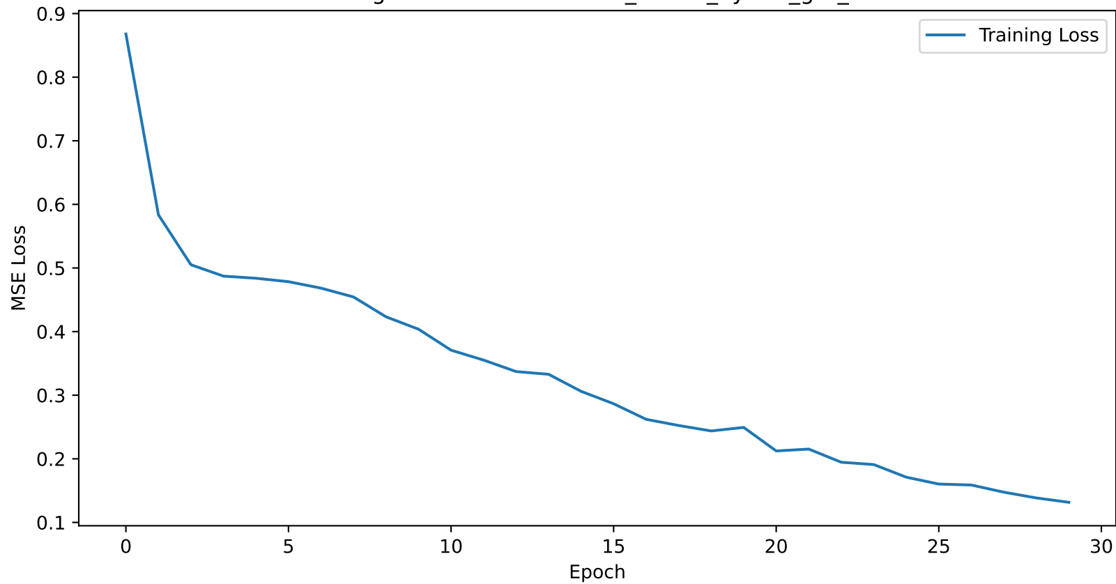
Training Loss Curve for dallas_30min_hybrid_gru_lstm
