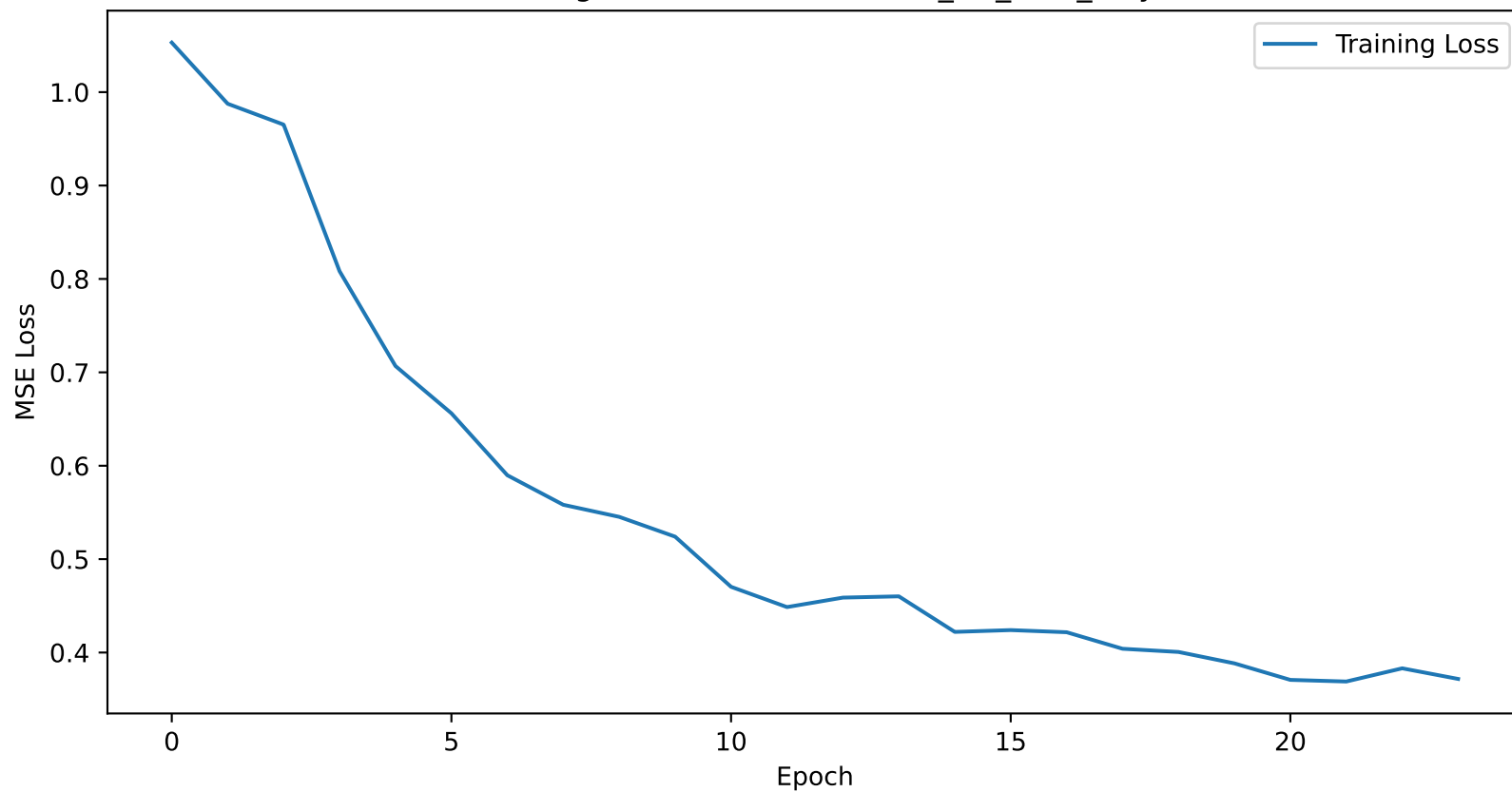
Training Loss Curve for atlanta_1H_lstm_only
