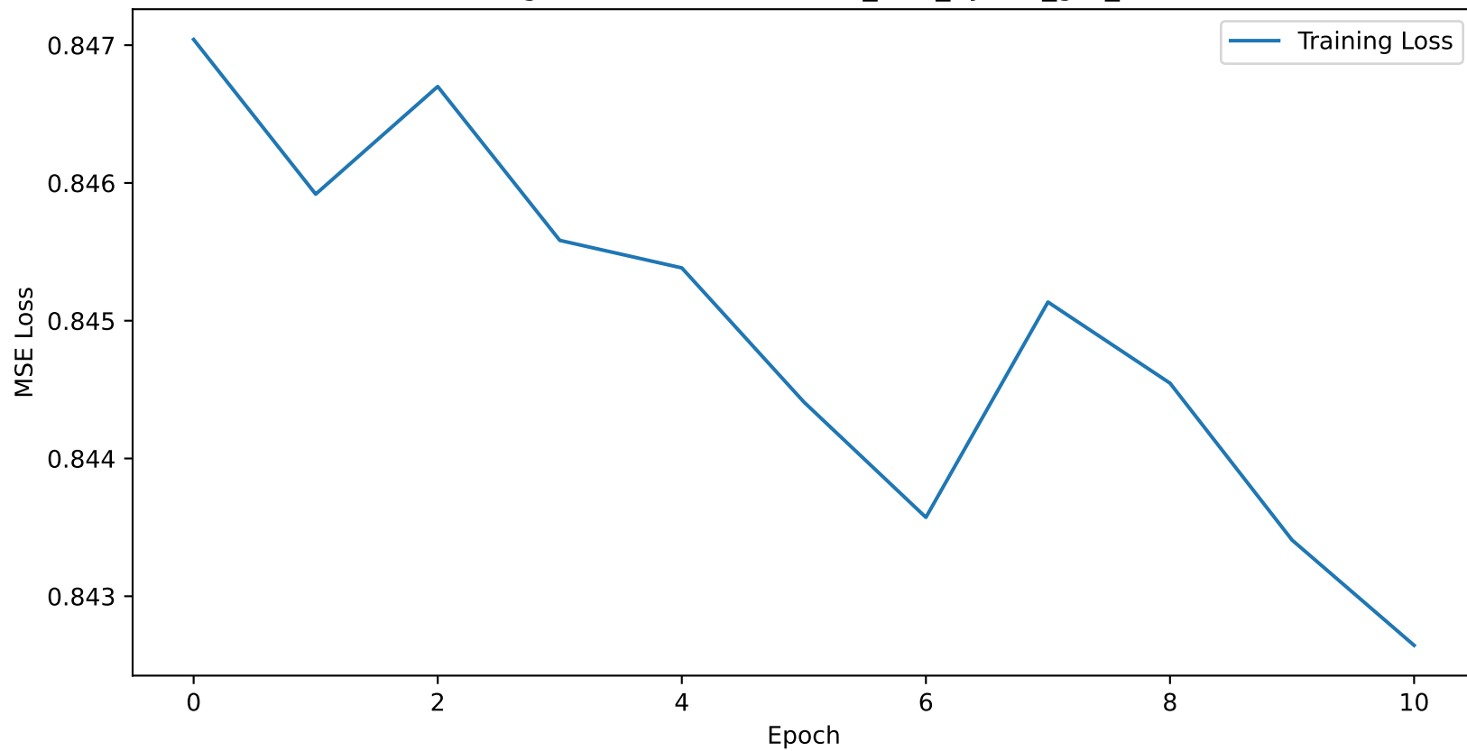
Training Loss Curve for boston_12H_hybrid_gru_lstm
