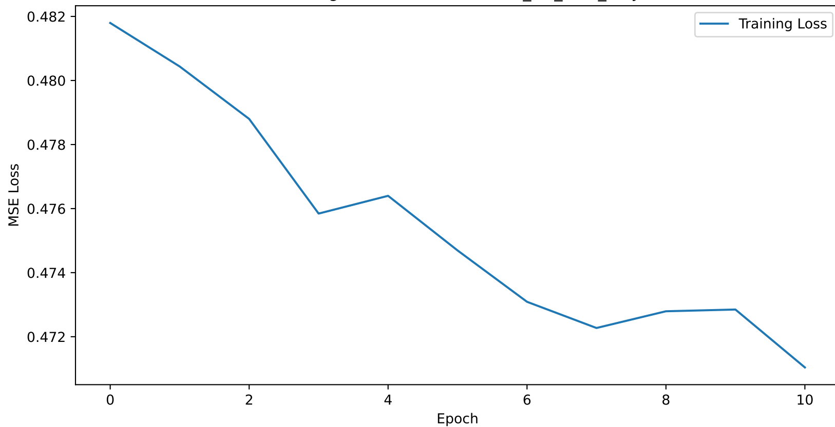
Training Loss Curve for boston_1D_lstm_only
