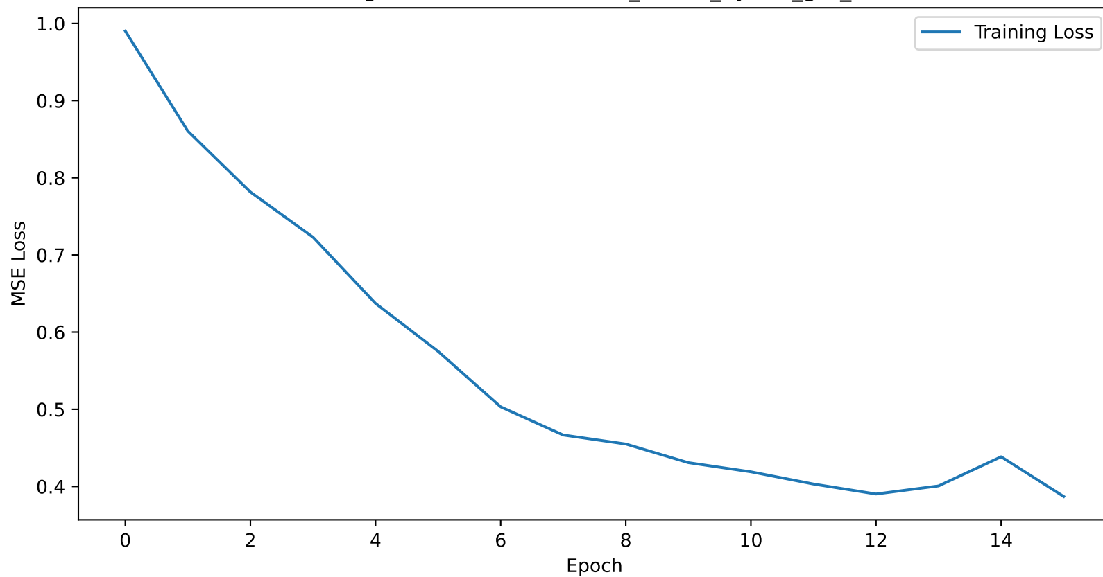
Training Loss Curve for atlanta_30min_hybrid_gru_lstm
