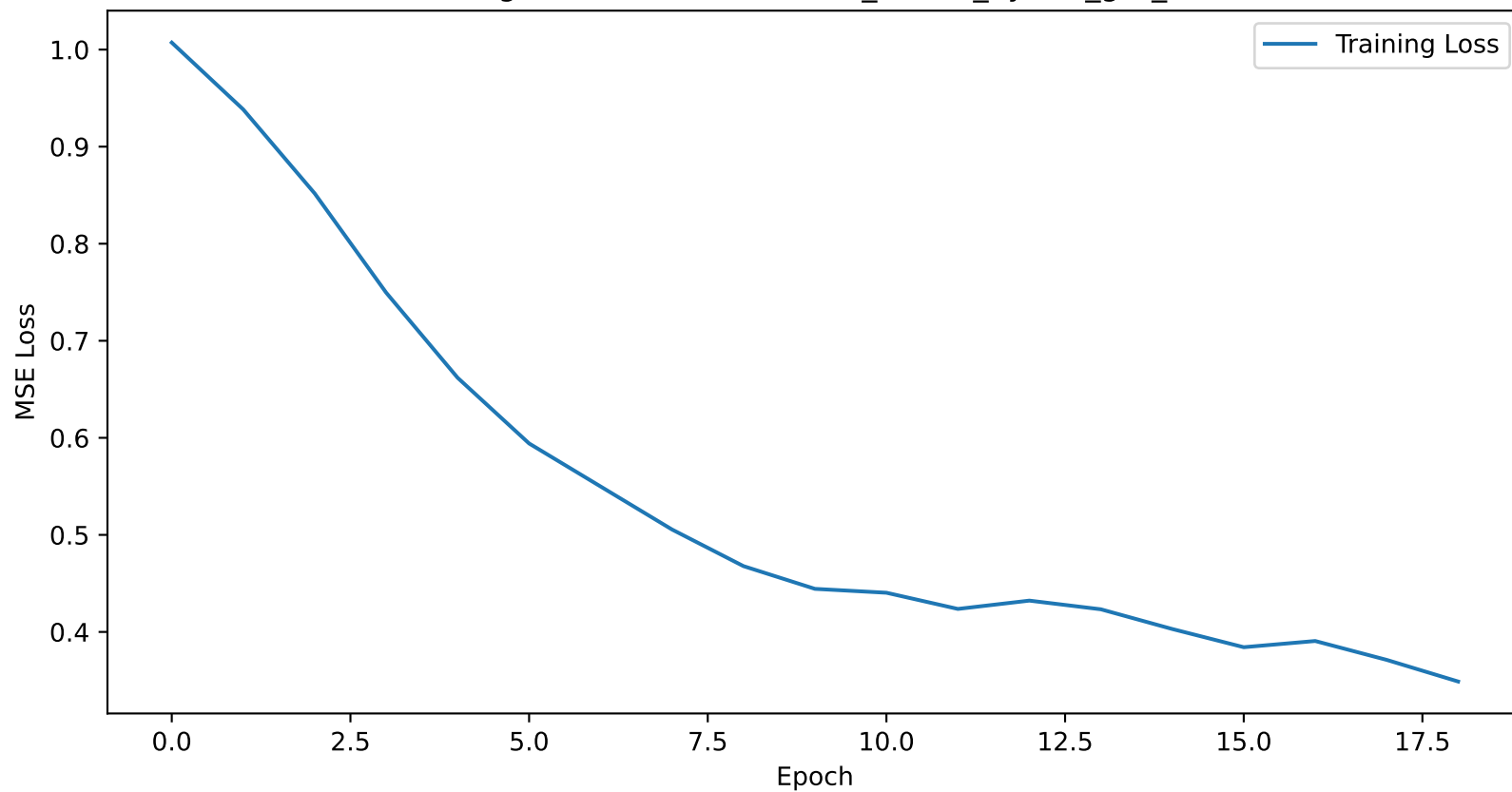
Training Loss Curve for atlanta_45min_hybrid_gru_lstm
