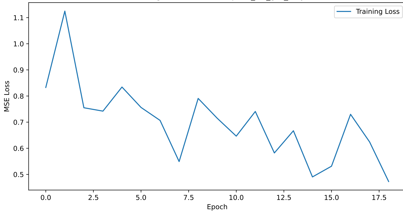
Training Loss Curve for elpaso_6H_gru_only
