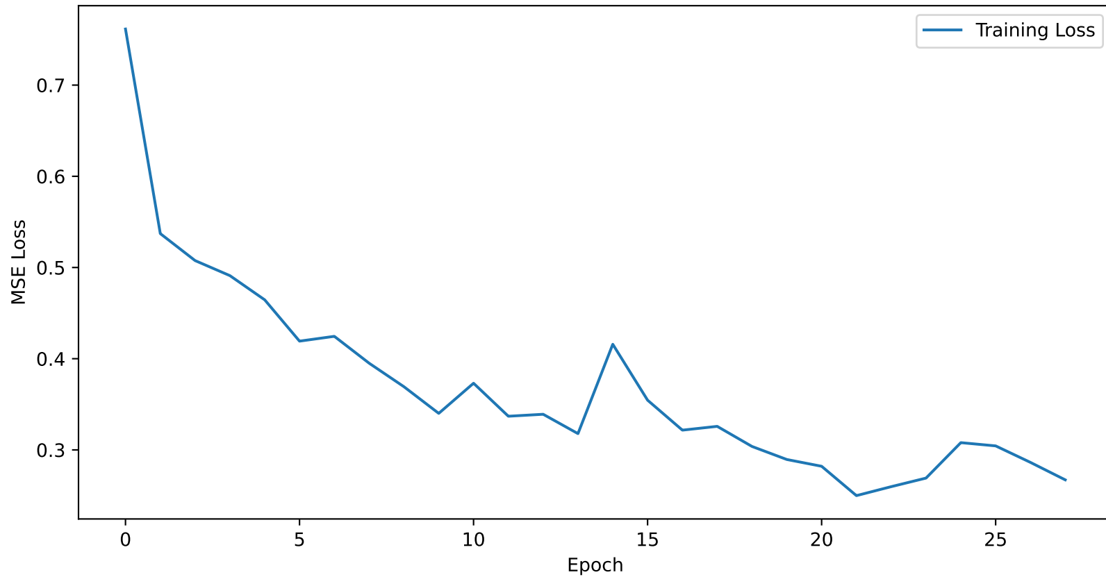
Training Loss Curve for dallas_15min_lstm_only
