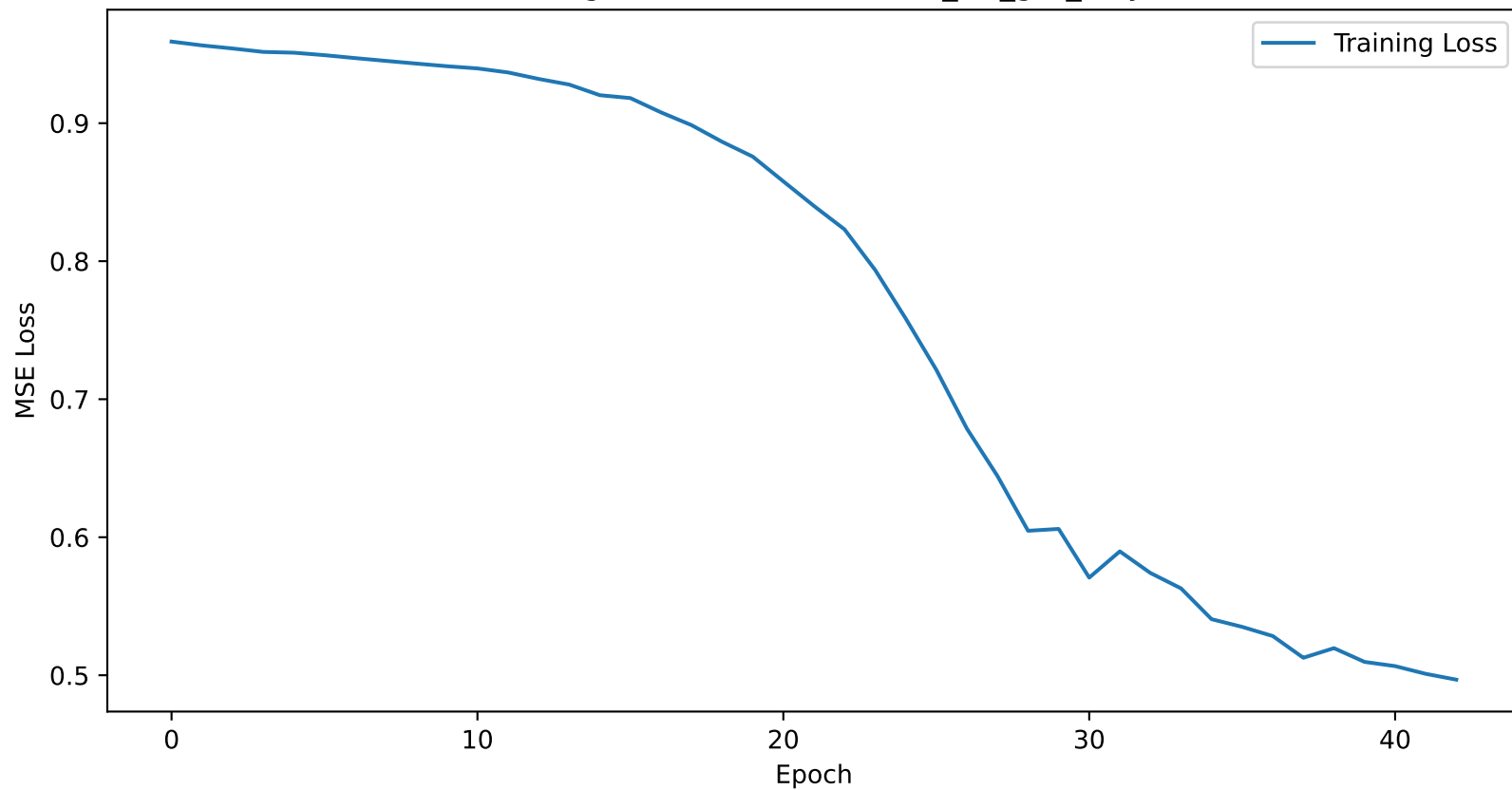
Training Loss Curve for boston_6H_gru_only
