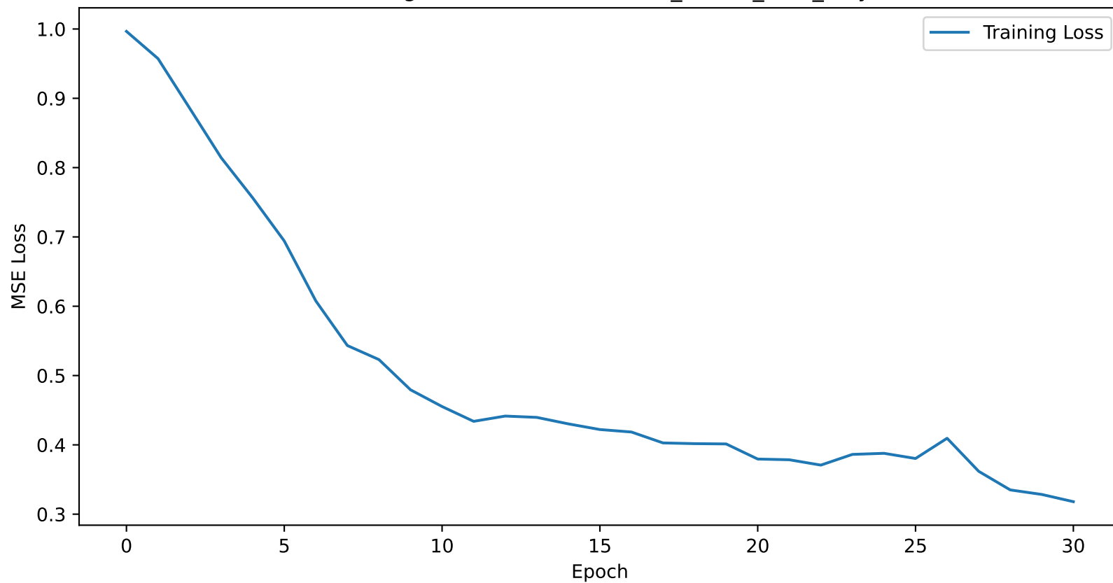
Training Loss Curve for atlanta_45min_lstm_only
