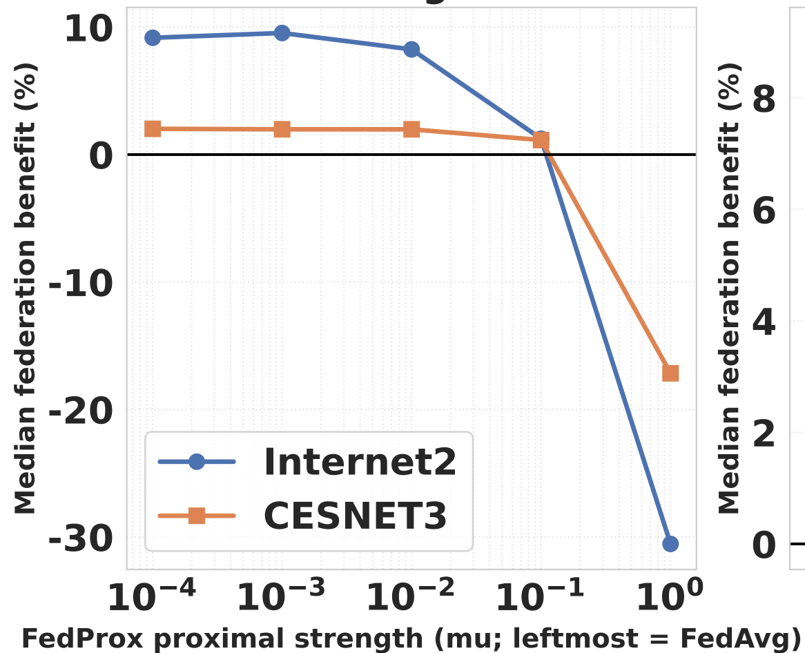
A: Constraining Local Drift
