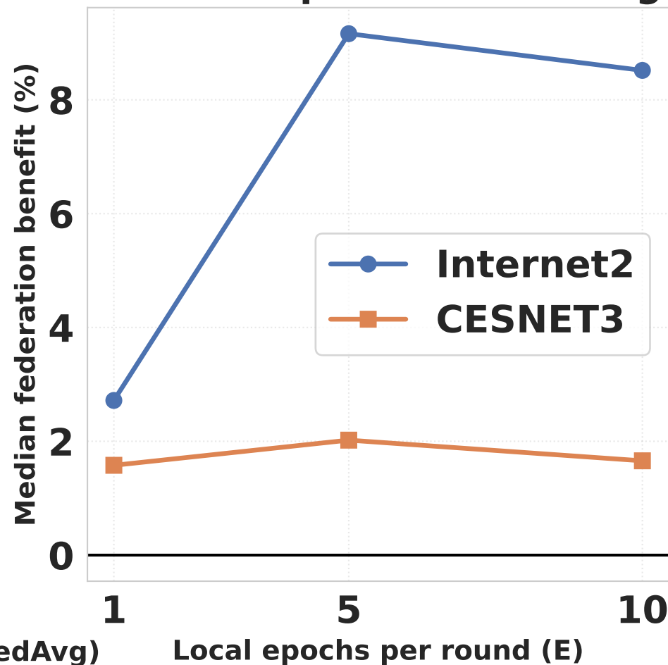
B: Local Optimization Budget
