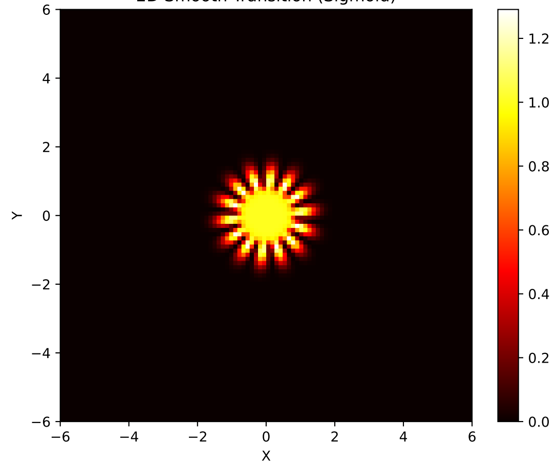
2D Smooth Transition (Sigmoid)
