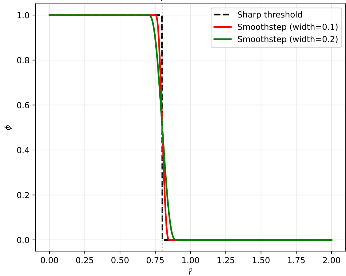
2D Smooth Transition (Sigmoid)
