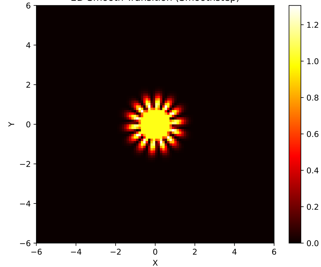
2D Smooth Transition (Smoothstep)
