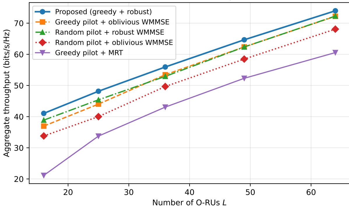
Aggregate throughput vs. L ( \tau_p = 8 , K = 16 )
