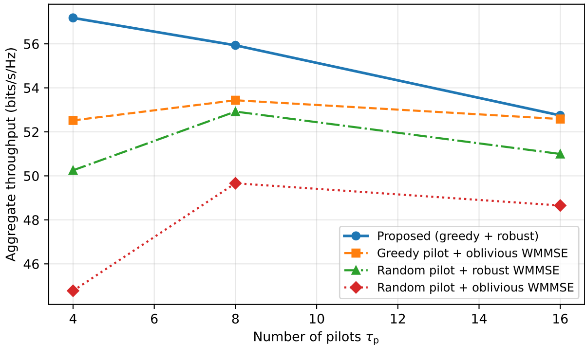
Ablation study ( K = 16, L = 36 )
