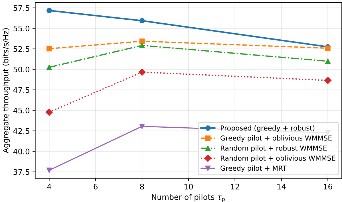
Aggregate throughput vs. \tau_p ( K = 16, L = 36 )
