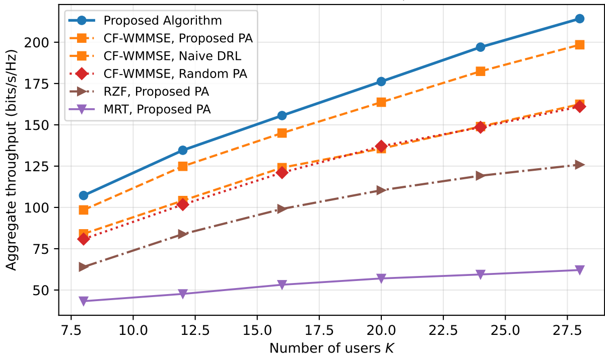
Aggregate throughput vs. K ( \tau_p = 8 , L = 49 )
