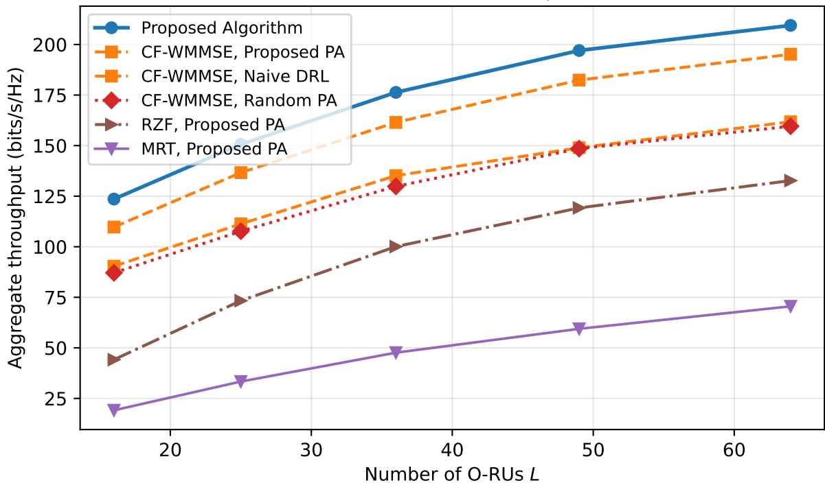
Aggregate throughput vs. L ( \tau_p = 8 , K = 24 )
