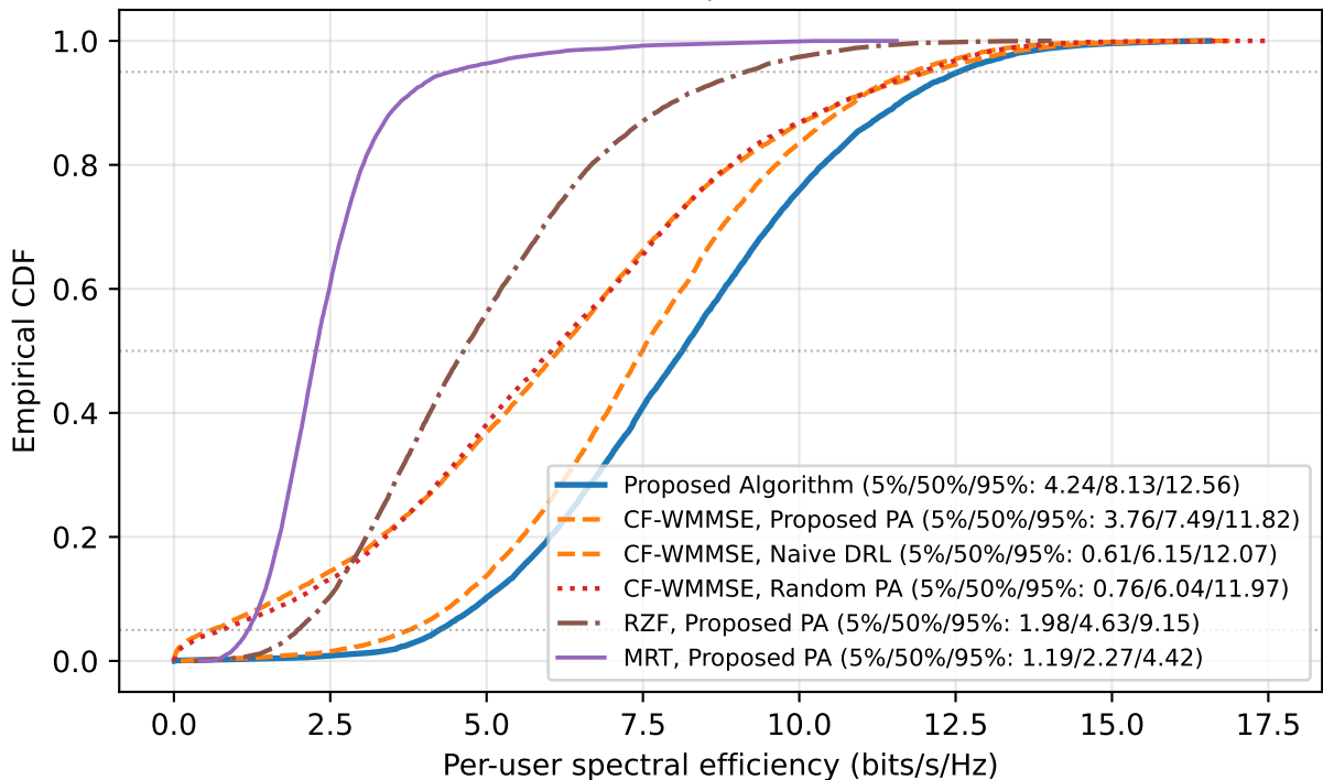
Per-user SE CDF ( \tau_p = 8 , K = 24 , L = 49 )
