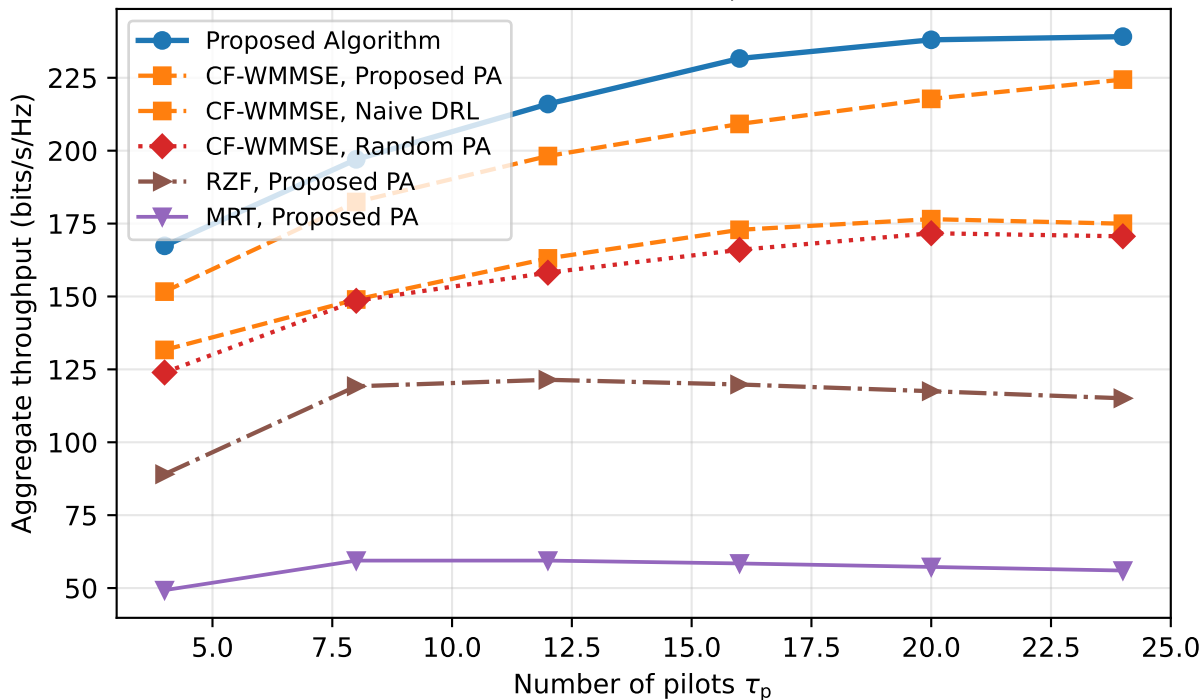
Aggregate throughput vs. \tau_p ( K = 24, L = 49 )
