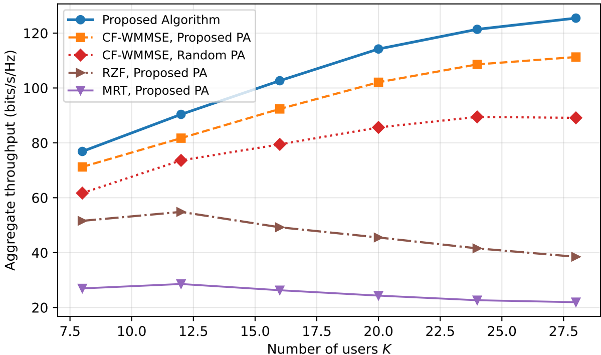
Aggregate throughput vs. K ( \tau_p = 4 , L = 25 )
