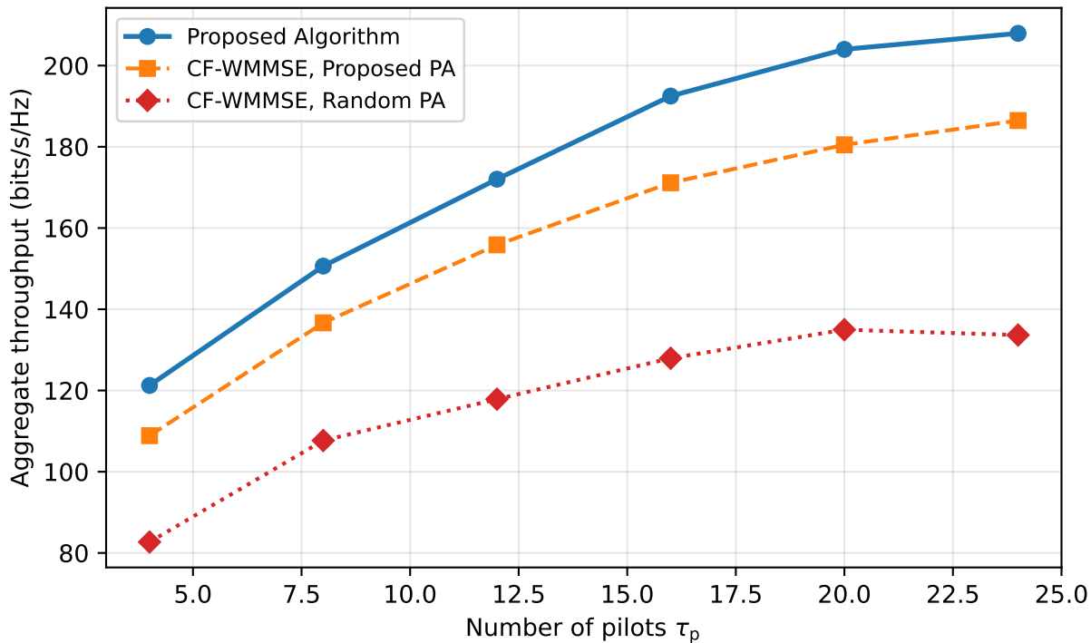
Ablation study ( K = 24, L = 25 )
