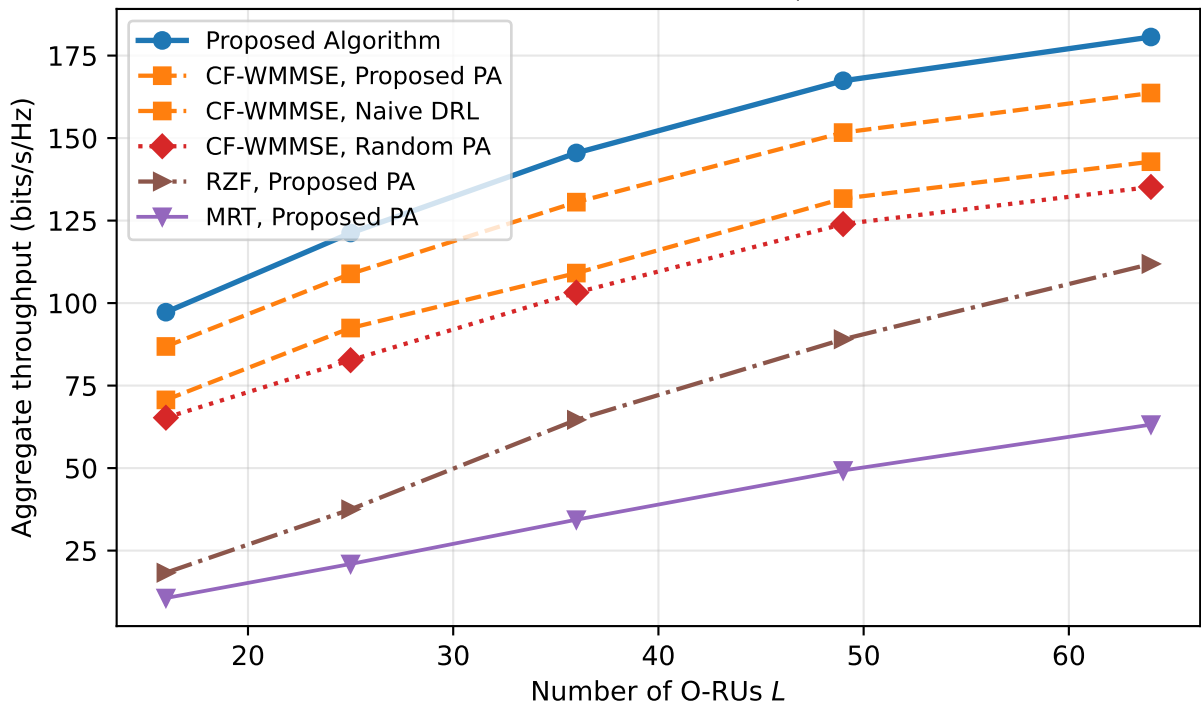
Aggregate throughput vs. L ( \tau_p = 4 , K = 24 )
