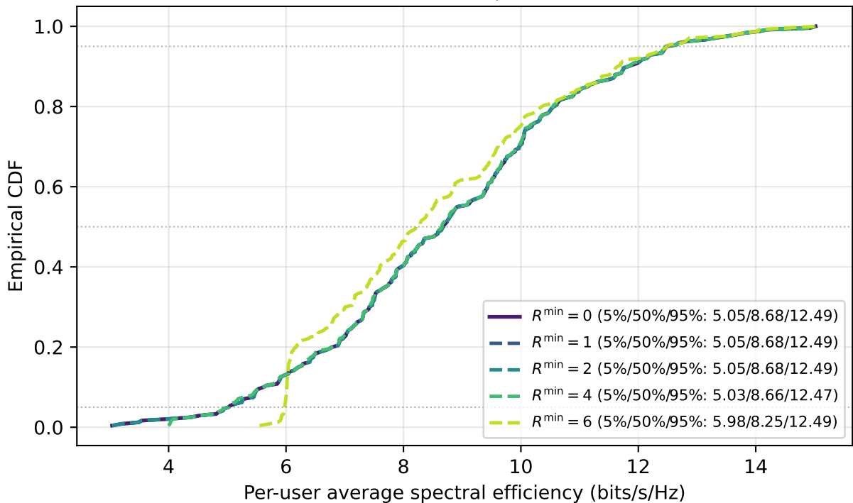
Proposed min-rate CDF ( \tau_p = 8 , K = 24 , L = 64 )
