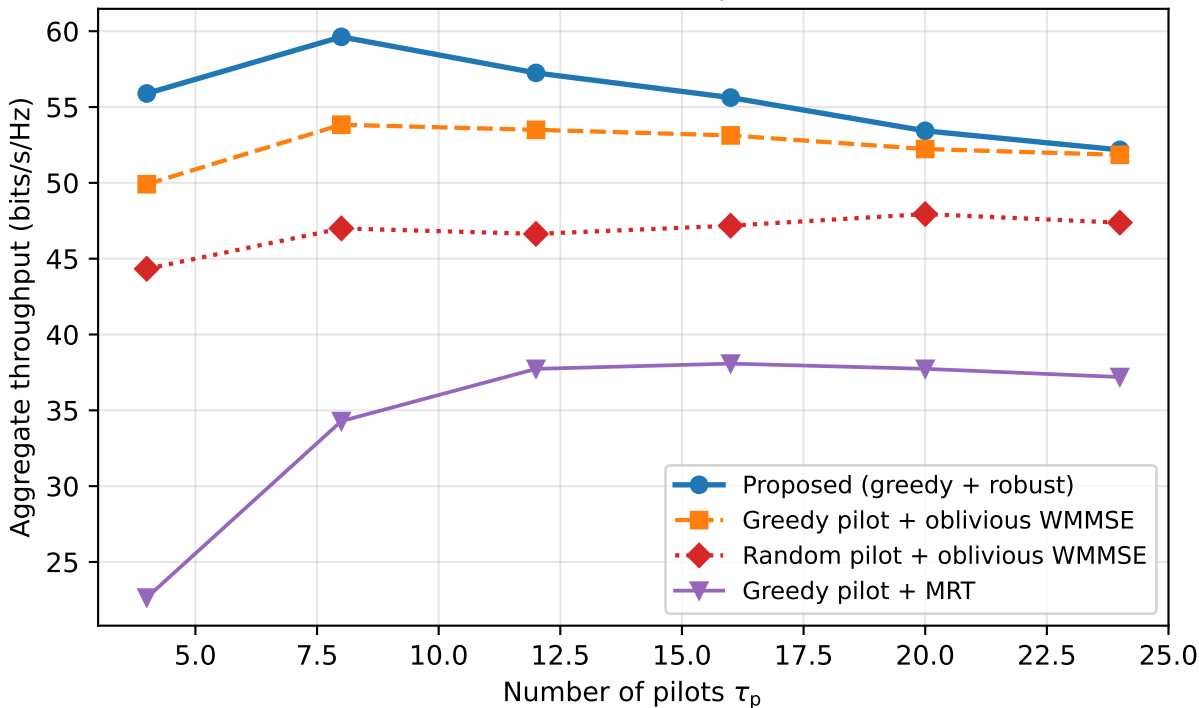
Aggregate throughput vs. \tau_p ( K = 24 , L = 25 )
