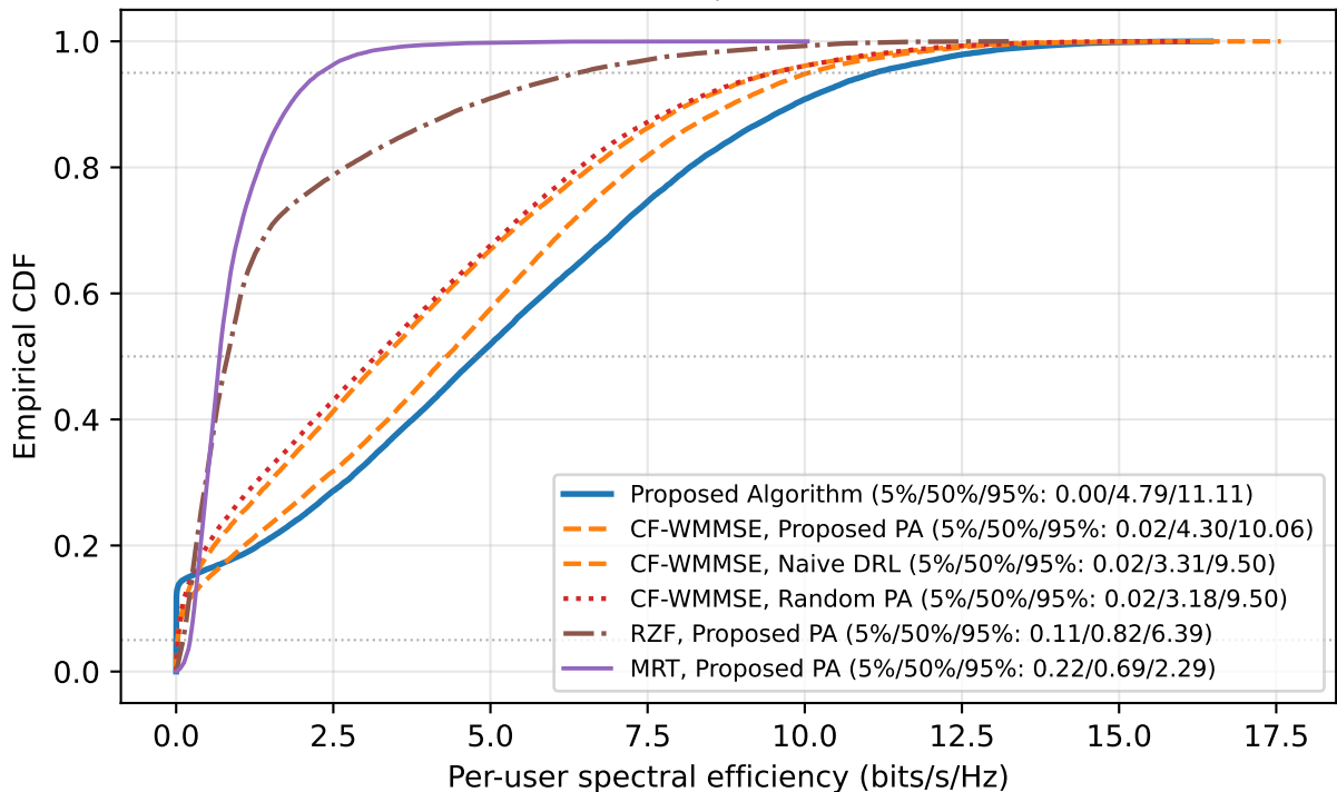
Per-user SE CDF ( \tau_p = 4 , K = 24 , L = 25 )
