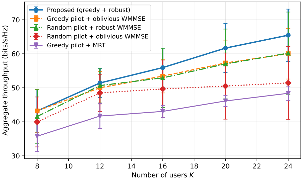
Aggregate throughput vs. number of users
