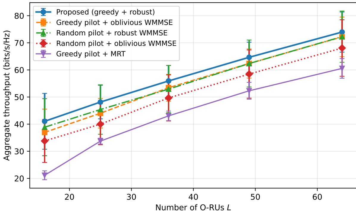
Aggregate throughput vs. number of O-RUs
