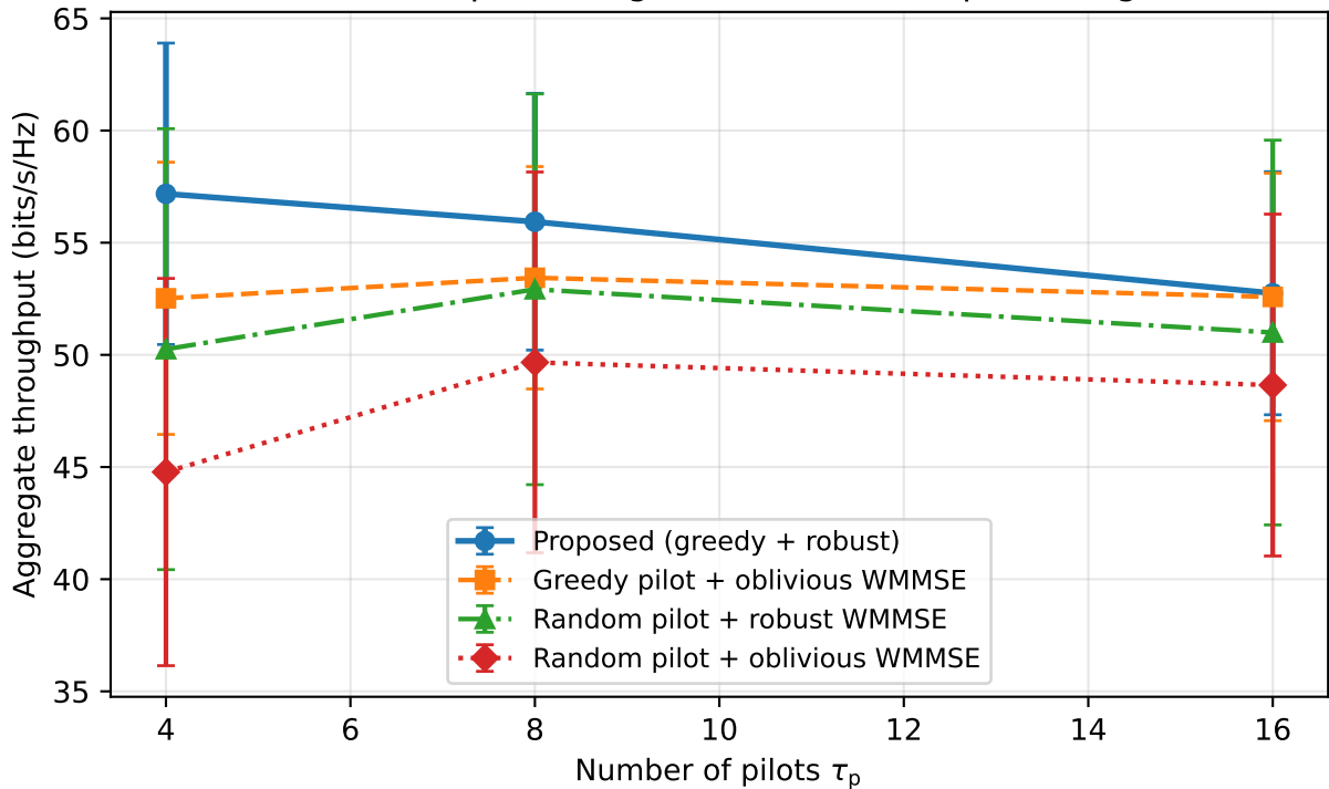
Ablation: pilot assignment vs. robust precoding
