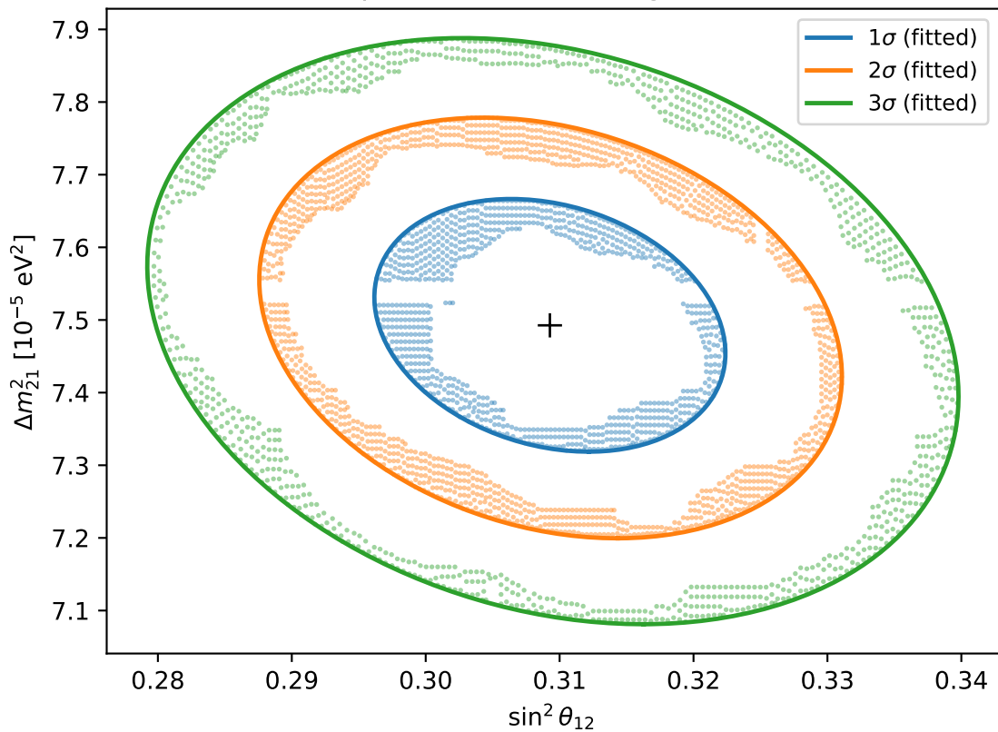
Outer ellipses fitted to the digitized contours
