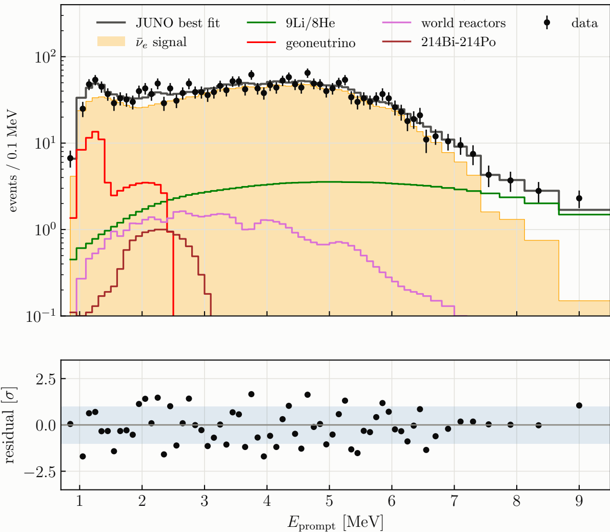
JUNO 2025, 59.1 days (2379 candidates)
