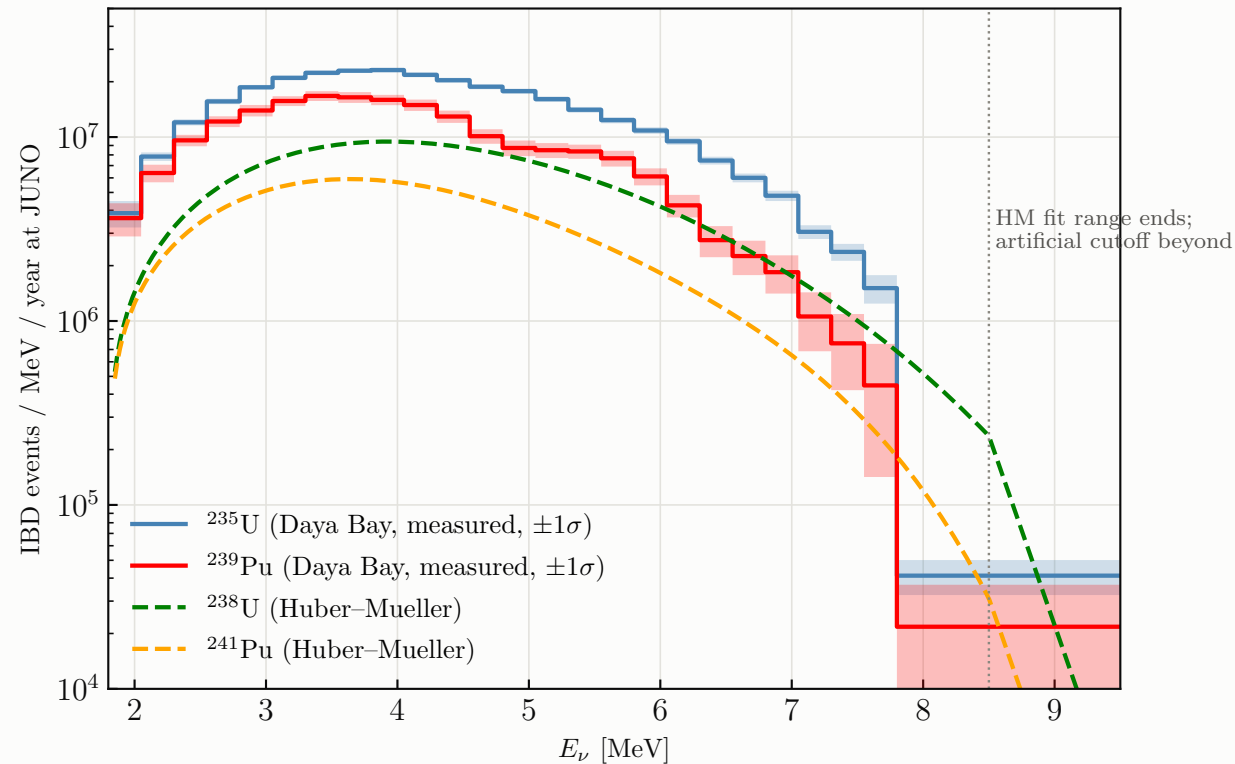
Per-isotope IBD rate at JUNO for a pure 10 MW core at 50 m
