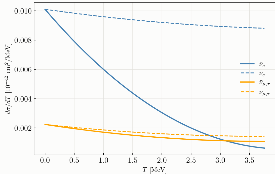
Recoil spectra at E_\nu = 4 MeV
