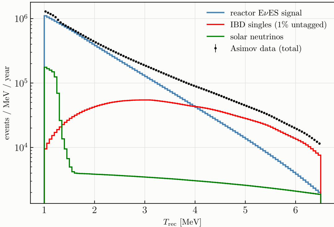
E\nu ES at JUNO from 10 MW at 50 m, one year at 90% duty
