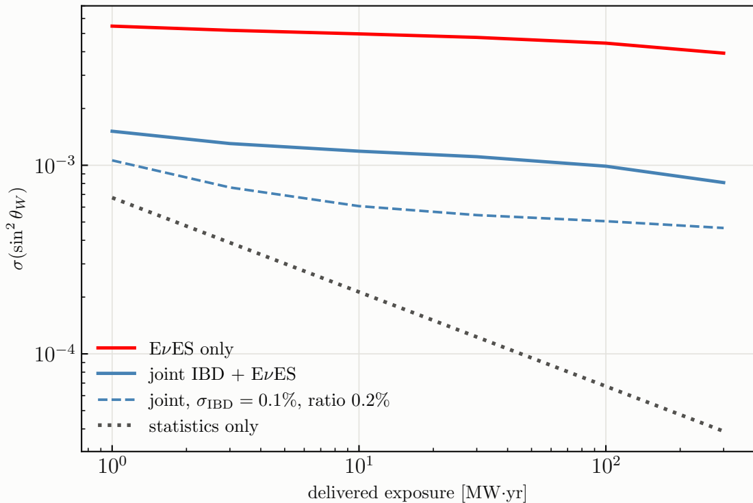
Weak mixing angle from E\nu ES, 10 MW at 50 m
