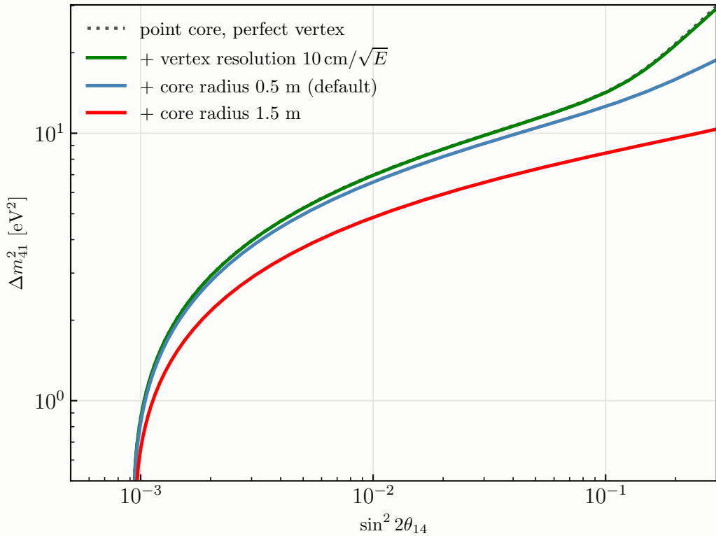
The high- \Delta m^2 wall, D = 50 m
