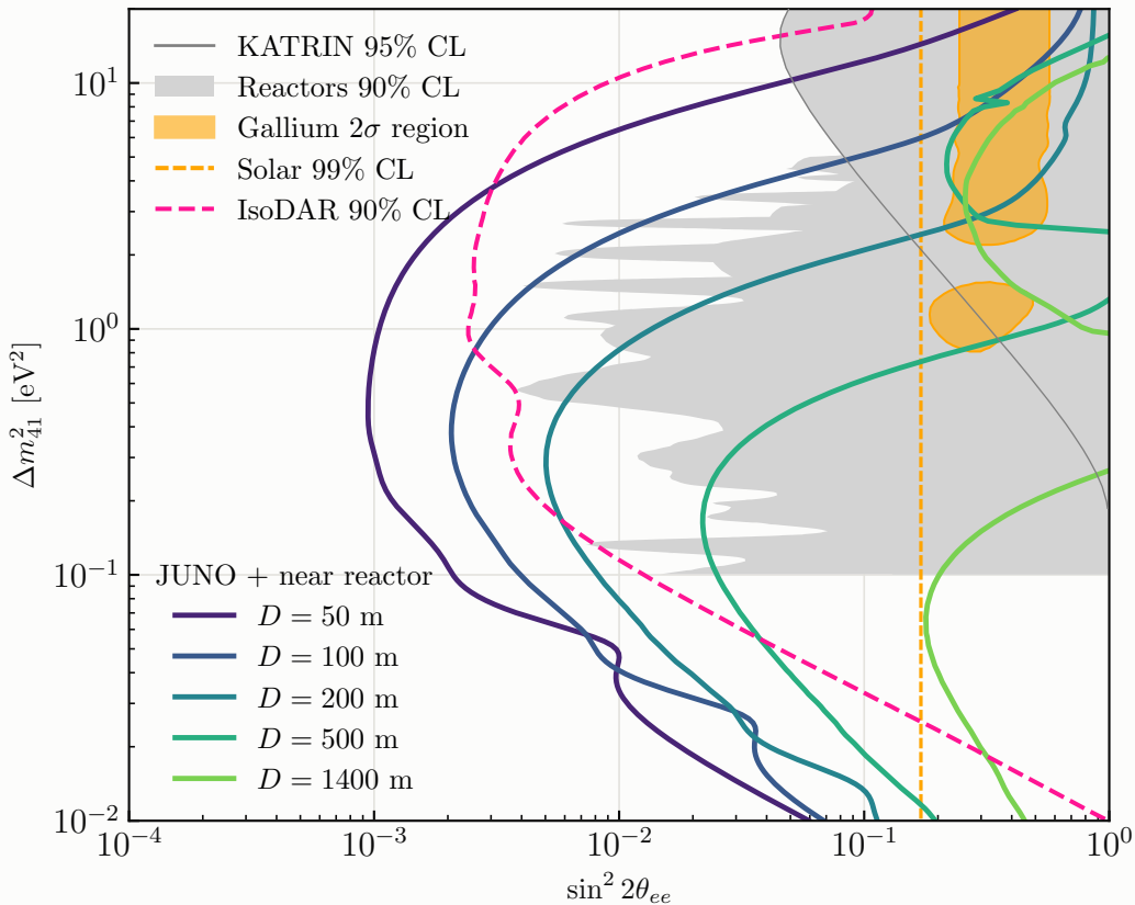
95% CL sensitivity, 27 MW·yr
