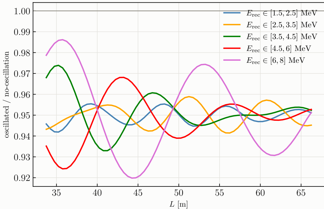
The wiggle across the detector, D = 50 m
