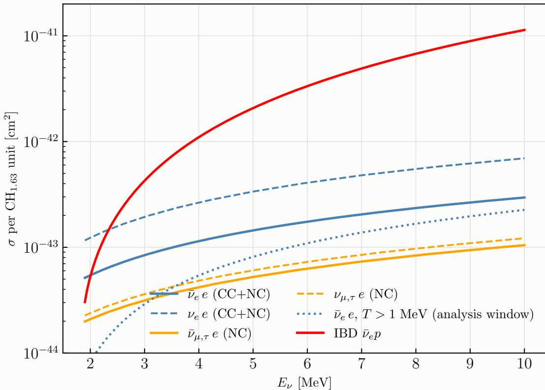
Cross sections per carbon of LAB ( \text{CH}_{1.63} )
