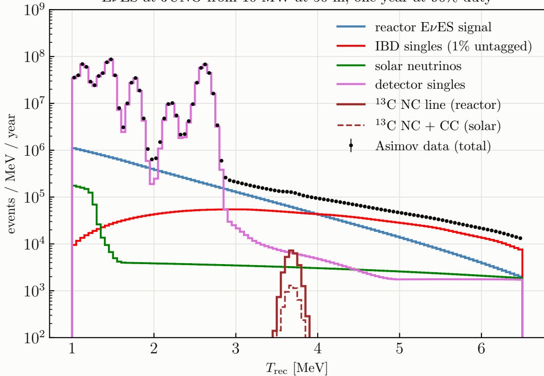
\text{E}\nu\text{ES} at JUNO from 10 MW at 50 m, one year at 90% duty
