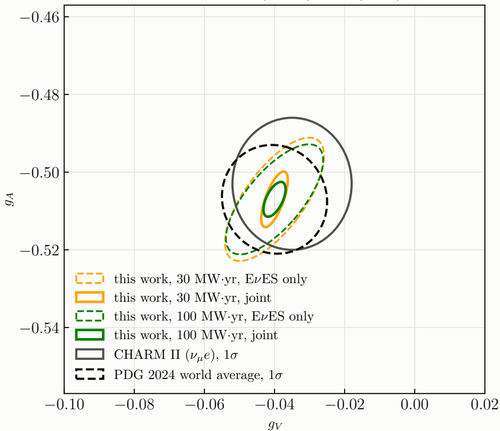
1\sigma regions in the (g_V, g_A) plane (zoom)
