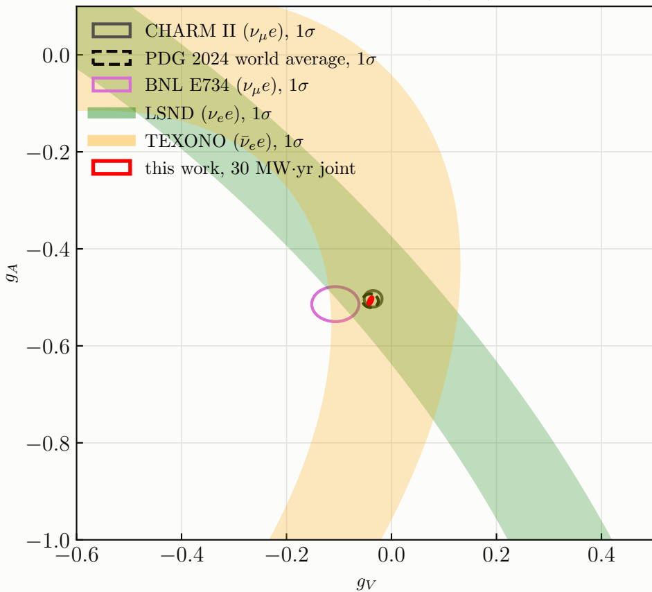
Existing constraints in the (g_V, g_A) plane
