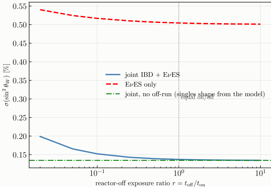
What the reactor-off run buys, 30 MW·yr
