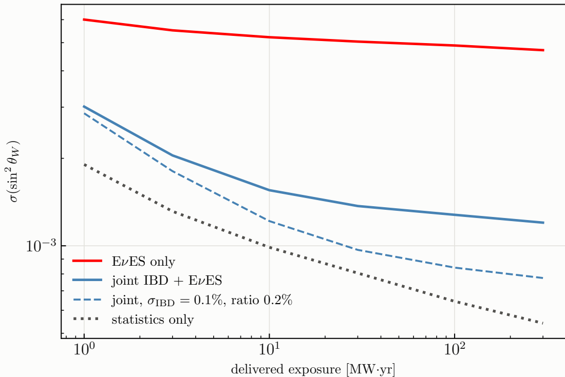
Weak mixing angle from \text{E}\nu\text{ES} , 10 MW at 50 m
