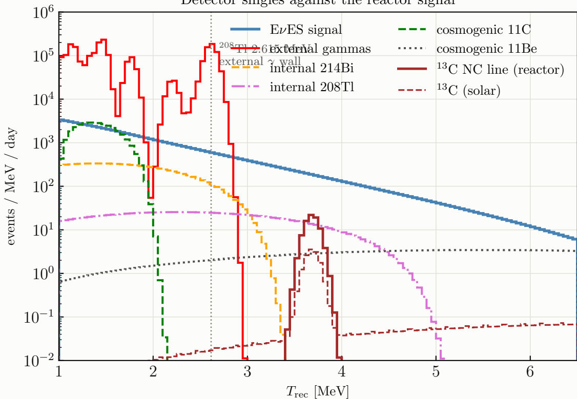
Detector singles against the reactor signal
