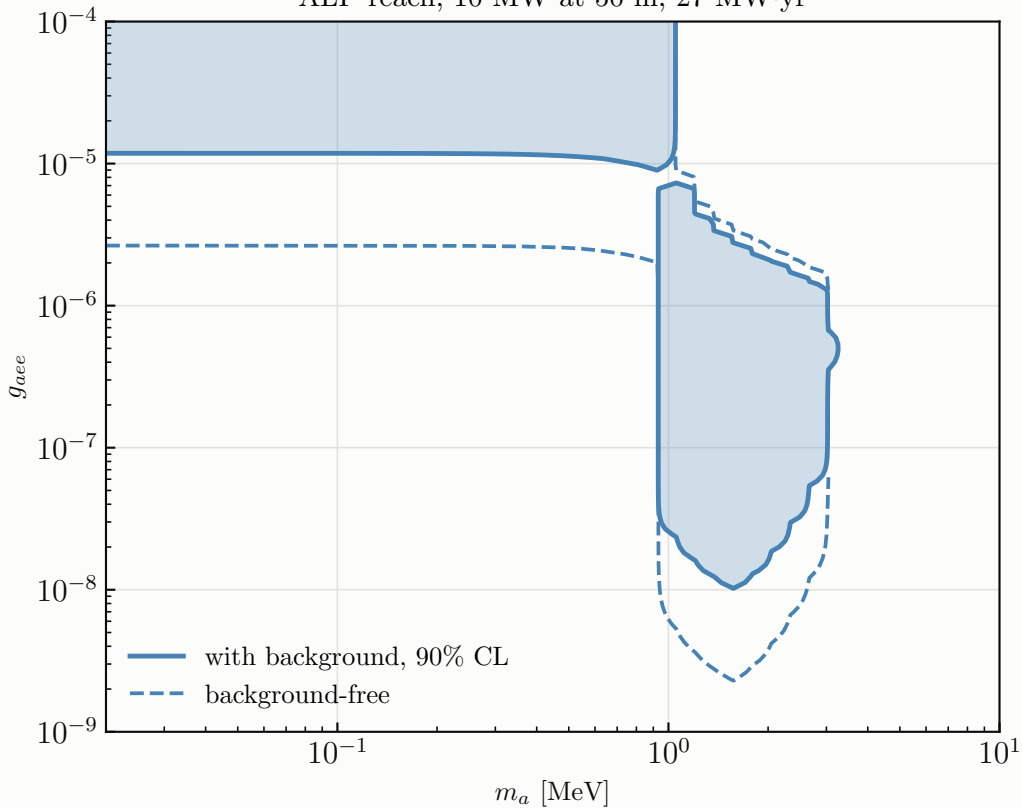
ALP reach, 10 MW at 50 m, 27 MW·yr
