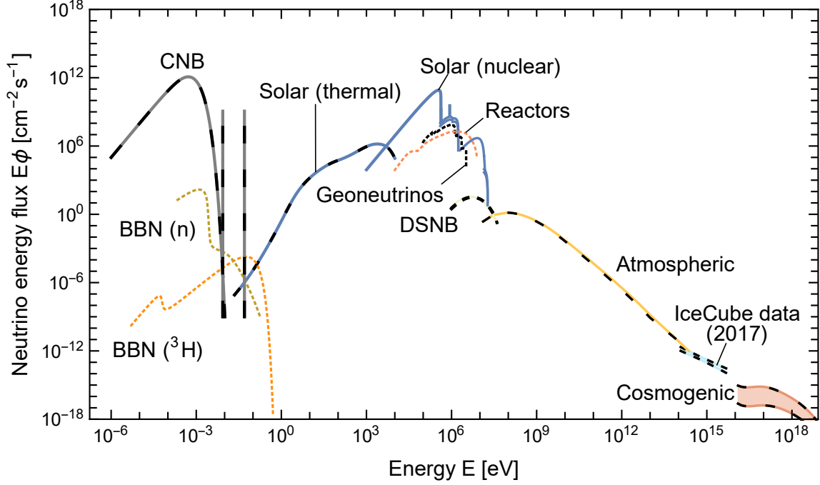
Figure 1: Energy flux of neutrinos from different sources as a function of neutrino energy in logarithmic scale (a more accurate label for the x -axis would be \log(E_\nu/\text{eV}) , with tick labels at -6, -3, 0, 3, \dots, 18 ). The CνB dominates the energy flux at very low energies, while solar neutrinos (nuclear) dominate at higher energies. The spikes appear because this figure accounts for the three different masses of the neutrino mass eigenstates. The two spikes in black-grey dashed indicate that the energy of two of the massive neutrinos are dominated by their mass and that the lightest state is taken to be massless (hence the broad distribution of energies that is allowed to go to zero). Figure from [? ].
