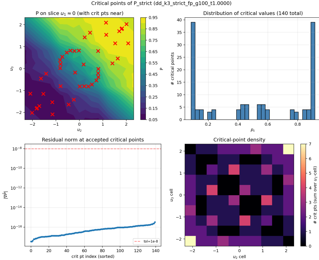
Figure 28: Critical points of P_{\text{strict}} at \gamma=100, \tau=1 : 140 points, 42 unique p_c values, distribution bimodal with mass concentrated near the p \rightarrow 0, 1 tails.
