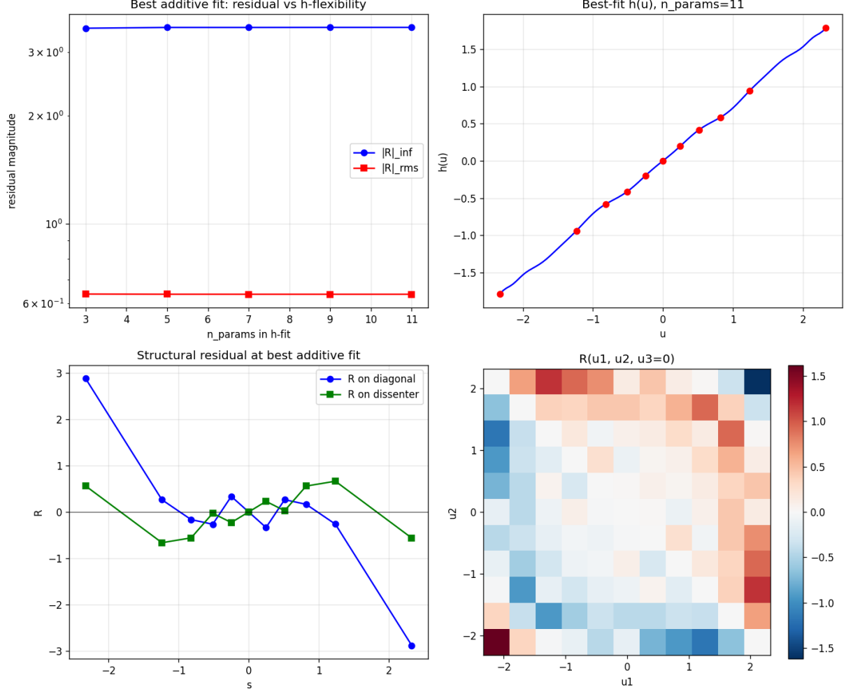
Figure 27: (Top left) Residual magnitude vs Cheby flexibility in \hat{h} : flat across n = 3 \dots 11 . (Top right) Fitted \hat{h}(u) : approximately linear. (Bottom left) Residual on diagonal R(s, s, s) and dissenter R(s, s, -s) : both antisymmetric, dominated by corners. (Bottom right) Heatmap R(u_1, u_2, u_3 = 0) : high-rank checkerboard, not a smooth polynomial.
