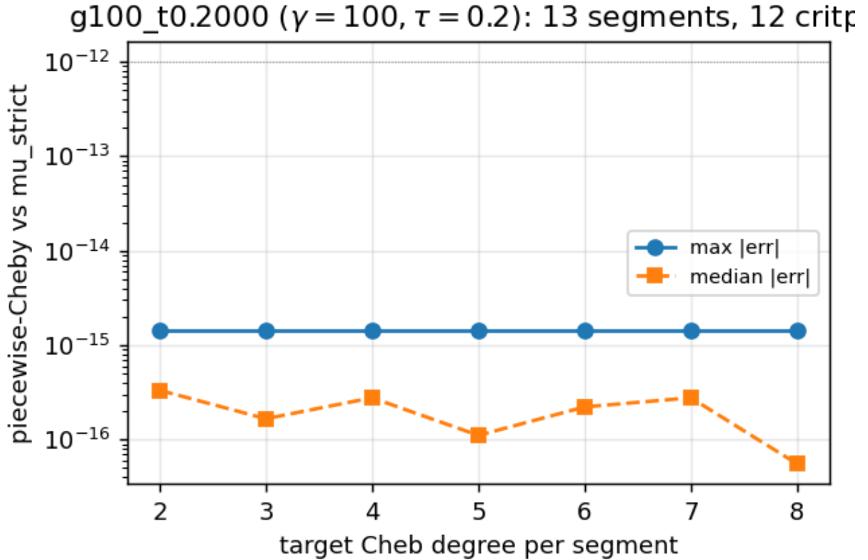
Figure 30: Per-segment Cheby convergence at (\gamma, \tau) = (100, 0.2) : machine \varepsilon at any degree, max error \sim 10^{-15} .
