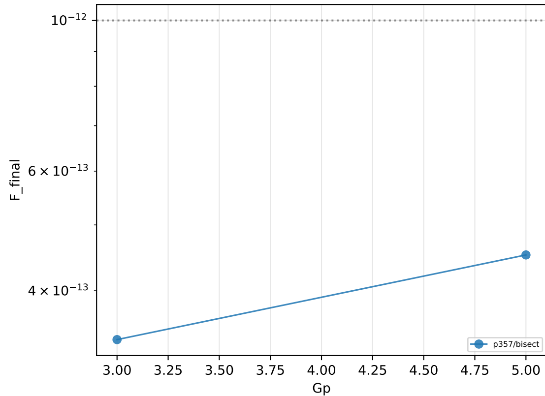
Newton residual F
