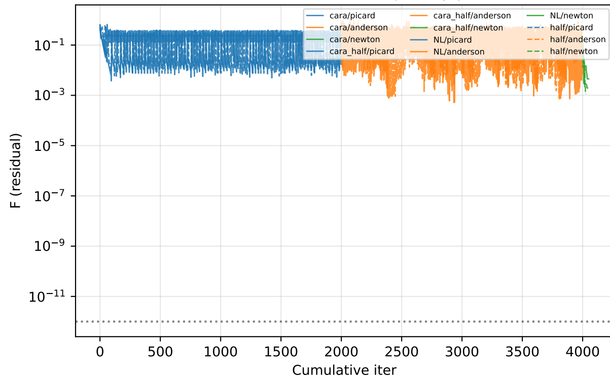
Cold start \tau=0.5 : solver trajectory per init
