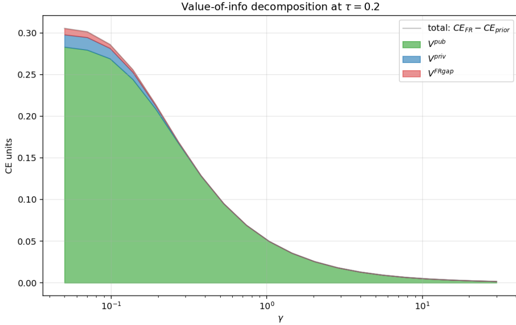
Figure 4: Value-of-information decomposition at \tau = 0.20 . The price delivers the majority of the welfare value; the own private signal contributes a strictly positive but smaller share; the welfare gap to full revelation is tiny at high \gamma but \Theta(V_i^{\text{pub}}) at low \gamma .
