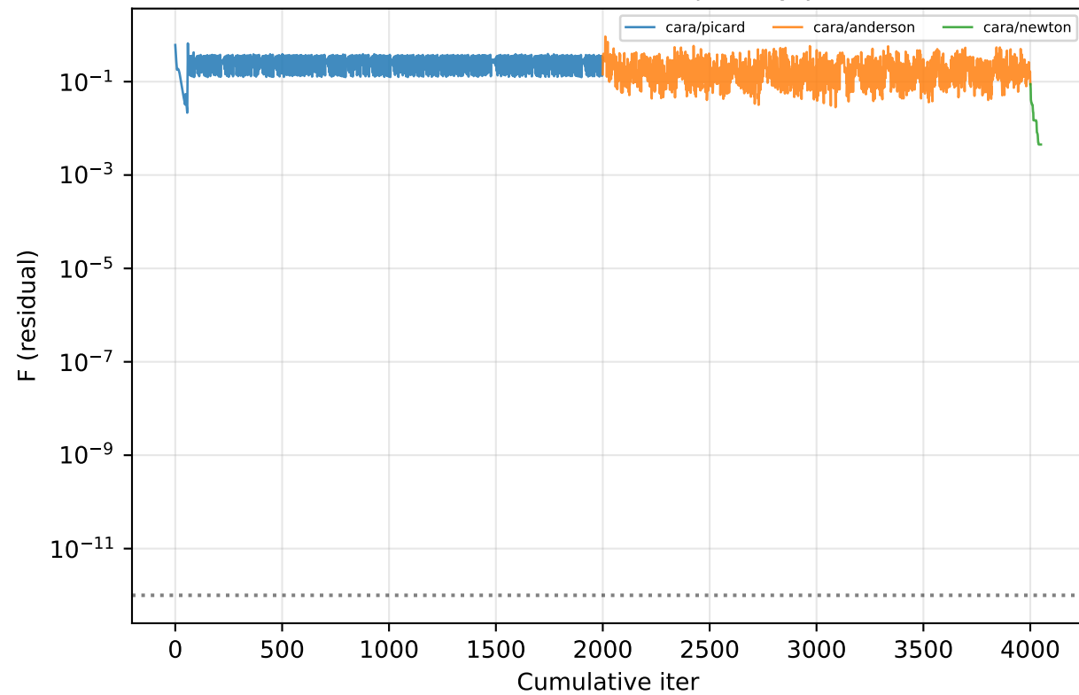
Cold start \tau=0.5 : solver trajectory per init
