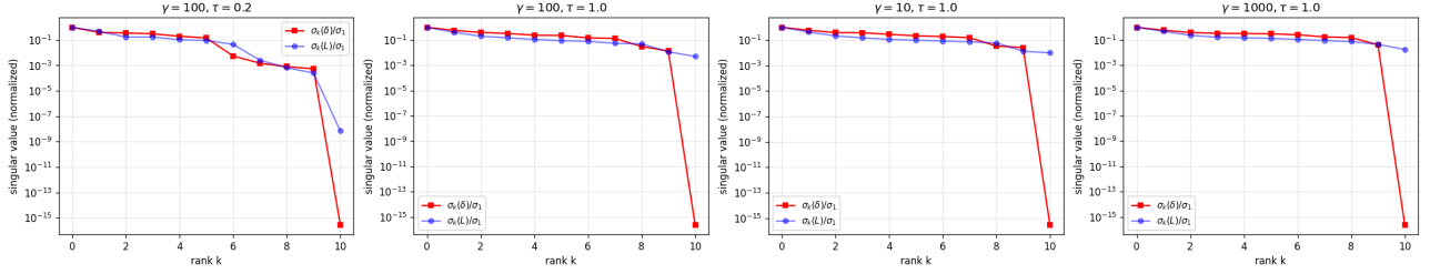
Figure 23: Singular value spectrum of \delta vs L . They track each other through k \approx 9 ; both are effectively full-rank ( G = 11 ). Rank-1 truncation captures only 30–45% of \delta ; rank-5 captures 65–80%. A low-rank multiplicative correction would not close the gap either.
