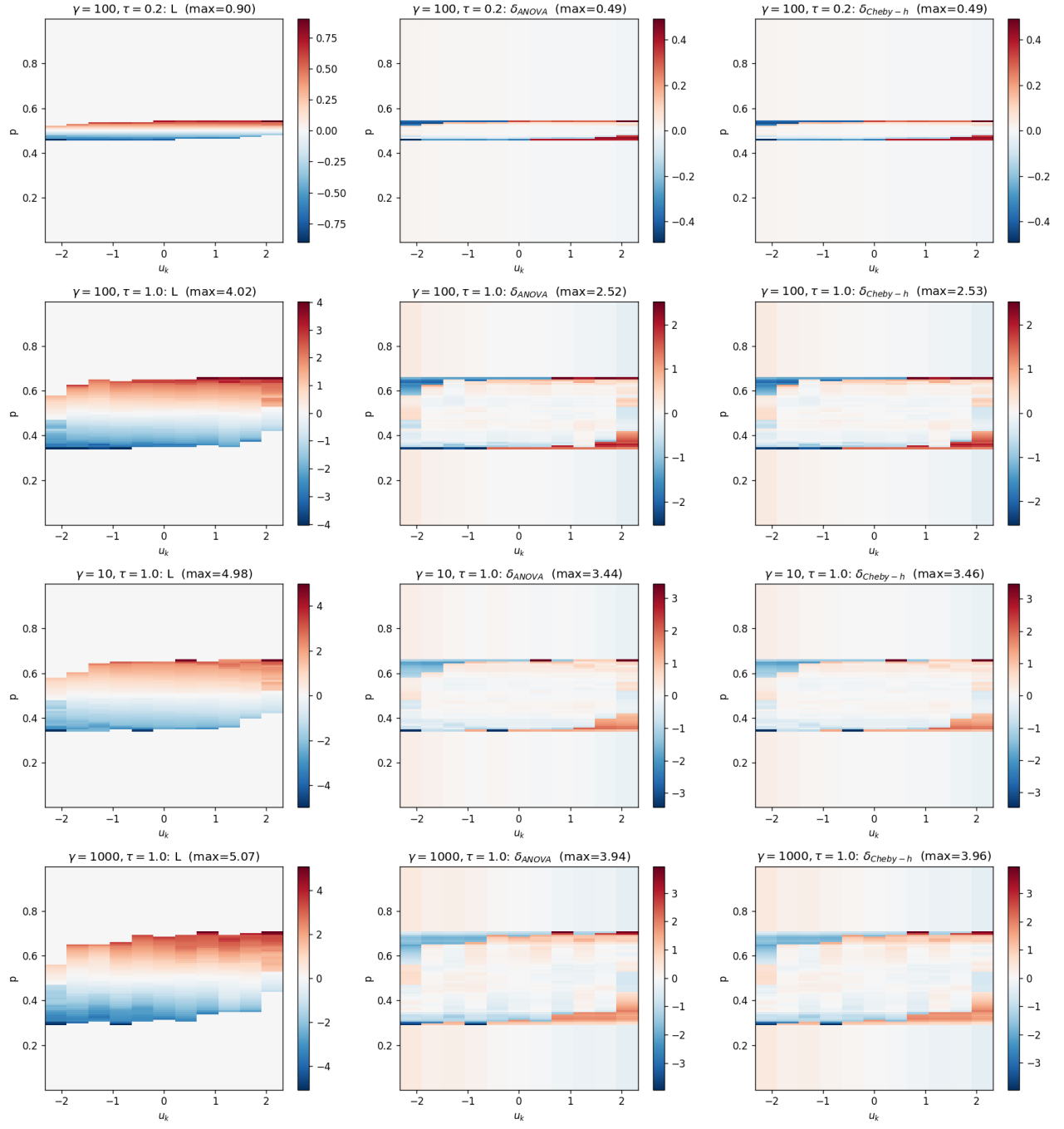
Figure 21: Heatmaps of L(p, u_k) (left), \delta_{ANOVA} (middle), \delta_{Cheby-h} (right). The smooth bulk gradient in L is removed in \delta , but the sharp horizontal bands at the critical-value p 's — the cusps — are preserved unchanged.
