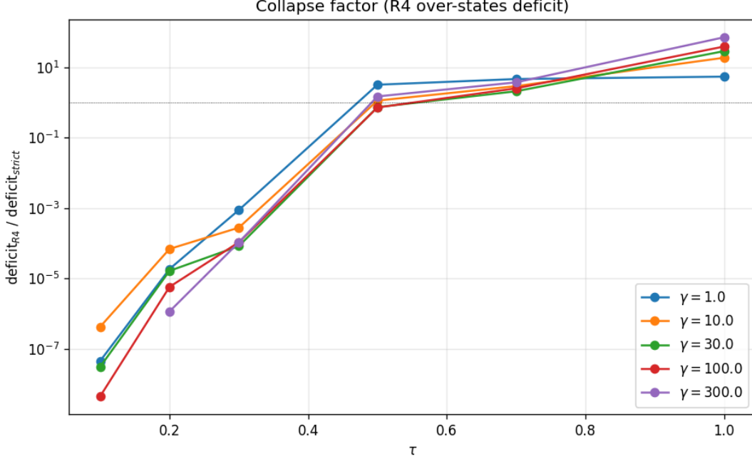
Figure 26: Collapse factor \text{def}_{R4}/\text{def}_{\text{strict}} per cell. Reaches \sim 30\times at \tau \in [0.7, 1] , consistent with the 40\times collapse seen in the original 8-cell strict spot-check. The sign-flip (ratio < 1 at low \tau ) suggests two distinct R4 failure modes: under-smoothing of smooth cells, over-smoothing of cuspy ones.
