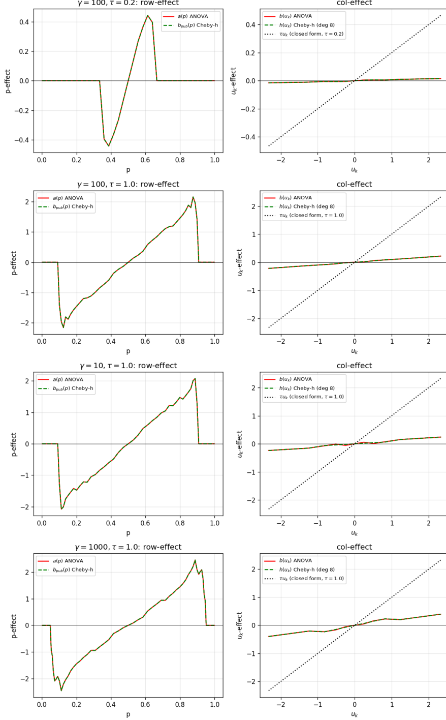
Figure 24: Left: row-effect a(p) . Right: column-effect b(u_k) . The dotted black line is the textbook prediction \tau u_k ; the fitted green line is \sim 10\times smaller in magnitude. At \tau = 1 the closed-form L_{\text{priv}} would range [-2.33, +2.33] but the empirical b(u_k) only ranges [-0.22, +0.22] .
