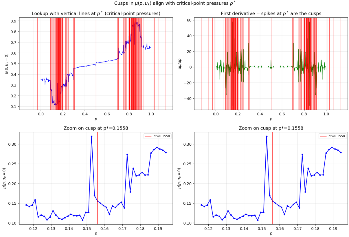
Figure 28: Resulting \mu(p, u_k) cusps: each spike in the horizontal-axis derivative corresponds to a critical-point crossing. PCHIP-based builders absorb these as kinks; polynomial builders ring around them.
