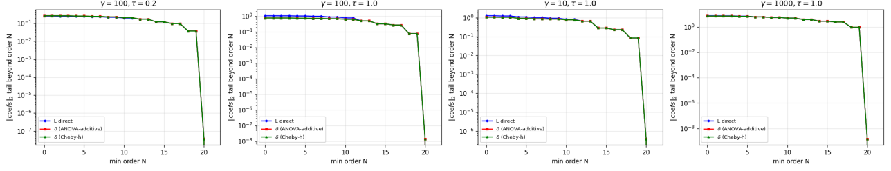
Figure 22: Cumulative Cheby coefficient tail norm: (\sum_{i+j \geq N} c_{ij}^2)^{1/2} vs N . The three curves overlap: direct fit of L , fit of \delta_{\text{ANOVA}} , fit of \delta_{\text{Cheby-h}} all decay at the same algebraic rate. The coordinate transformation does not improve the per-coefficient convergence rate.
