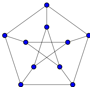
Figure 1: The Petersen Graph P
