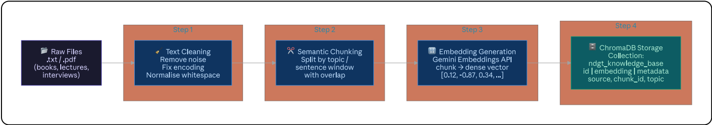
Diagram 2 — Document Ingestion Pipeline
